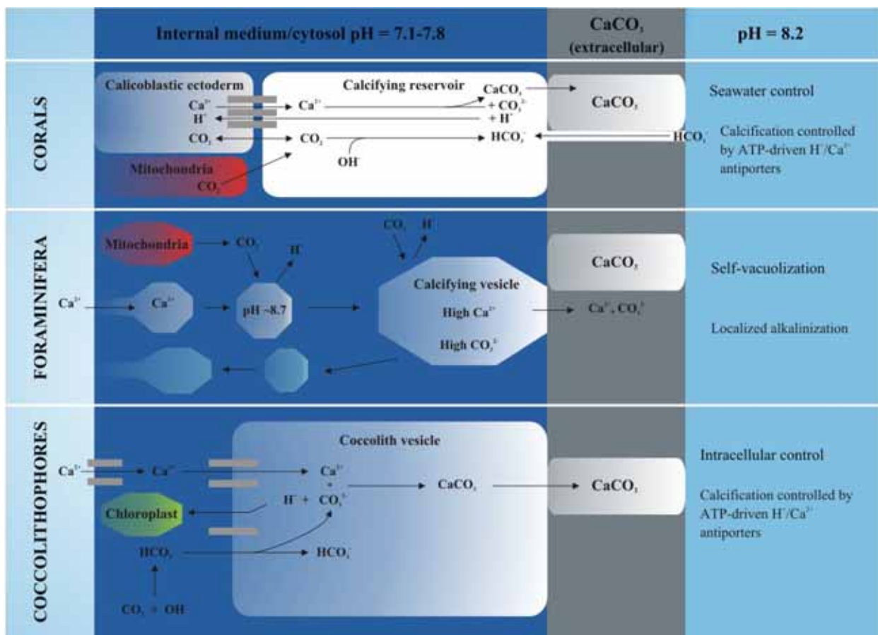
Fig. 9.2. Models describing possible calcification mechanisms in organisms that calcify extracellularly (corals, foraminifera) and intracellularly (coccolithophores). Most calcifying organisms maintain a region of calcification that is isolated from ambient seawater. The rate of calcification is likely dependent upon the organisms' ability to maintain an elevated CaCO 3 saturation state ( [Ca^{2+}] , [CO_3^{2-}] ) by exchanging Ca 2+ and H + ions via a network of Ca 2+ -ATPases and ion pumps (Allemand et al. 2004; Taylor et al. 2011). The pH of the calcifying fluid of tropical scleractinian corals (De Beer et al. 2000; Bown 2005) and some benthic foraminifera (Bentov et al. 2009) is thought to be 9.0-9.5 and ~8.7, respectively. In contrast, the pH of the organisms' cytosolic fluid is thought to be 7.2-7.5 (Venn et al. 2009).
