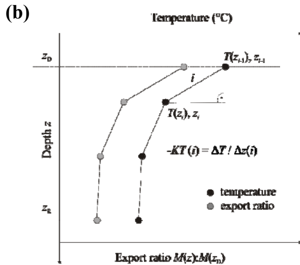
Fig. 4.1. (a) Parameterization of the decay rate [ k_{(T)} ] of jelly-POM and temperature. Also, k data of phytodetritus (Sudo et al. 1978; Fujii et al. 2002)]. (b) Piecewise linear calculation of the export ratio. The depth range between z_D and z_R is divided into intervals bounded by z_{i-1} and z_i , within which a linear thermal gradient K_T(i) is assumed.
