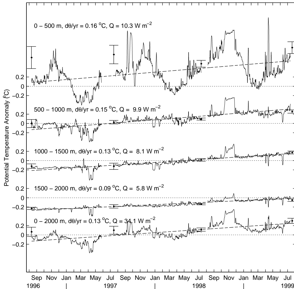
FIG. 4.6: Potential temperature anomaly ( 3 \text{ }^\circ\text{C} subtracted) averaged over 500 m layers at the Labrador Sea convection moorings K1 (1996/97), K11 (1997/98), and K21 (1998/99). A linear trend fitted to the temperature time series is shown as a dashed line. Each curve is labeled with the warming rate and the equivalent heat flux (for that particular layer) resulting from the fit. Mean and standard deviations from CTD profiles are shown as dots and errorbars.
