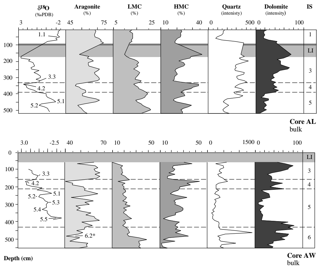
Figure C.7-3: Mineralogical logs of the sediment cores at Abington Reef. In this cores only the mineralogy of the bulk sediments was determined by X-ray diffraction analysis. Core AW reaches down to IS 6, the penultimate glacial, where LMC-percentages are significantly increased. Numbers on the isotope curve are SPECMAP events, 6.2* on the aragonite curve corresponds to the same isotopic event (aragonite stratigraphy). IS = isotope stages, LI = lithified interval.
