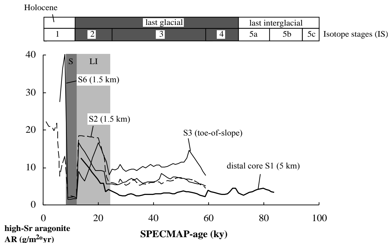
Figure D.3-10: Accumulation rates of high-Sr-aragonite in the periplatform sediments at Sanganeb Atoll. AR decrease with distance from the reef, which points to reduced shallow-water sediment input in the distal core S1. Increased dissolution of aragonite or carbonate in the distal core S1 is unlikely because all cores were taken in approximately same waterdepth. S = sapropel, LI = lithified interval.
