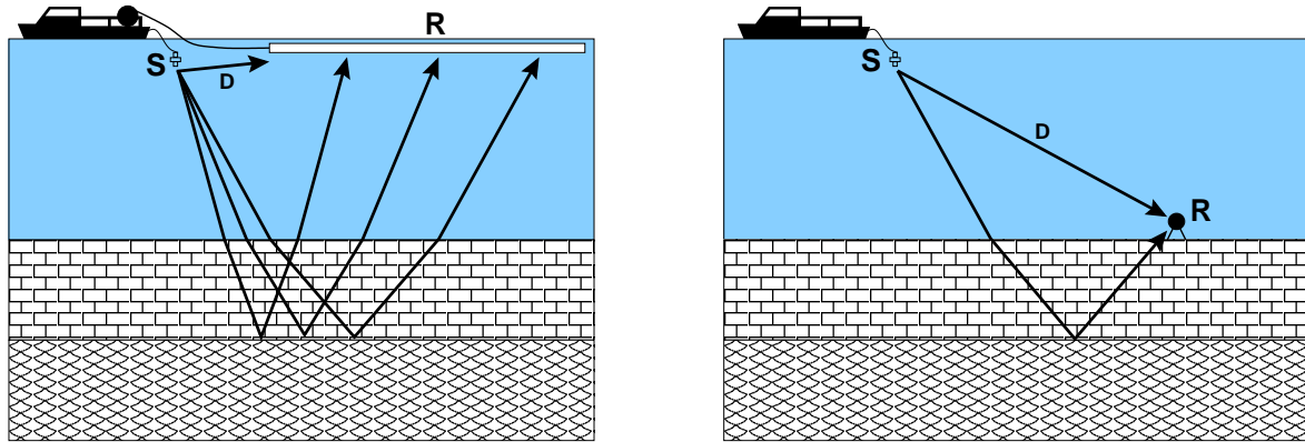
Figure 4.1: Seismic data were acquired using streamer- and ocean-bottom-hydrophone techniques. Airgun (S) and streamer (R) acquisition geometry in multichannel reflection seismic profiling reveal common shot gathers, where the direct water wave (D) is well-separated from the primary arrivals (left). In airgun-OBH acquisition geometry, the direct water wave often masks shallow primary reflections in the common receiver gather (right).
