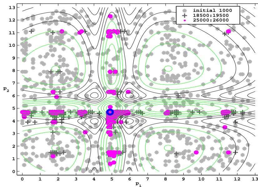
Figure A.4: Two dimensional cross-section of the parameter estimates during the search course with a normal GA. The markers refer to a certain range of iterations, see legend.
