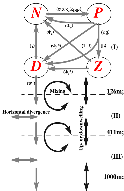
Figure 3.11: Annual net fluxes of nitrogen as they are evaluated at all three locations. The upper 1000 meters are resolved into three depth ranges (I-III). Horizontal arrows represent advective fluxes according to horizontal divergence in order to conserve water volume, see model description in main text. Vertical arrows show advective fluxes unless in the model vertical velocities are neglected (as in NPZD-nW). Open circles refer to turbulent and convective fluxes. Upward as well as incoming horizontal fluxes are indicated with positive signs. Diapycnal mixing at 1000 meters is not shown since it has no effect on the biology within the upper 400 meters. The internal biological exchange rates of nitrogen are given within the upper 126 meters (gray arrows between compartments).
