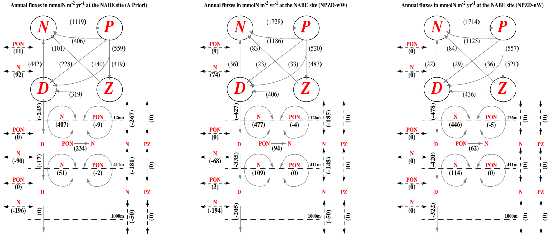
Figure 3.13: Simulated annual fluxes of nitrogen at 47°N20°W (NABE site). The units are mmol N m -2 yr -1 . LEFT: Resulting fluxes when a priori parameter values are used. MIDDLE: Fluxes of model with vertical velocities (NPZD-wW) when optimal parameter set is considered. RIGHT: Optimised model fluxes when neglecting vertical velocities. Only advection due the sinking of detritus (NPZD-nW) is allowed.
