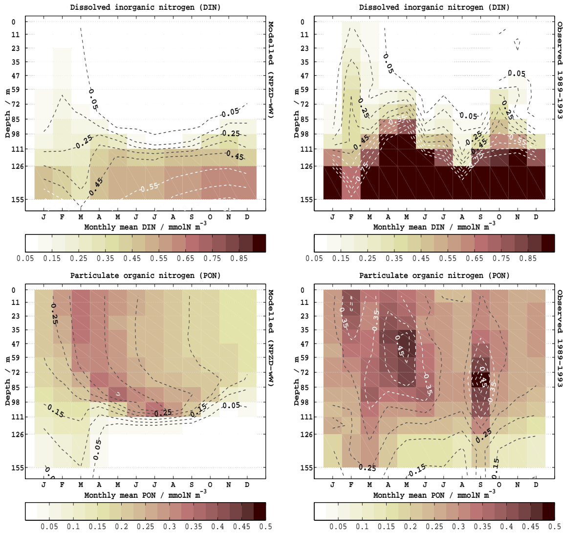
Figure 3.17: Monthly averaged concentrations of dissolved inorganic (contour interval=0.1 mmol N m -3 ) and particulate organic nitrogen (contour interval=0.05 mmol N m -3 ) within the upper 11 model grid cells: Modelled variables (left side) and the observational counterparts on the same grid (right side). Location: BATS site.
