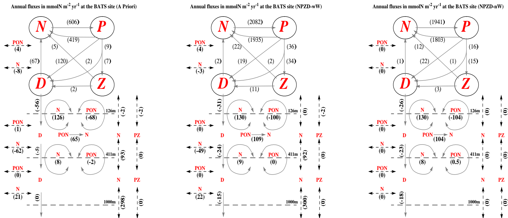
Figure 3.12: Simulated annual fluxes of nitrogen at 31^{\circ}\text{N } 64^{\circ}\text{W} (BATS site). The units are \text{mmol N m}^{-2} \text{yr}^{-1} . Vertical arrows illustrate vertical advective fluxes, with positive values meaning upward flux. Due to the divergence of the obtained vertical velocity field we must also solve for horizontal advective fluxes. This simply accounts for the continuity equation, conserving the water mass. LEFT: Resulting fluxes when a priori parameter values are used. MIDDLE: Fluxes of model with vertical velocities (NPZD-wW) when optimal parameter set is considered. RIGHT: Optimised model fluxes when neglecting vertical velocities. Only advection due the sinking of detritus (NPZD-nW) is allowed.
