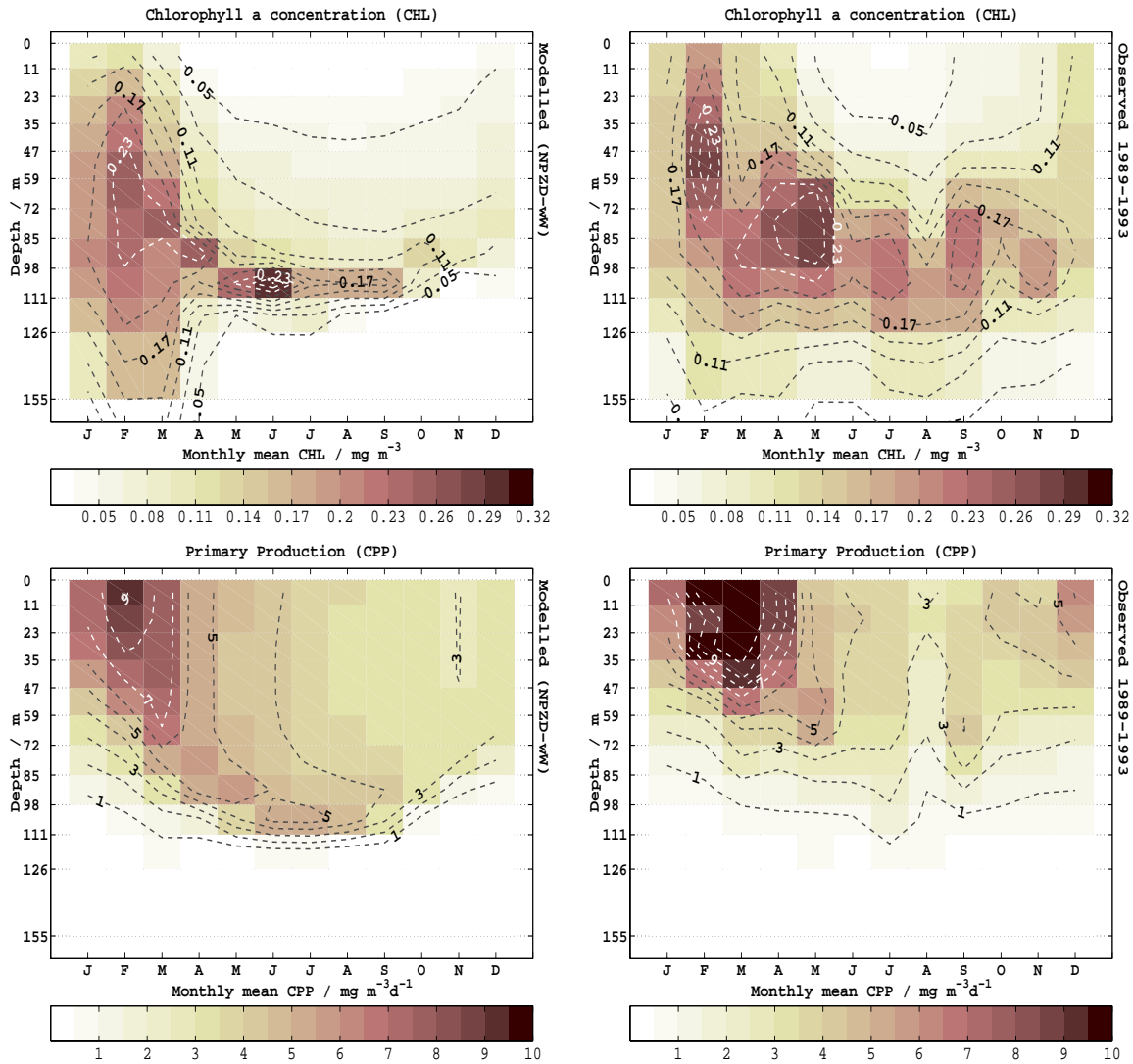
Figure 3.16: Monthly averaged chlorophyll concentration (contour interval=0.03 mg CHL \text{m}^{-3} ) and primary production (contour interval=1 mg C \text{m}^{-3}\text{d}^{-1} ) within the upper 11 model grid cells: Modelled variables (left side) and the observational counterparts on the same grid (right side). Location: BATS site.
