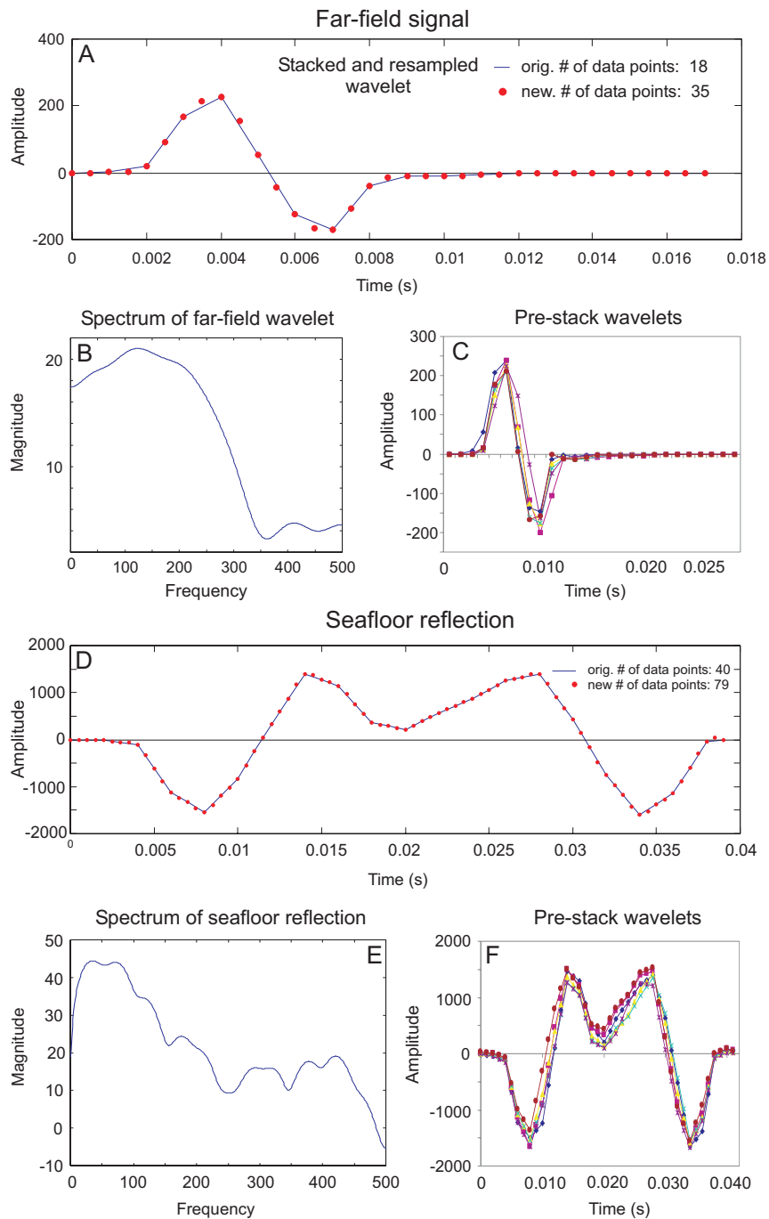
Fig. 4.1. Generator Injection gun (GI-gun) source signal characteristics. (C) matched far-field wavelets prior to stacking. (A) stacked and resampled far-field wavelet used for convolution. (B) spectrum of the far field source signal shown in (A). (D) matched sea floor reflections prior to stacking. (A) stacked and resampled sea floor used for convolution. (E) spectrum of the sea floor source signal shown in (A).
