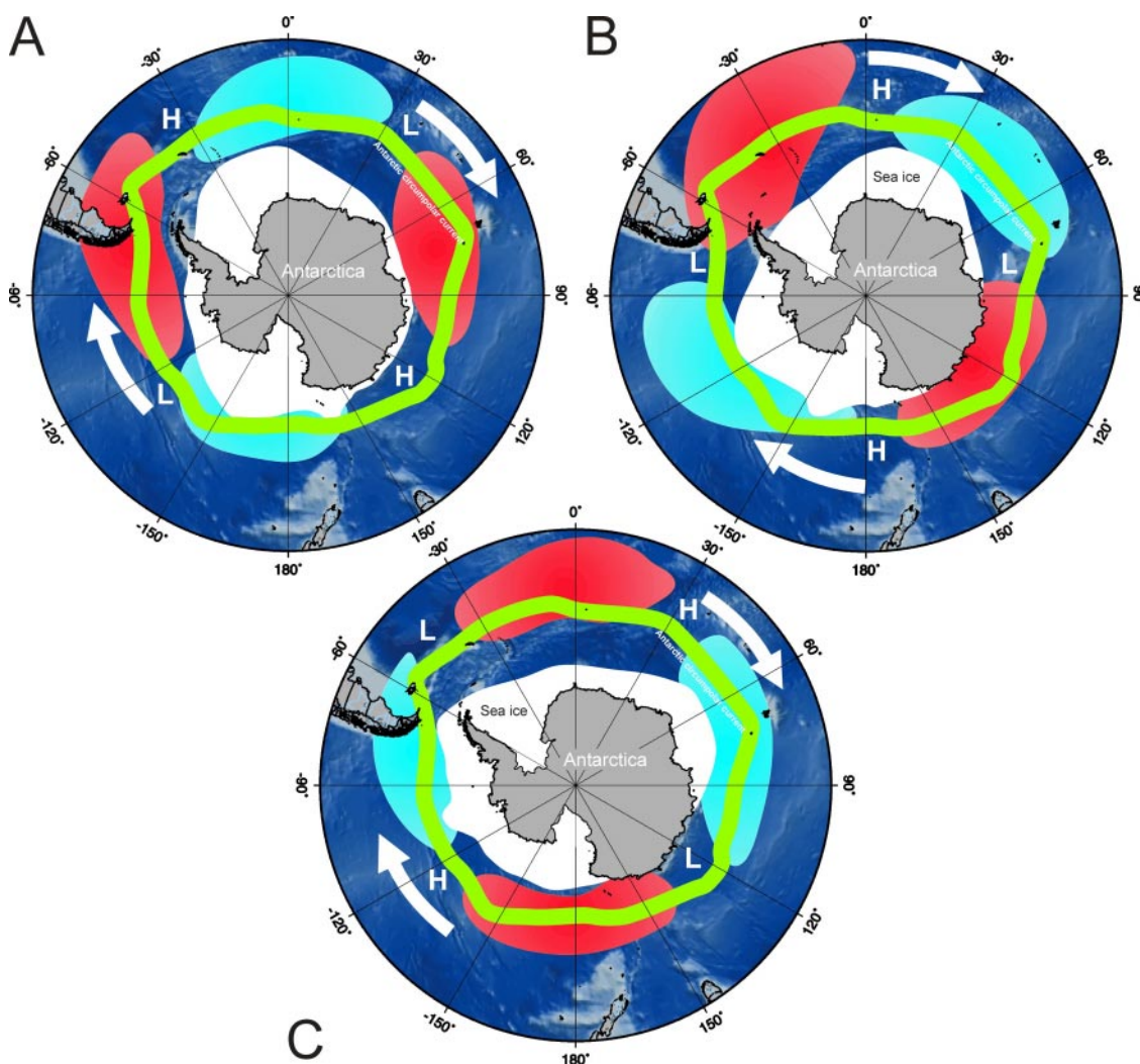
Fig. 1.3. Atmosphere-ocean interaction. Propelled by the ACC and atmospheric high and low pressure systems (H,L) – areas of relatively warmer (red) and colder (blue) water are driven around Antarctica. These anomalies propagate eastward with the circumpolar flow, with a period of 4-5 years and taking 8-10 years to encircle the pole. The system of coupled anomalies is called the Antarctic Circumpolar Wave and plays an important role in heat exchange between the South Pacific and the South Atlantic and climate regulation and dynamics both within and beyond the Southern Ocean. (Courtesy: White and Peterson, 1996, Figure modified from National Geographic, October 2000: „ New Eyes on the Oceans “, p.94.)
