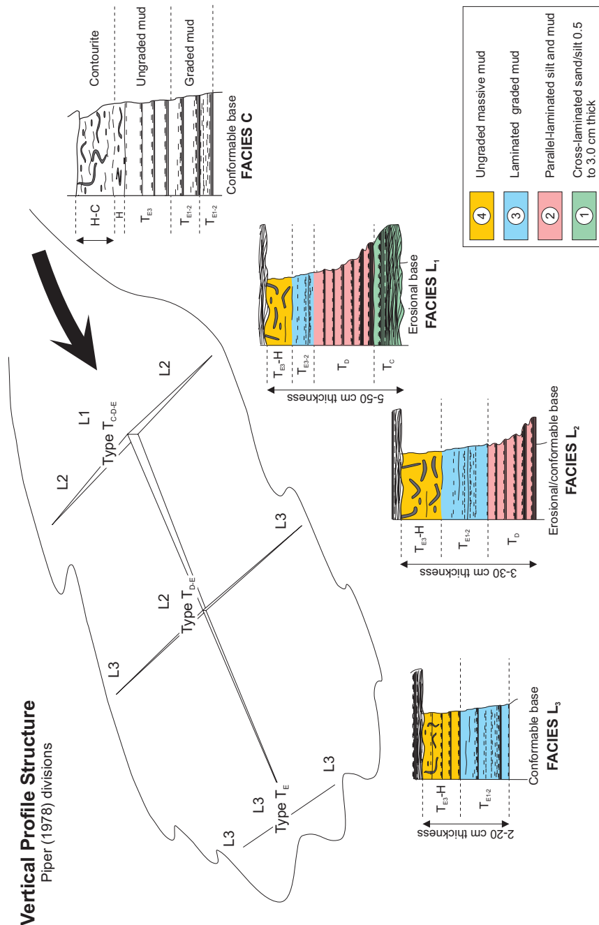
Fig. 4.1. Schematic diagram showing typical downslope and across-slope relationship between turbidite Facies L1, L2, and L3 as proposed by Stow and Piper (1984). Schematic representation of internal structure of facies within turbidites recovered during Leg 178. The standard Bouma scheme is refined with a descriptive classification for muddy turbidites (Piper, 1978). Facies C (contourite) is similar in the lower part to Facies L3 but with a contourite influenced in the facies subdivisions H-C. Facies C can occur as an ancillary component in the hemipelagic H interval of fine-grained muddy turbidite Facies L1-3. Figure modified from ODP Leg 178 Shipboard Scientific Party 1999.
