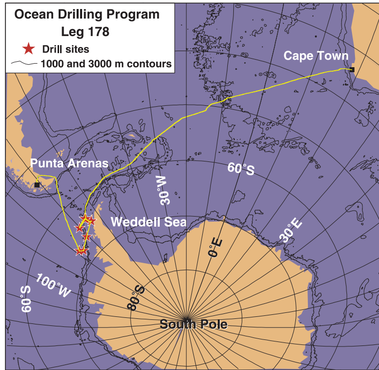
Fig. 1.1. General map of Leg 178 ship track with drill sites stated (Shipboard Scientific Party, 1999).
