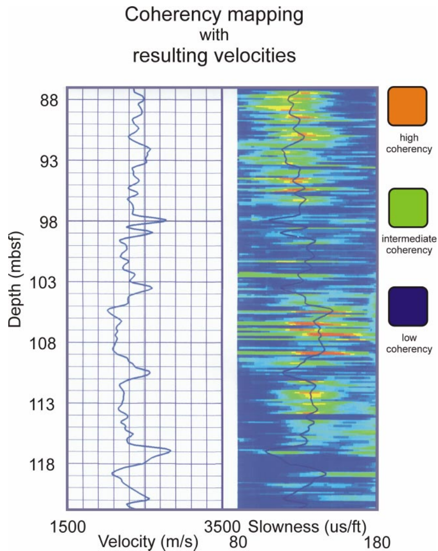
Fig. 2.2. Example of digital coherency mapping performed with data of logging run two, based on the tracking of highly coherent velocity values. The coherency values within the slowness range (80–180 \mu s) are color coded (right side). The resulting velocity values are shown on the left side.
