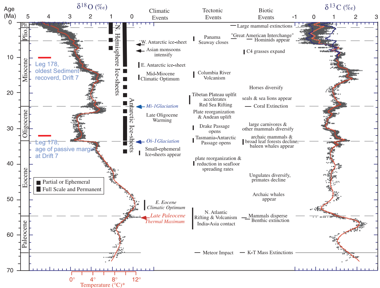
Fig. 1.2. Summary of global deep-sea oxygen and carbon isotope records based on data compiled from more than ~50 DSDP and ODP Leg 178 sites with pelagic sedimentary sections, dominated by fine-grained, carbonate-rich (>50%) oozes or chalks. Most of the data are derived from analyses of Cibicidoides and Nuttallides . To correct for genus-specific isotope vital effects, the \delta^{18}\text{O} values were adjusted by +0.64 and +0.4 ‰, respectively. The absolute ages are based on the time scale of Berggren et al. (1995). The raw data were smoothed with a 5 point running average and a locally weighted mean. The carbon isotope record shows separate curve fits for the Atlantic (blue) and Pacific above the middle Miocene, illustrating the increase in basin-to-basin fractionation that exceeds \sim 1.0 ‰ in some intervals. Prior to 15 Ma, interbasin gradients are insignificant or nonexistent. The \delta^{18}\text{O} temperature scale was computed for an ice-free ocean [ \sim 1.2 ‰ Standard Mean Ocean Water (SMOW)], and thus only applies to the time preceding the onset of large-scale glaciation on Antarctica ( \sim 35 Ma). From the early Oligocene to present, much of the variability ( \sim 70\% ) in the \delta^{18}\text{O} record reflects changes in Antarctic and Northern Hemisphere ice volume. The vertical bars provide a rough qualitative representation of ice volume in each hemisphere relative to the Last Glacial Maximum (LGM), with the dashed bar representing periods of minimal ice coverage ( \leq 50\% ), and the full bar representing close to maximum ice coverage ( >50\% of present). Some key tectonic and biotic events are listed as well. Reprinted with minor additions by permission of Zachos et al. (2001). Refer to the original paper for details.
