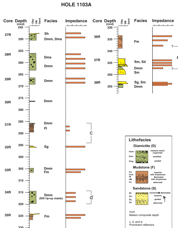
Fig. 2.1. Simplified lithostratigraphy showing lithofacies impedance indicators and possible reflector tops of the seismostratigraphic unit S3 below the major shelf unconformity at Site 1103 A. Refer to the text for characterization of the facies types. Modified from Shipboard Scientific Party (1999), the Figure has been rescaled to represent true thickness of recovered intervals and depth scale is converted to the mcd. Tentative impedance indicators have been added based on acoustic measurements on board the ship.
