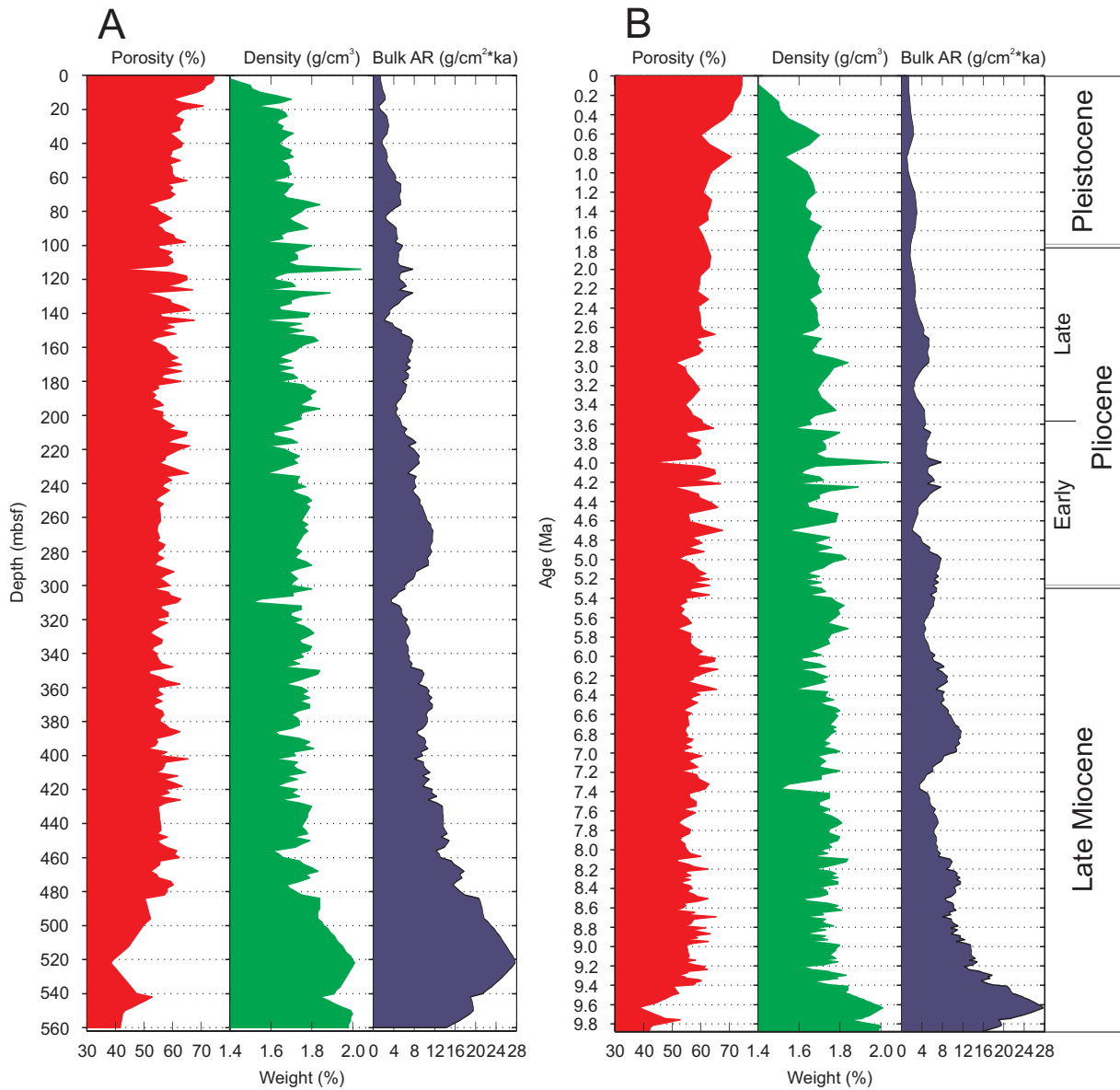
Fig. 4.3. Bulk accumulation rates (mass flux) of Site 1095 derived from the linear sedimentation rates of the „model 0.4“ shown in Fig. 4.1E and the porosity and density compilations of Volpi et al. (2001). Even though the bulk accumulation rates are heavily dominated by the sedimentation rates, the intervals with slightly higher densities (probably linked to glacial debris input) agree well with intervals of higher sedimentation (Fig. 4.1) and accumulation rates.
