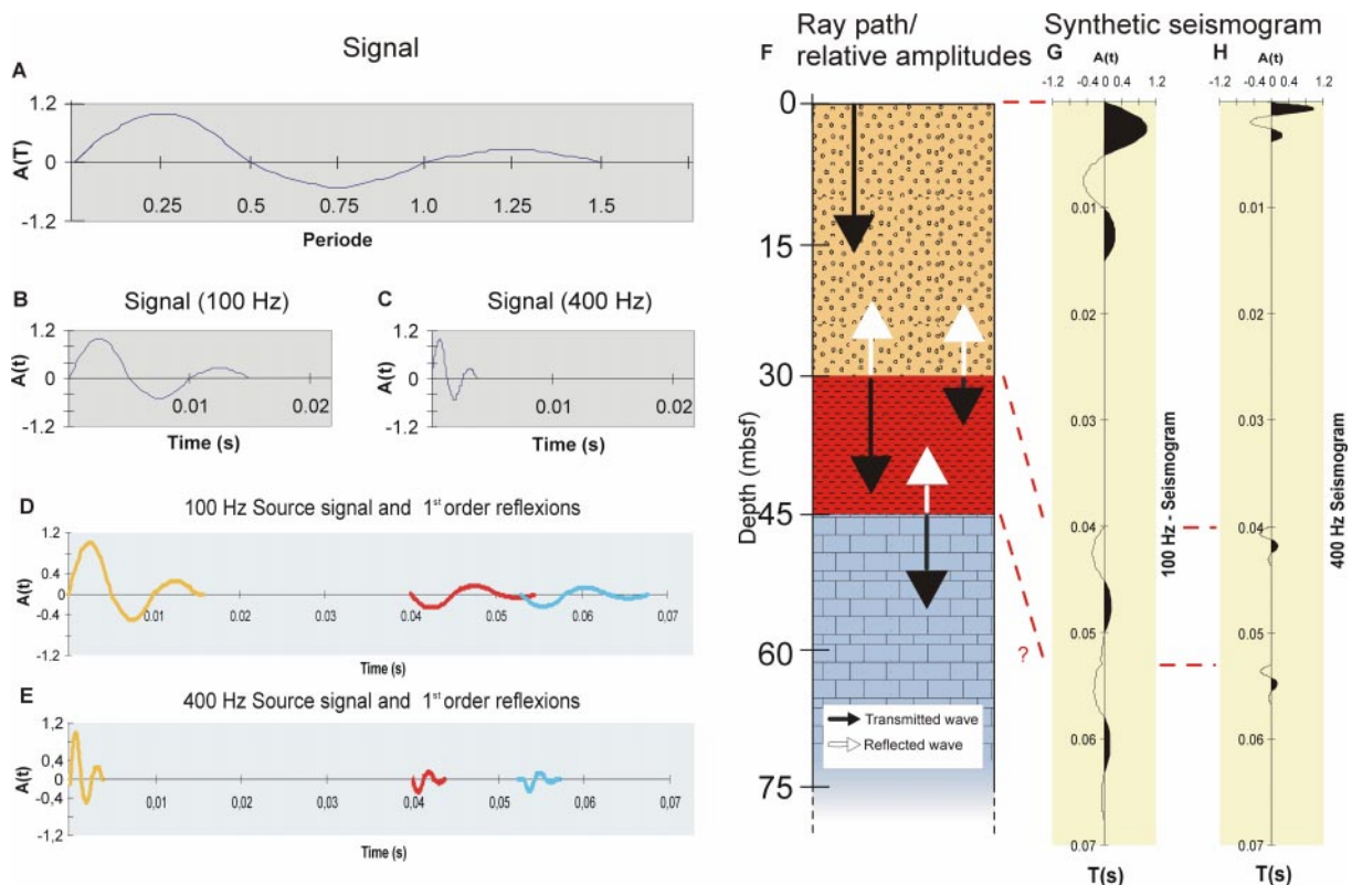
Fig. 7.3. Simplified illustration showing how source signal wavelets of the same amplitudes but different wavelengths travel through the earth model from Fig. 7.2. The ray path is indicated by direction of the arrows. The amounts of the reflected and transmitted amplitudes by the arrow length. Note the limitation due to interference of a wavelet with 100 Hz in detecting the 15 m thick clay stone layer. The 400 Hz wavelet reproduces all impedance contrasts unambiguously.
