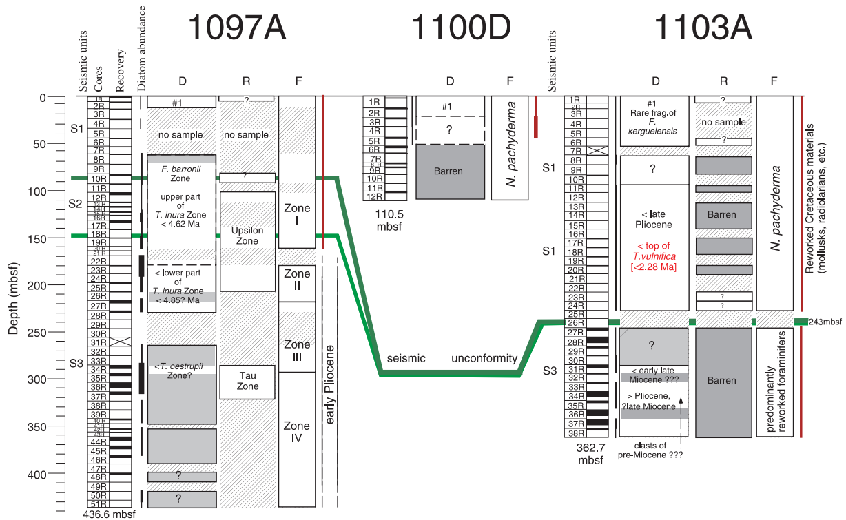
Fig. 2.1. Age constraints - Biostratigraphic summary of shelf sites (Holes 1097A (Fig. 1.2), 1100D, and 1103A (Fig. 2.1-Fig. 2.1)), based on shipboard observations and seismic correlation. Light gray horizons are material with very rare diatom occurrence. Age assignment of S3 (4.5-4.6 Ma, Camerlenghi et al., in press) at Hole 1097A is based on benthic foraminifers, diatoms, and radiolarian biostratigraphy. Age assignment of the base of S1 at Hole 1103A is based on diatom biostratigraphy. Dark gray horizons show intervals barren of microfossils. Note seismic unit S2 is missing at Site 1103 and the top of S3 at Site 1103 (early late Miocene) may be older than at Site 1097 (4.5-4.6 Ma). Noteworthy for later considerations: sediments above the unconformity S1/S3 contain the top of Thalassiosira vulnifica giving a minimum time constraint for the age of the unconformity.
