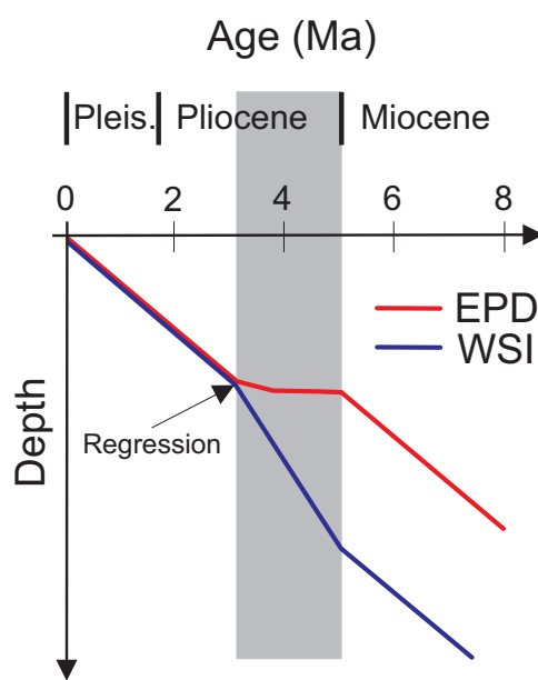
Fig. 1.2. Hypothetical sedimentation rates on the continental rise for a warmer early Pliocene. Depositional scenario of Barker (1995) for a proposed Warm Stable Ice Sheet hypothesis (WSI, blue line) and Early Pliocene Deglaciation (EPD, red line). Both scenarios reunite at the beginning of the late Pliocene/Pleistocene Northern Hemisphere Glaciation, leading to a regression (modified from Barker, 1995).
