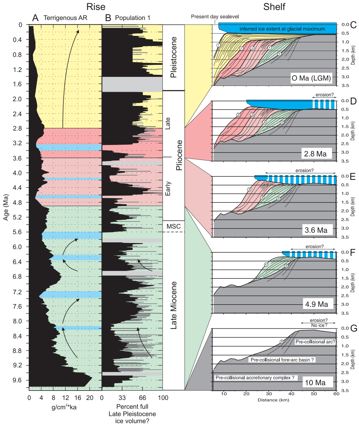
Fig. 5.1. Correlation of (A) terrigenous accumulation rates at the rise Site 1095 with (B) ice-indicator signal derived from grain-size data. Note the lows in accumulation at times of reduced ice volume or decreased frequency of ice advances to the shelf edge (blue bars = correlation bars, gray bars = gap in data; MSC = Messinian Salinity Crisis). (C-G) Backstripping model of the shelf (Camerlenghi et al., 2001, with modified ages).
