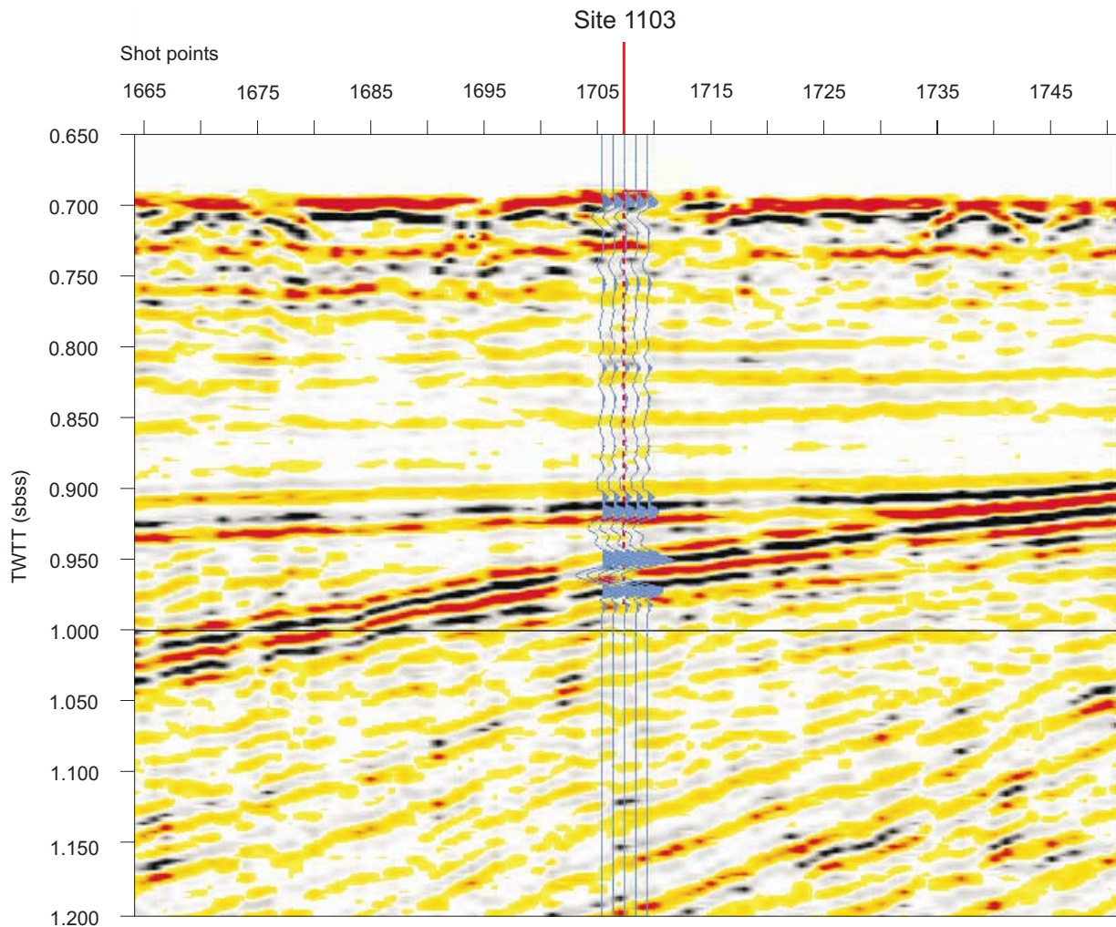
Fig. 2.2. The new synthetic traces overlain on part of MCS line I95-152. The major reflectors are in place – indicating an overall correct velocity model. For the seismic section red indicates positive amplitudes and black negative. Note that TWTT is given in sbss (seconds below sea surface), see notes Fig. 2.1. See text for detailed discussion of the comparison. Figure received and modified from Trevor Williams of the Borehole Research Group at Lamont-Doherty Earth Observatory.
