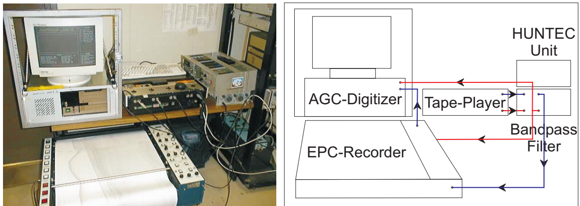
Fig. 3.1. Atlantic Geoscience Center (AGC) digitizing unit. The data on analog tape is played back and filtered. The trigger channel (blue line, standardizing of the trigger pulse) and the data channel (red line) are first fed into an EPC recorder (online display). The 12 bit AGC unit is working trace oriented with fixed samples in each trace and uses the trigger pulse for the start of a new trace. Data after the trigger pulse is lost due to a fixed delay set at the beginning of the trace to fade out most of the water column.
