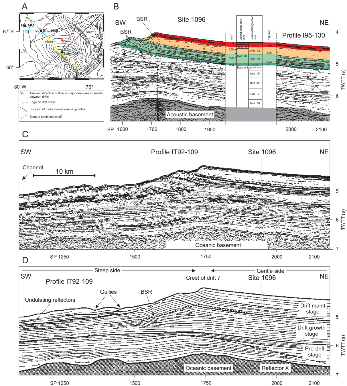
Fig. 4.1. Seismic profiles across Drift 7, parallel to the margin. (A) Location map of seismic profile sections. (B) Profile I95-130 across Site 1096, parallel to the margin. Lithostratigraphic and seimostratigraphic boundaries are shown together with an approximate depth and age scale. Note the upper and lower bottom simulating reflectors (BSR). The upper BSR was first noted by ODP Leg 178 Shipboard Scientific Party, 1999. It had not been identified on the 1992 profiles (C,D) . (D) schematic interpretive line drawing of C with the interpretation of various drift stages (Rebesco et al., 1997; 1996). Possible explanations for the origin of “Reflector X” are discussed in chapter 4.5.2.
