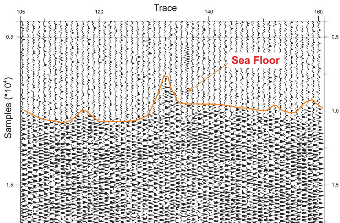
Fig. 3.2. Large static shifts distort the single channel record digitized with the AGC Unit. Most likely cause are poorly-detected trigger pulses.
