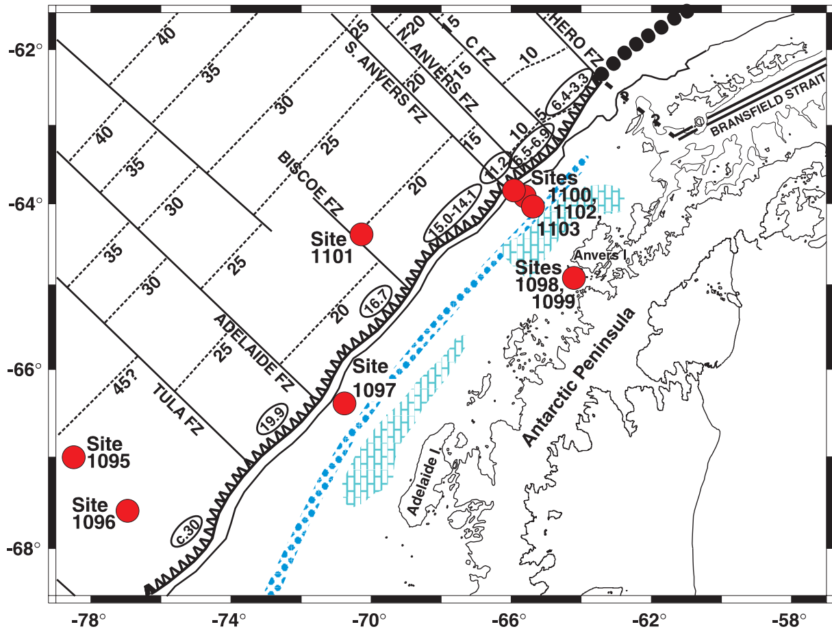
Fig. 3.1. Ages of ocean floor and ridge crest–trench collisions along the Antarctic Peninsula Pacific margin with drill sites marked (based on the time scale of Cande and Kent, 1995). The mid-shelf high and the shelf basins are marked as dots and bars signatures respectively (Courtesy: ODP Leg 178 Shipboard Scientific Party, 1999).
