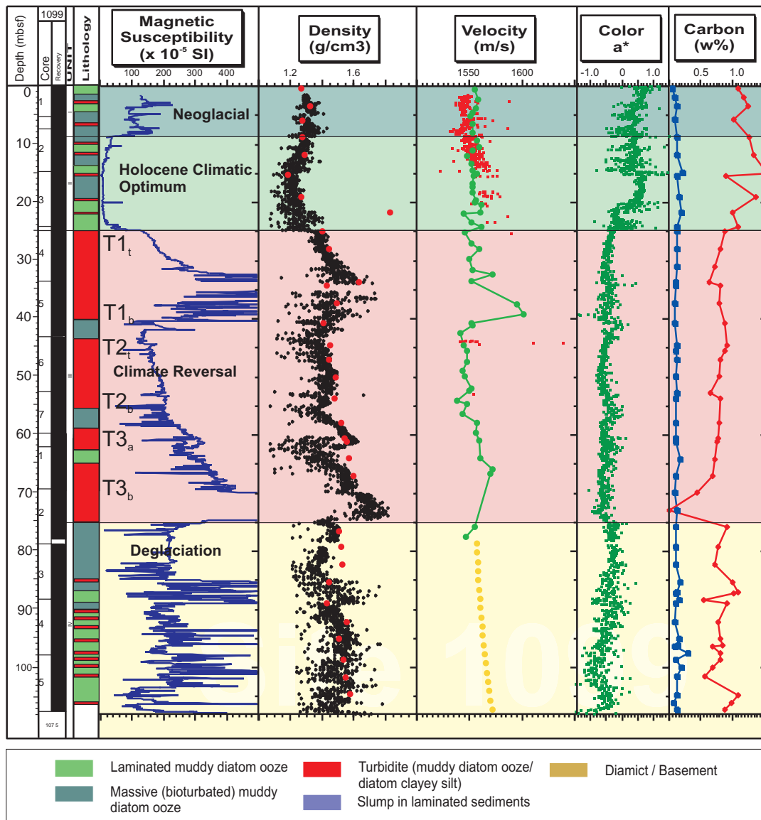
Fig. 3.3. Lithology summary chart of Site 1099. See Fig.1.6 for the labels of the climatic zones (colored horizontal sections). See text for details. Note the correlation of magnetic susceptibility highs with the base of turbidites, and corresponding highs in density and velocity (e.g. interval 25 to 40 mbsf). The velocity record below 75 meters was severely degraded due to close spaced horizontal gas expansion cracks within the core. A polynomial fit is used instead (connected yellow dots).
