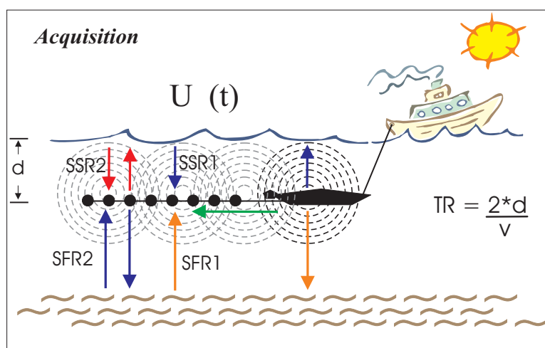
Fig. 3.1. Data acquisition with the HDTB System. The tow depth ( d ) of the fish and the sea water velocity ( v ) determine the maximum time window available for receiving data unaffected by the arrival of the sea surface return.
