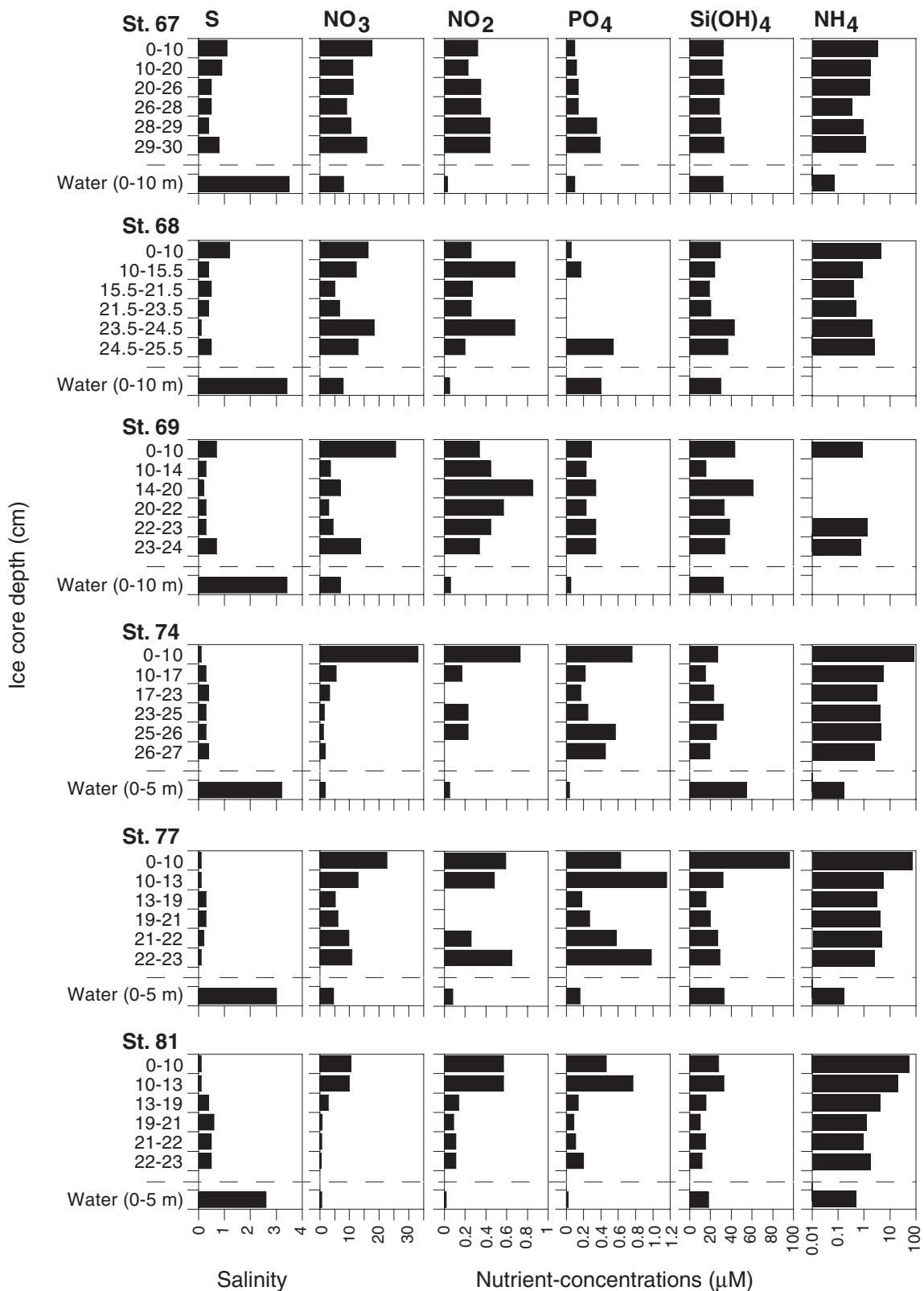
Fig. 2.1.3: Vertical distribution patterns of salinity, nitrate (NO 3 ), nitrite (NO 2 ), phosphate (PO 4 ), silicate (Si(OH) 4 ) and ammonia (NH 4 ) in sea ice and values for the underlying water. Note logarithmic scale for NH 4 . All nutrient data from the ice core sections are normalised to the salinity of the under-ice water of the same station. NO 2 , PO 4 and NH 4 were measured in all samples, but concentrations were below detection limits in few cases.
