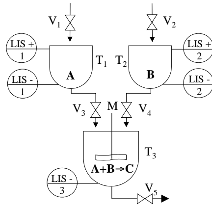
Figure 5.2: The plant
