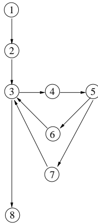
Figure 3.7: A data flow graph
