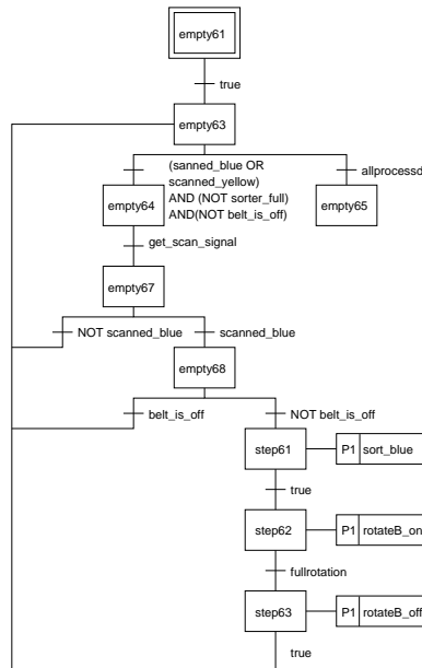
Figure 6.3: Sub-SFC of the control process
