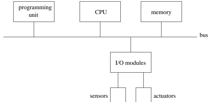
Figure 1.1: PLC architecture
