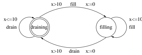
Figure 3.2: Timed automaton for a tank model
