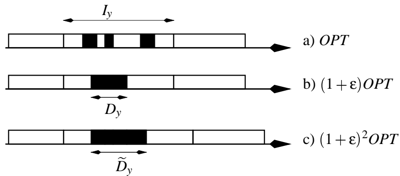
Figure 1.12: Scheduling inside interval I_y
