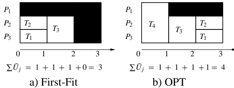
Figure 4.5: First-Fit scheduling of parallel tasks T_1, T_2, T_3 and T_4
