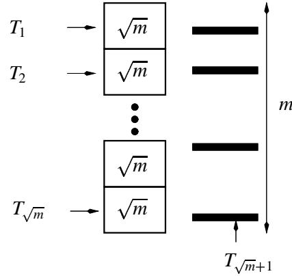
Figure 4.26: Tasks T_1, T_2, \dots, T_q and T_{q+1} , where m = q^2
