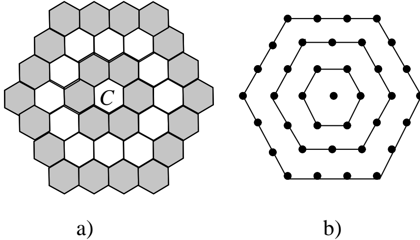
Figure 2.10: Labeling of C
