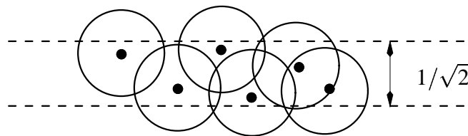
Figure 2.17: A \frac{1}{\sqrt{2}} -strip unit disk graph
