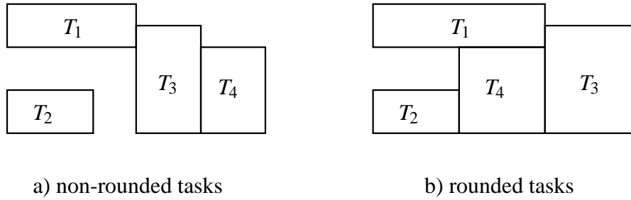
Figure 3.8: Scheduling 4 tasks
