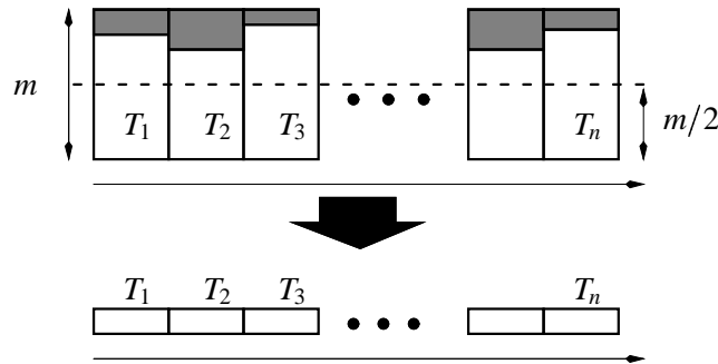
Figure 4.7: Scheduling large tasks
