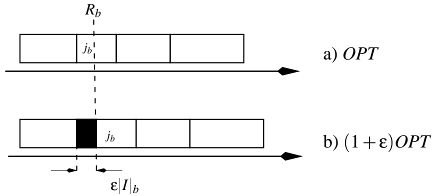
Figure 1.9: A job j_b with R_b \in (S_{j_b}, C_{j_b}]
