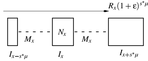
Figure 1.17: Interval I_x with sets N_x and M_x
