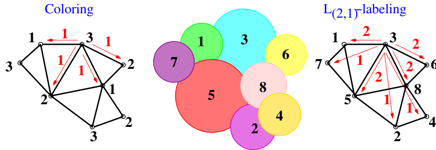
Figure 2.3: FAP – L_{(2,1)} -labeling
