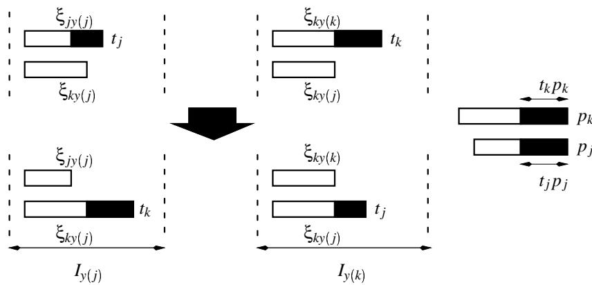
Figure 1.11: The y(j), y(k) th fractions of jobs k and j
