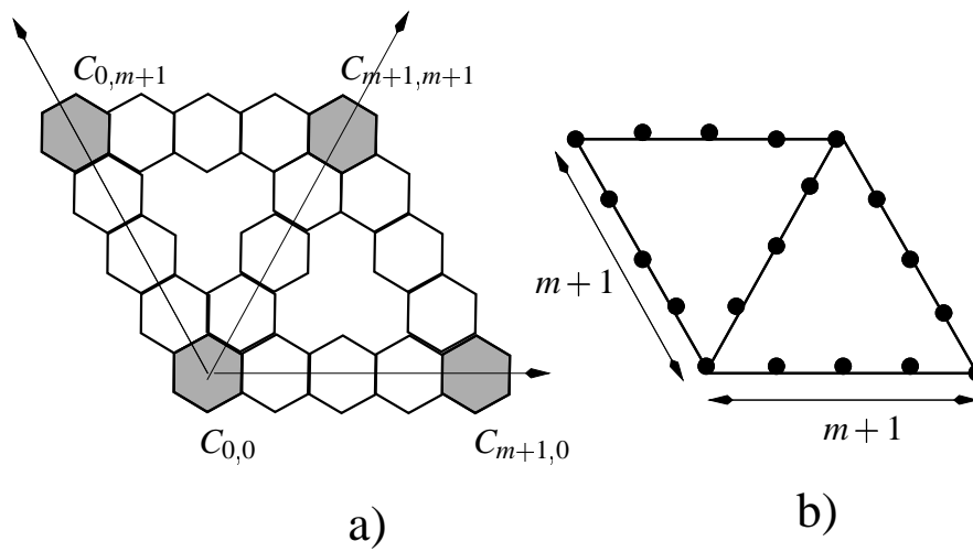
Figure 2.6: Cells for i = 0 and j = 0 and t = m + 1
