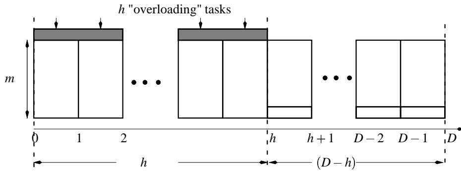
Figure 4.18: “Overloading”
