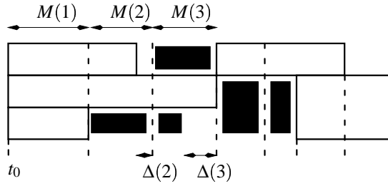
Figure 1.31: Deducing a schedule
