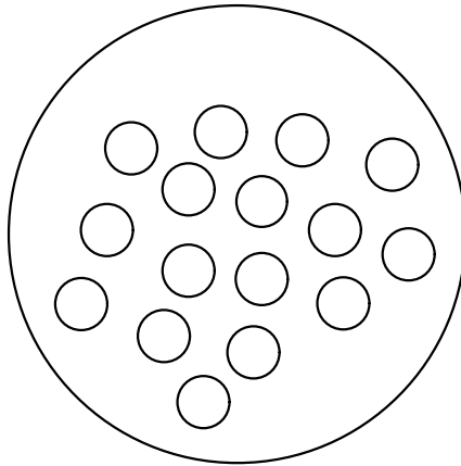
Figure 2.14: A set D of disks
