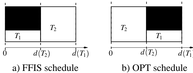
Figure 4.13: Scheduling tasks T_1 and T_2
