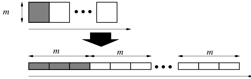
Figure 4.9: Scheduling parallel tasks of size one
