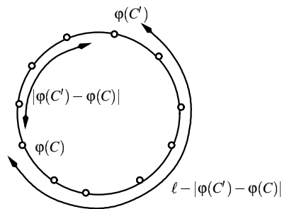
Figure 2.9: A circle with \ell nodes, and cells C and C'
