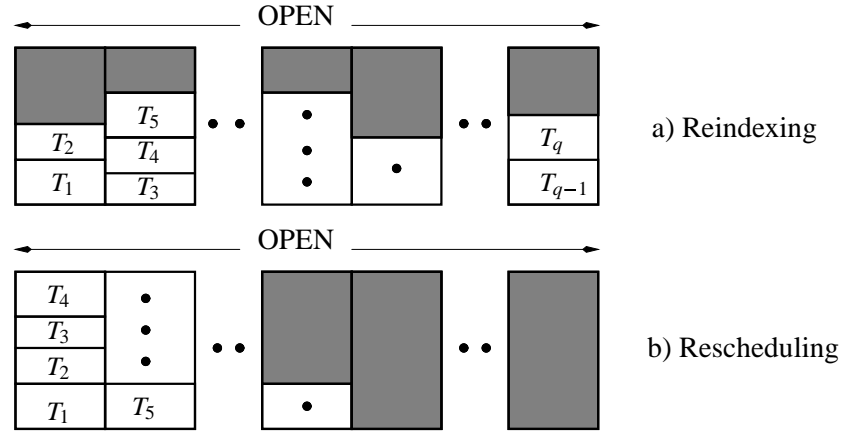
Figure 4.21: Reindexing and rescheduling of small tasks
