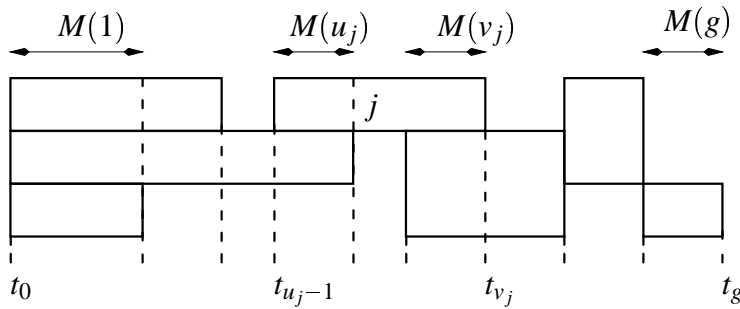
Figure 1.29: Long task j in a relative schedule
