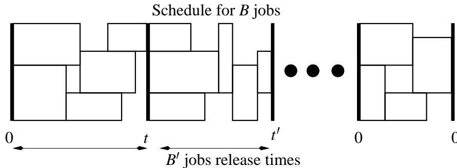
Figure 3.10: Passive-Active-Bin scheduling
