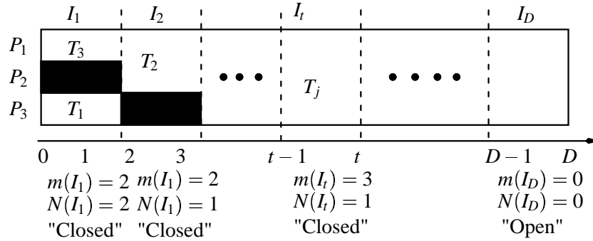
Figure 4.3: Scheduling on time slots
