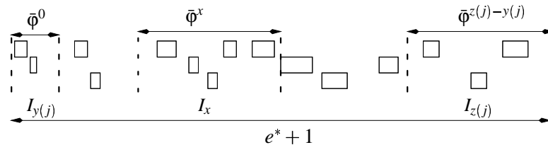
Figure 1.18: Local profiles of job j
