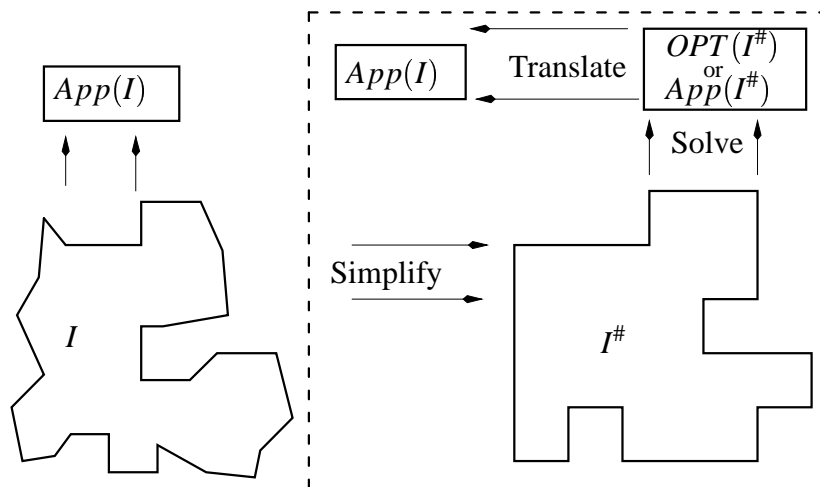
Figure 1.2: Simplifying of the instance
