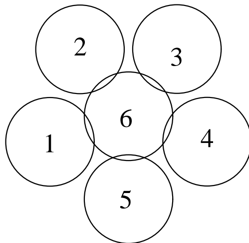
Figure 2.13: Graph G_{\text{bad}} for L_{2,1} -labeling
