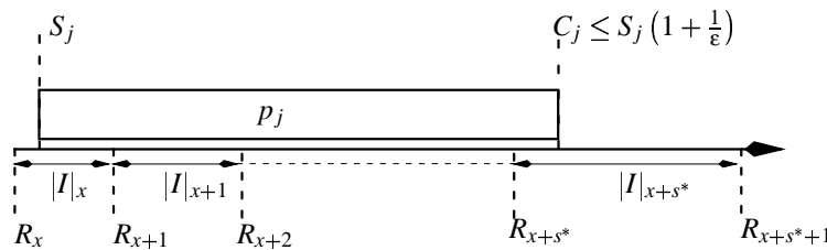
Figure 1.7: A crossing job j
