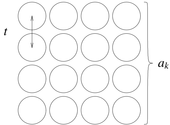
Figure 2.15: The set D of a_k^2 unit disks
