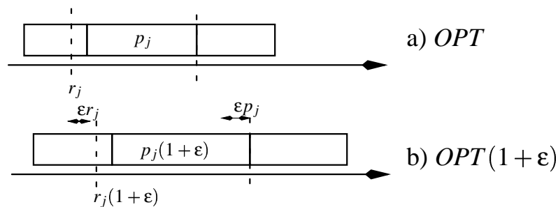
Figure 1.4: Geometric rounding
