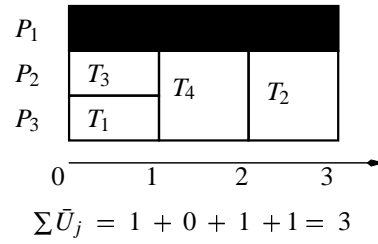
Figure 4.1: Scheduling parallel tasks T_1, T_2, T_3 and T_4
