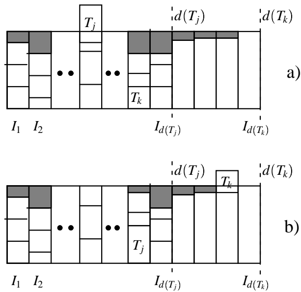
Figure 4.17: Loading tasks T_j and T_k
