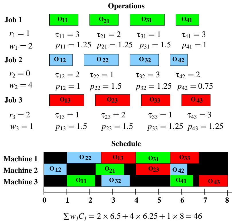
Figure 1.14: A schedule for 3 jobs
