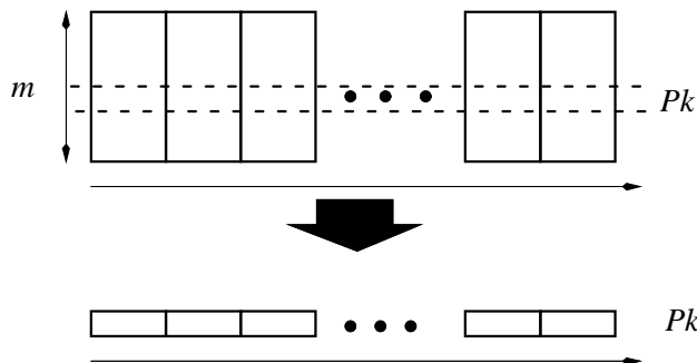
Figure 4.8: Scheduling dedicated tasks of size one
