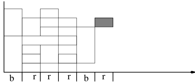
Figure 3.6: Red and blue intervals in a schedule
