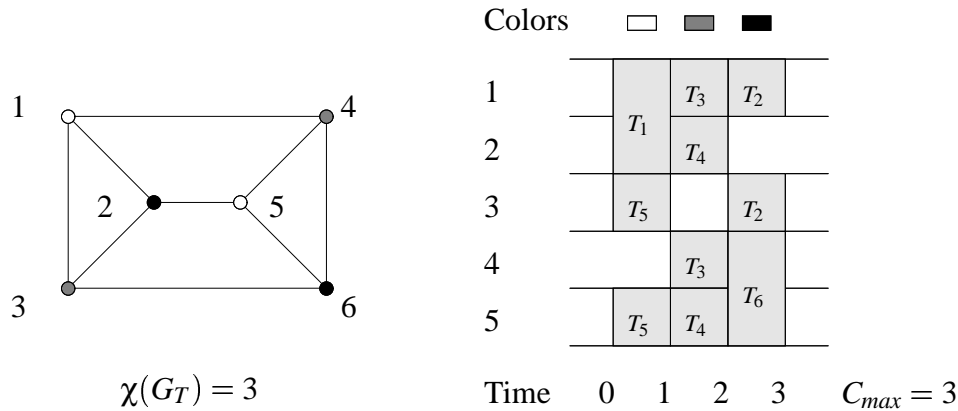
Figure 3.5: Scheduling of T = \{1, 2, 3, 4, 5, 6\} and coloring of G_T
