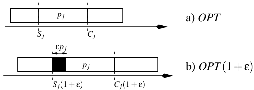
Figure 1.6: Stretching of a schedule
