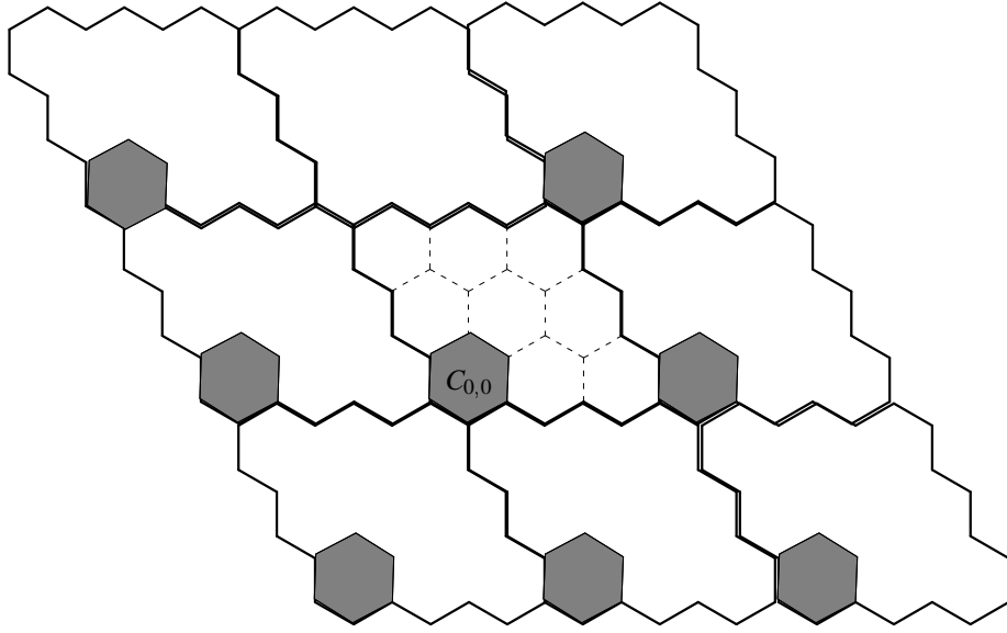
Figure 2.8: Shifting the pattern: The copies of C_{0,0}
