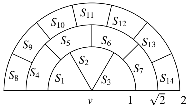
Figure 2.23: The sector partition around a vertex v
