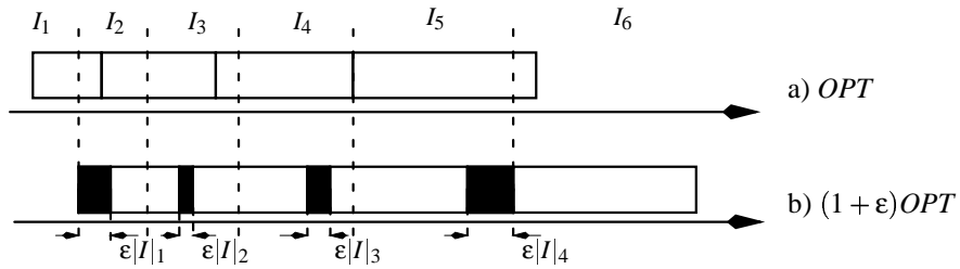
Figure 1.8: Time-stretching
