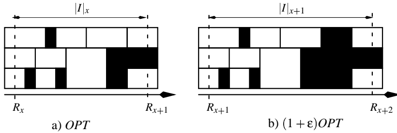
Figure 1.28: Tasks in interval I_{x+1}
