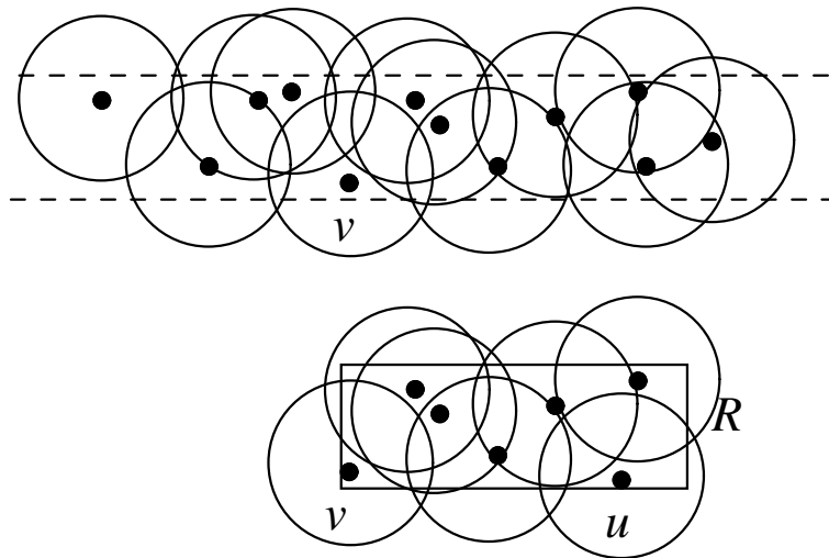
Figure 2.20: A vertex v \in V(G) and a vertex u \in N_{G^2}(v)
