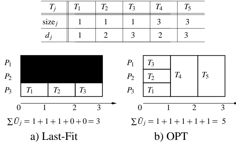
Figure 4.6: Latest-Fit scheduling of parallel tasks T_1, T_2, T_3, T_4 and T_5
