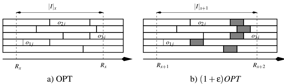
Figure 1.21: Operations in interval I_x and I_{x+1}
