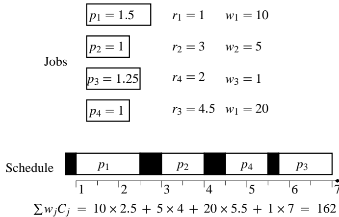
Figure 1.3: A schedule for 4 jobs
