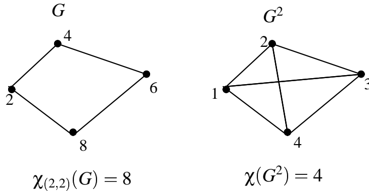
Figure 2.18: An L_{(2,2)} -labeling of G and a coloring of G^2
