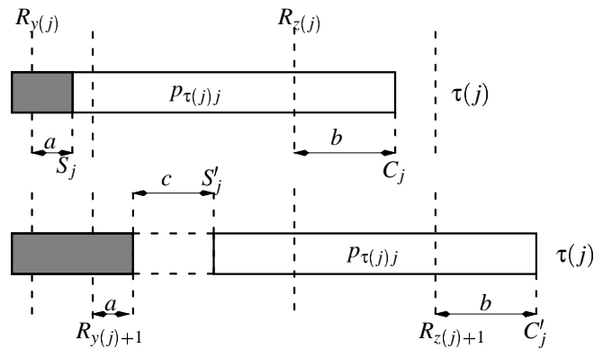
Figure 1.26: Shifting
