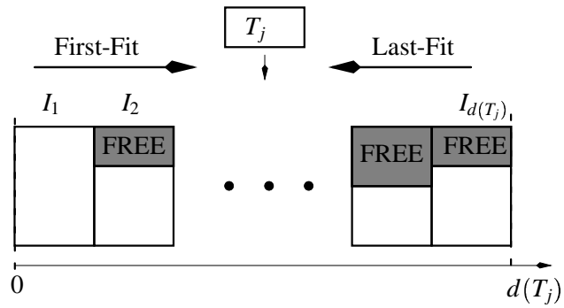
Figure 4.4: First-Fit and Last-Fit for task T_j
