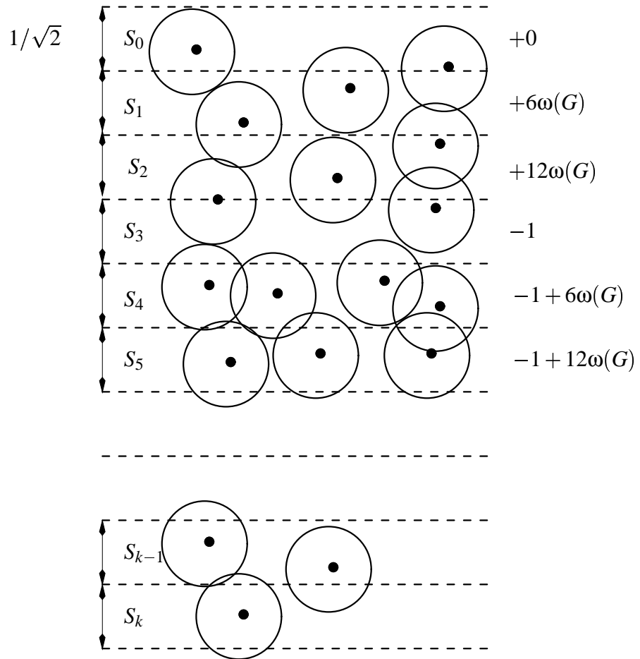
Figure 2.21: Strips S_0, S_1, \dots, S_k
