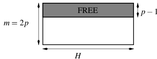
Figure 4.24: Free time for m = 2p
