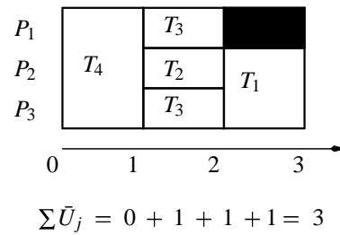
Figure 4.2: Scheduling dedicated tasks T_1, T_2, T_3 and T_4
