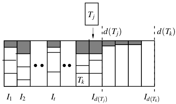
Figure 4.16: Tasks T_j and T_k in the LFIS schedule
