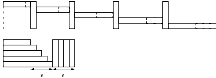
Figure 3.7: The output and optimal schedules
