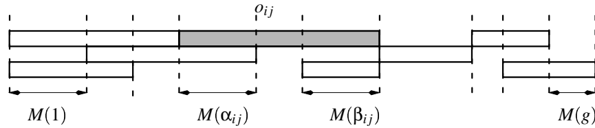
Figure 1.22: A relative schedule and an operation o_{ij}
