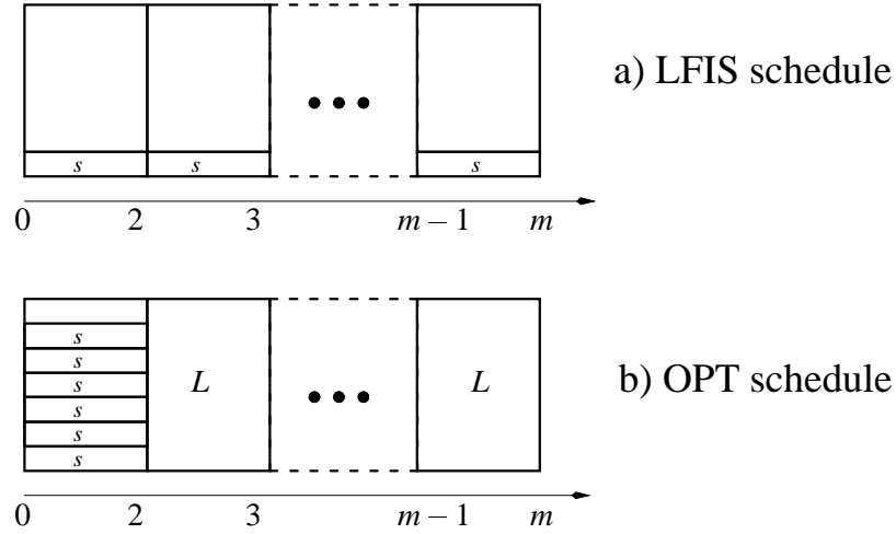
Figure 4.14: Scheduling small and large tasks
