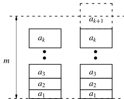
Figure 4.11: Items a_1, a_2, \dots, a_k and a_{k+1}
