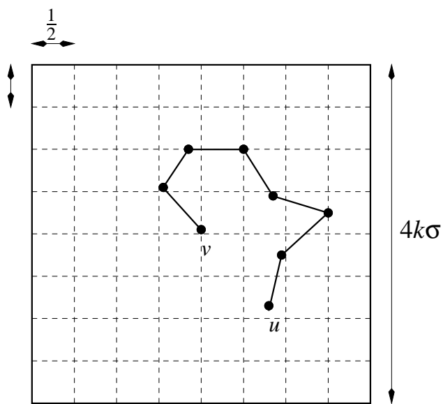
Figure 2.25: A square S at a vertex v
