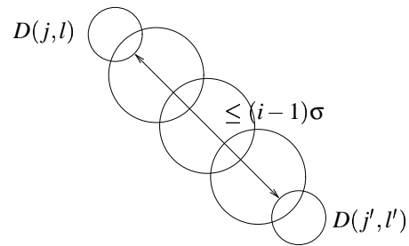
Figure 2.16: Disks D_{j,l} and D_{j',l'}
