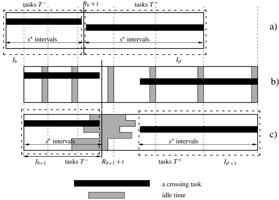
Figure 1.27: Creating a gap
