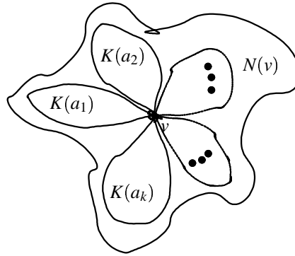
Figure 3.4: A vertex v and N(v)
