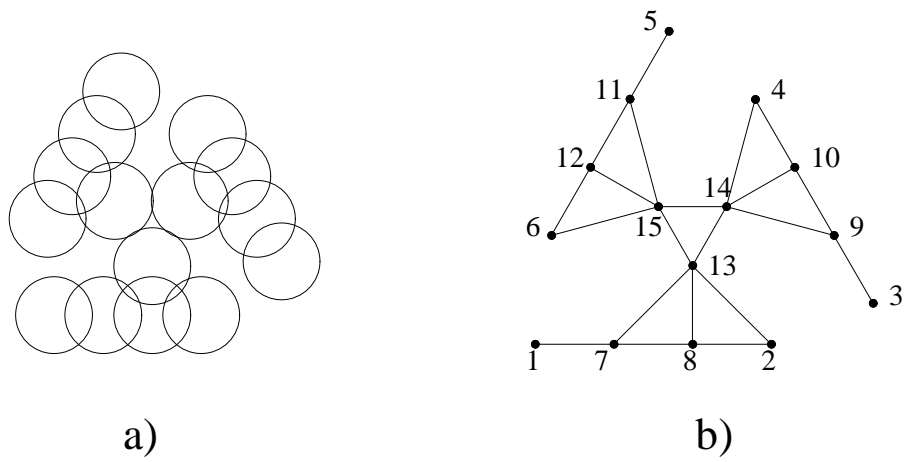
Figure 2.12: Graph G_{\text{bad}} for coloring
