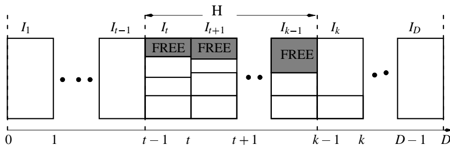
Figure 4.23: The LFIS schedule
