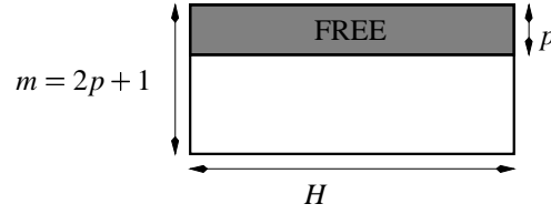
Figure 4.25: Free time for m = 2p + 1
