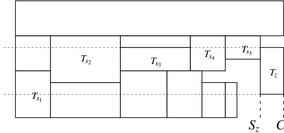
Figure 3.9: A task z and a sequence s_1, s_2, s_3, s_4, s_5
