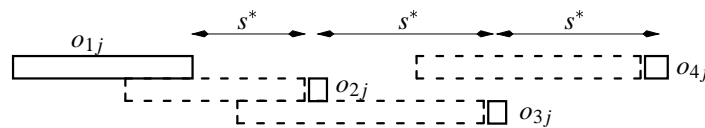
Figure 1.16: Main operation o_{1j} and negligible operations o_{2j}, o_{3j}, o_{4j}
