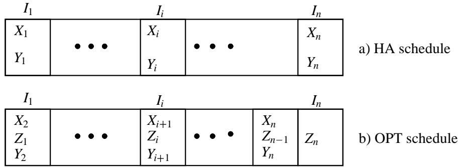
Figure 4.22: Scheduling tasks X_i, Y_i, Z_i
