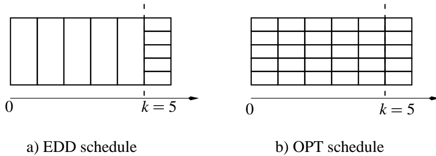
Figure 4.10: Scheduling k large and m(k + 1) small tasks in EDD order, for k = 5 and m = 5
