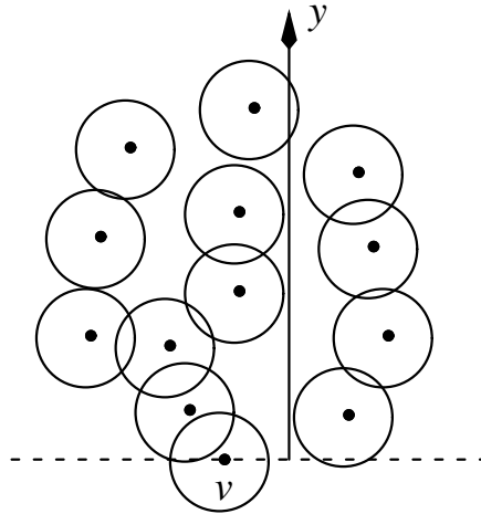
Figure 2.22: A vertex v with the least y -coordinate
