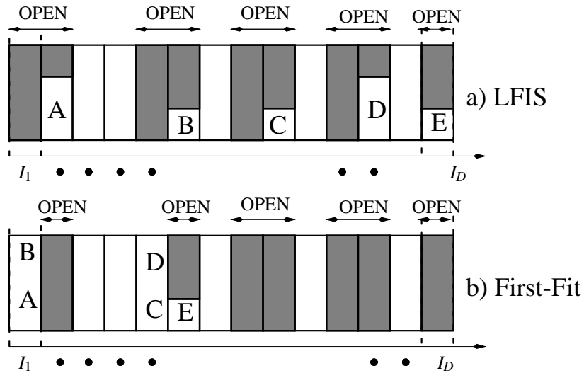
Figure 4.20: Scheduling small tasks
