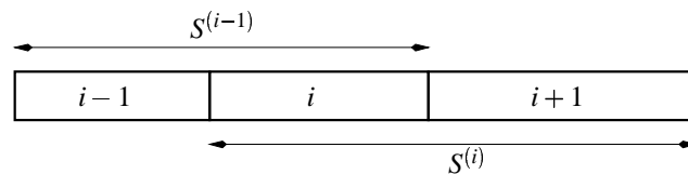
Figure 1.13: Pseudo-schedules S^{(i)} and S^{(i-1)} for block i
