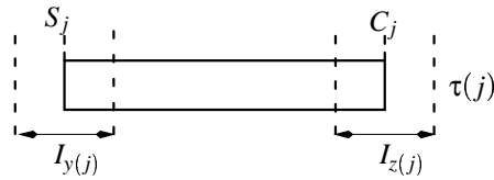
Figure 1.25: Indices
