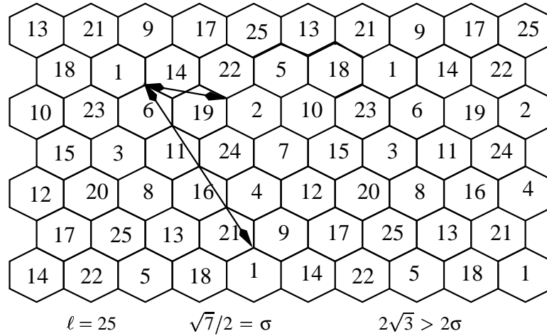
Figure 2.11: A 25-circular labeling with (p_1, p_2) = (2, 1) , \sigma = \frac{\sqrt{7}}{2}
