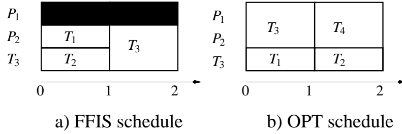
Figure 4.12: Scheduling tasks T_1, T_2, T_3 and T_4
