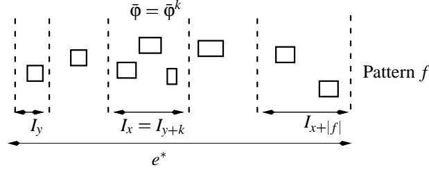
Figure 1.20: Pattern f and its load in an interval I_x
