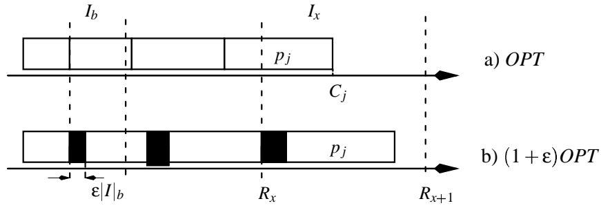
Figure 1.10: A job j with C_j \in I_x
