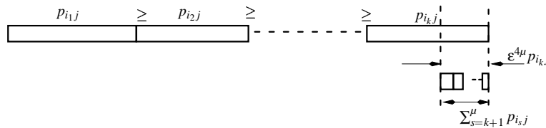
Figure 1.15: Main and negligible operations
