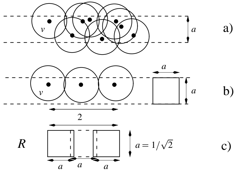
Figure 2.19: A \frac{1}{\sqrt{2}} -strip unit disk graph
