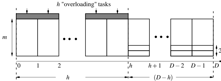
Figure 4.19: "Overloading"
