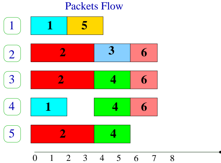
Figure 3.3: A schedule
