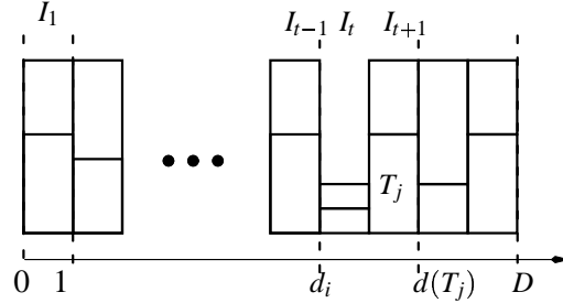
Figure 4.15: A tasks T_j with d(T_j) > d_i
