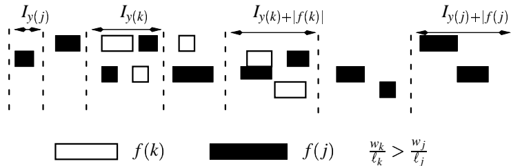
Figure 1.19: Smith's rule for jobs k and j
