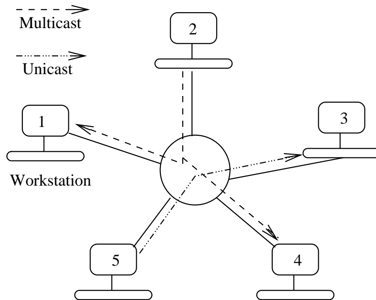
Figure 3.1: A passive-star-based local optical WDM network
