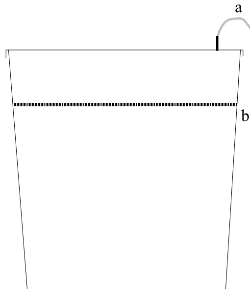
Figure 5.2: Experimental container. a - aeration tube; b - water level. Volume of the medium was 25 L.
