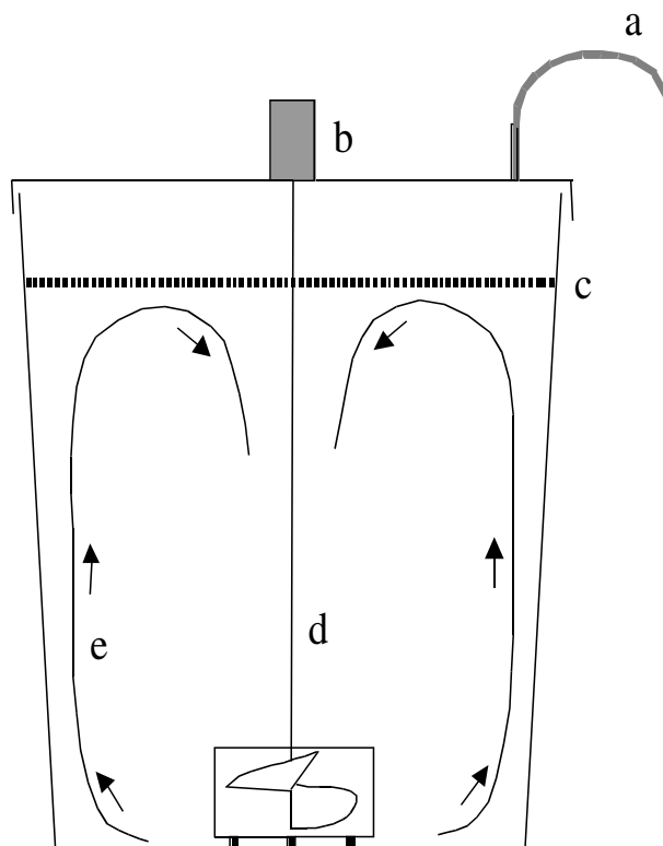
Figure 6.1: Container for permanent cultivation of calanoid copepods. Volume of the medium appr. 25 L. a - aeration tube; b - engine; c - water level; d - glass stick with screw; e - induced current.
