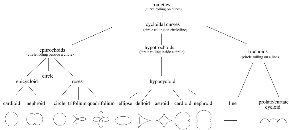
Fig. 6.5: Subtree of algebraic curves.
