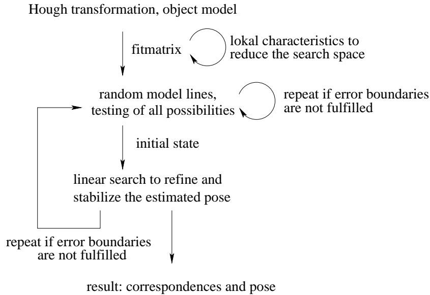
Fig. B.4: A scheme of the tracking algorithm.
