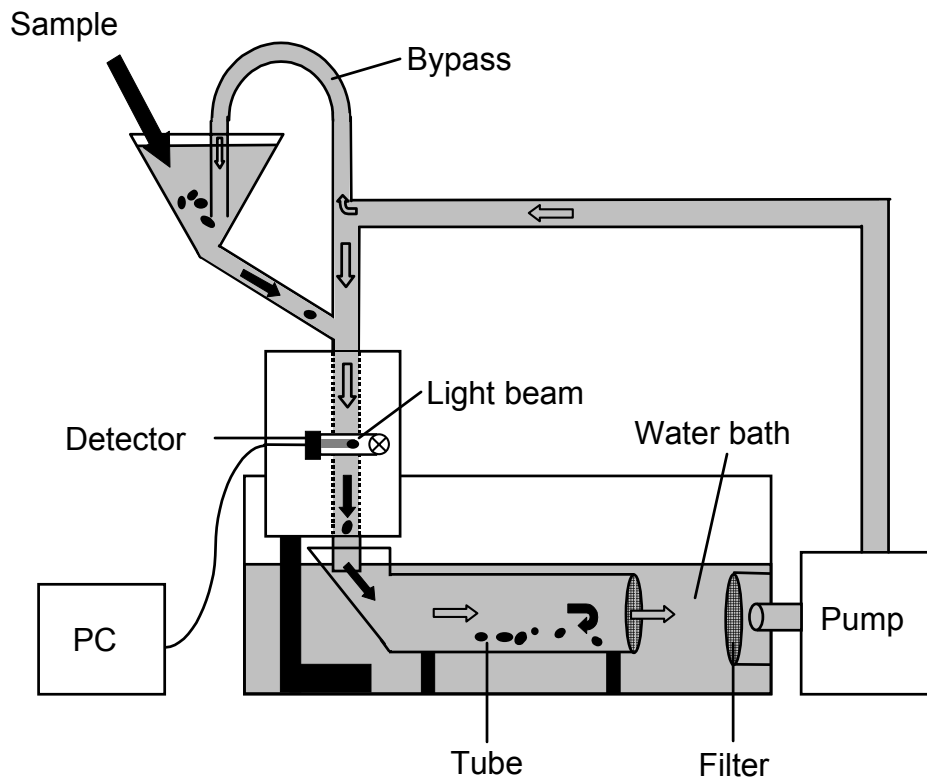
Figure I 1. Schematic drawing of the Optical Plankton Counter bench-top model as used in this study.
