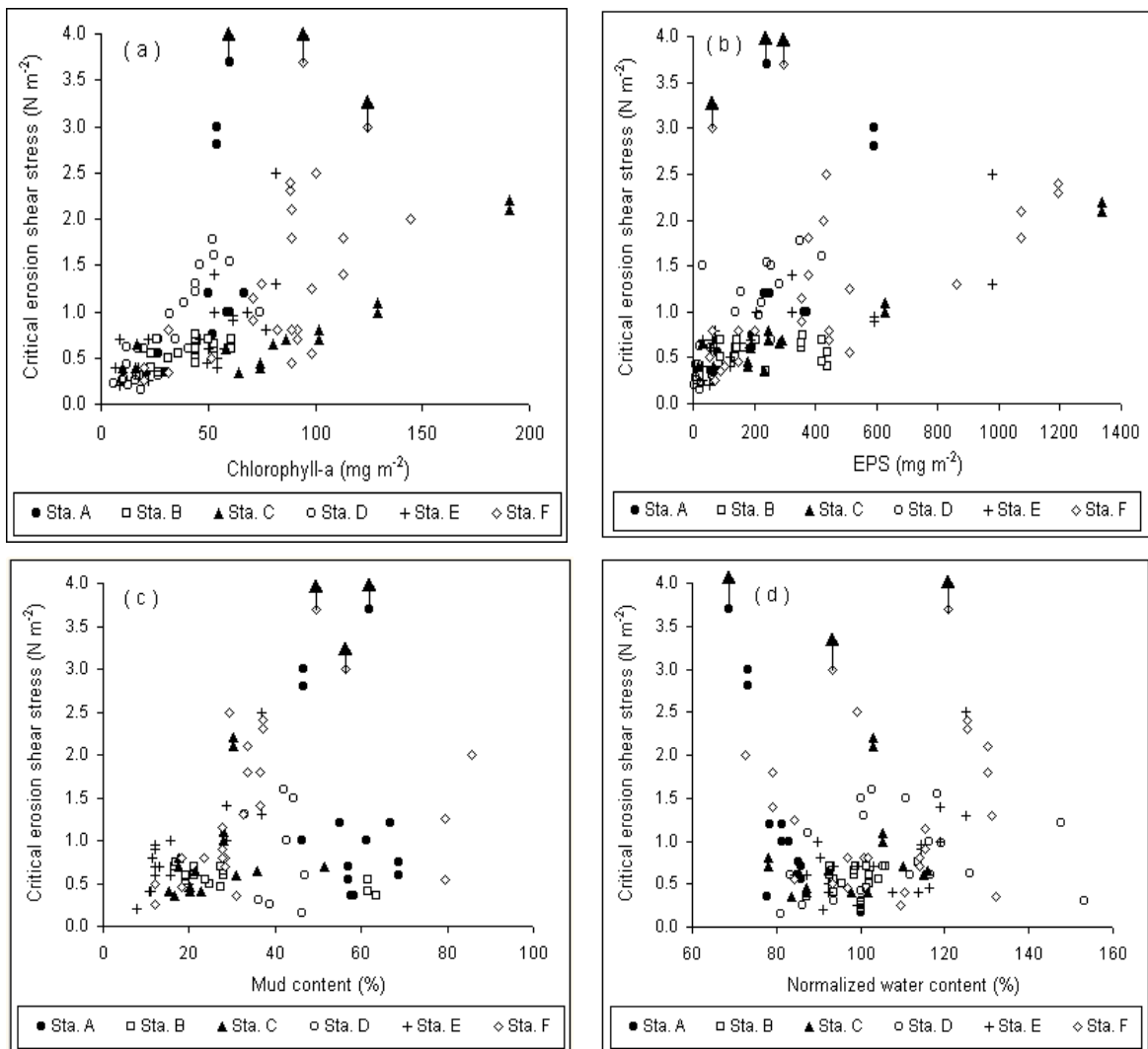
Figure 3.3. Scatter plots of critical erosion shear stress versus (a) chlorophyll-a, (b) EPS, (c) mud content, and (d) normalized water content present in the upper 1mm sediment surface. The data with arrows were omitted in the linear regression analysis because the upper limit of the erosion device was reached.
