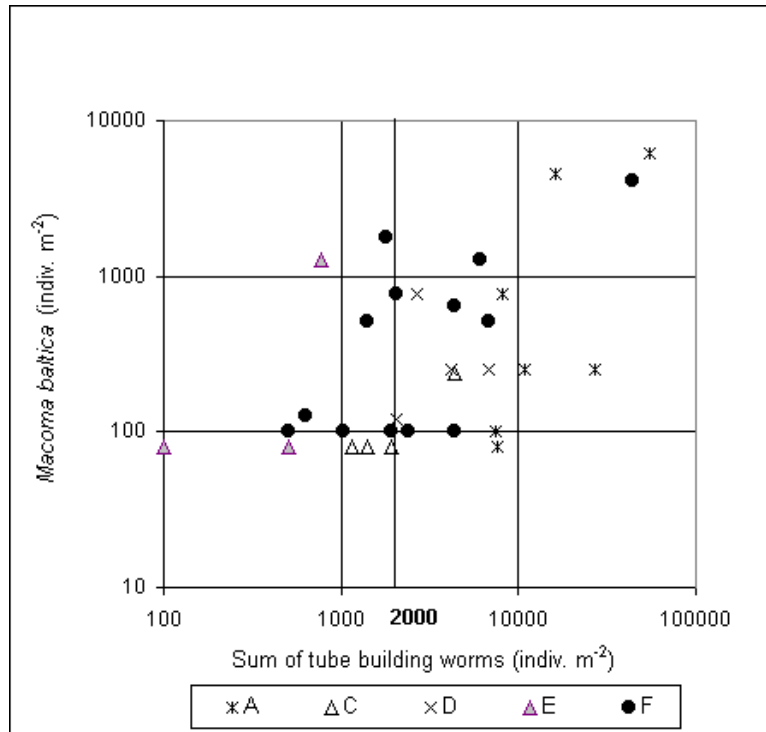
Figure 6.5. Density of Macoma baltica versus the sum of tube building worms. Note that only samples with critical erosion shear stresses higher than 1 \text{ N m}^{-2} and EPS concentrations higher than 400 \text{ mg m}^{-2} were used.
