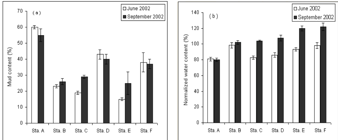
Figure 5.1. Spatial variation of the (a) mud content and (b) normalized water content at stations A - F for June and September 2002 (mean \pm SE, n = 4 - 14).
