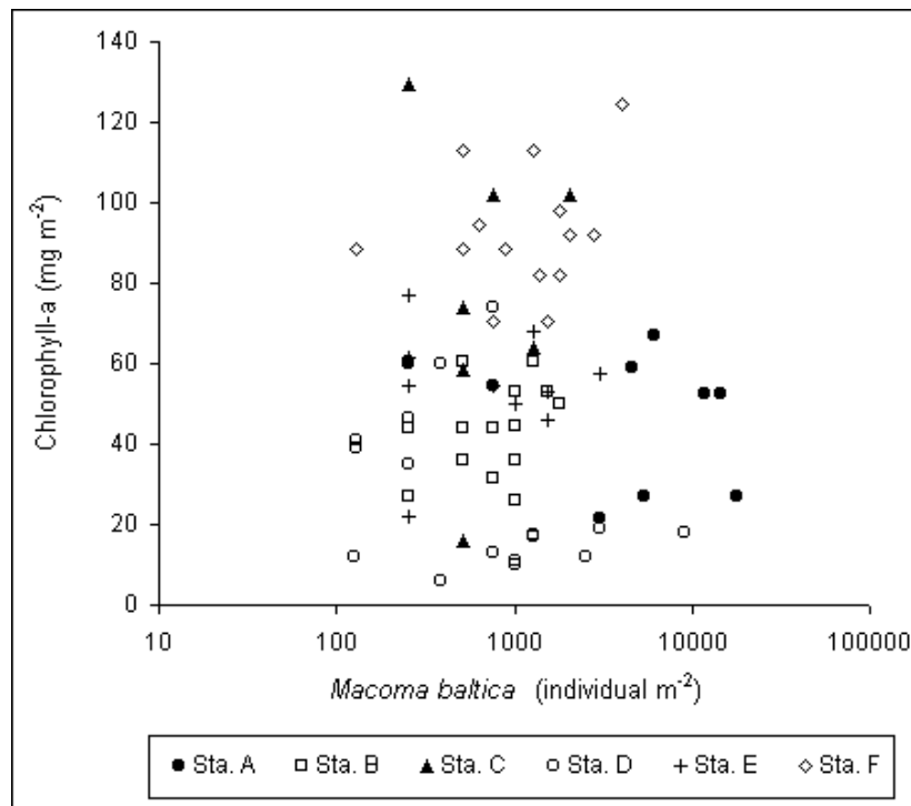
Figure 3.8. Scatter plots of Macoma baltica density versus chlorophyll-a concentration at the study site.
