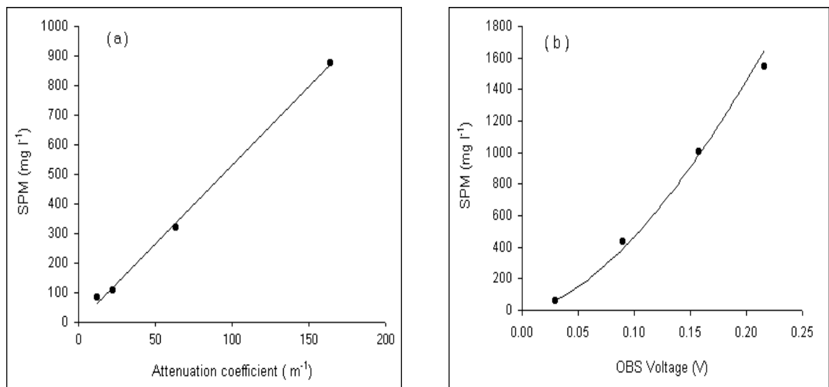
Figure 2.7. Calibration curves for suspended particulate matter (SPM) versus (a) transmission sensor and (b) OBS output.
