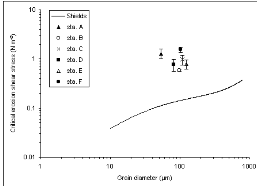
Figure 3.9. Measured critical erosion shear stress in 2002 (mean \pm SE) and compared to \tau_{cr - Shields} of quartz grain in seawater of 10^\circ \text{C} and salinity 35 \text{ }^\circ/\text{oo} (Soulsby and Whitehouse 1997).
