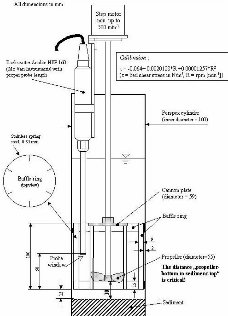
Figure 1.4. Schematic view of EROMES device with backscatter
