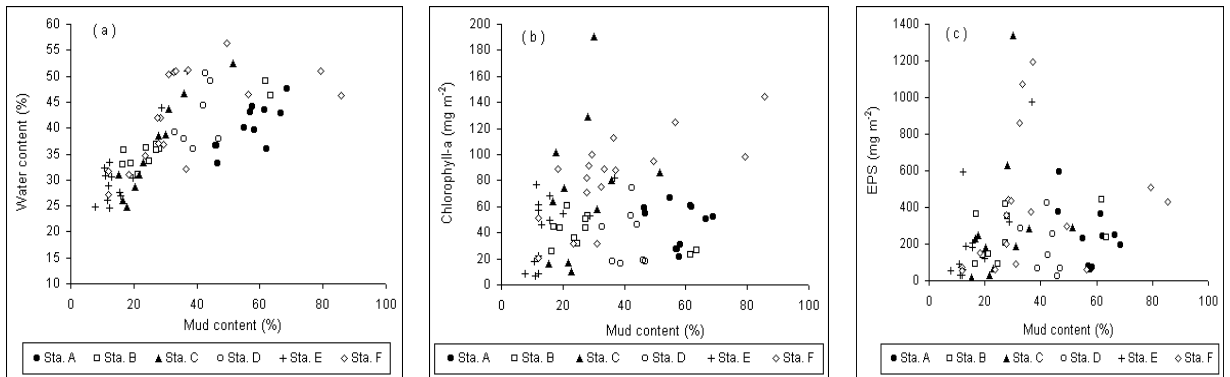
Figure 3.1. Scatter plots of mud content versus (a) water content, (b) chlorophyll-a, and (c) EPS present in the upper 1mm sediment surface.
