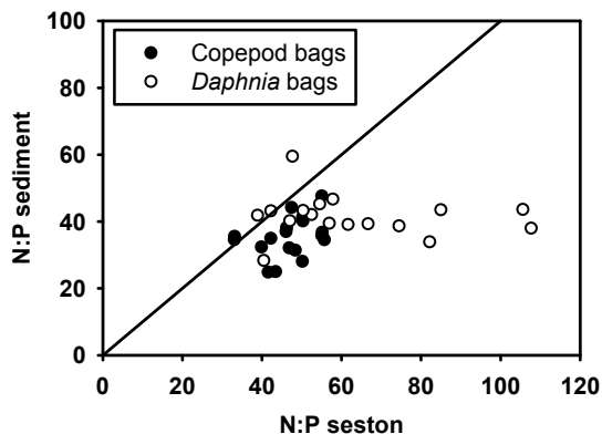
Figure 1-16: N:P ratios (molar) of suspended particulate matter and sediment. Data from day 7 and 13 for seston, and day 8 and 14 for sediment, were grouped. The line of equality is shown.
