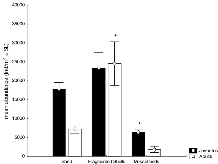
Figure 5. Mean adult abundance of juveniles and adults in three habitats (June and August, 2001. Sites B, C in Fig. 1). * indicates significantly different abundance compared to the other habitats within juveniles and adults (sand n= 6, fragmented shell patches n=6, mussel beds n=6)
