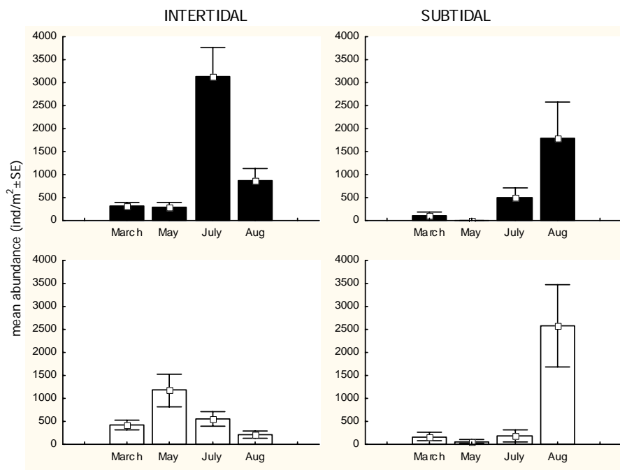
Figure 11. Temporal variability in 2001 of juvenile and adult P. elegans in Königshafen (sites A, B, C, E and D in Fig. 1 respectively) (black bars=juvenile, white bars= adults).
