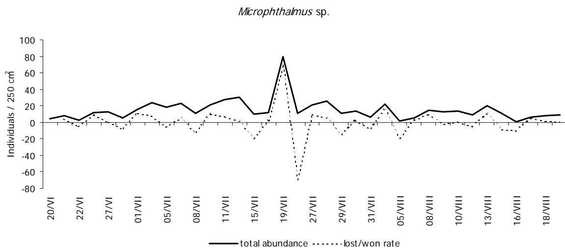
Figure 2. Temporal variability of abundance in juvenile Microphthalmus sp. on a 4 m 2 plot sampled at 25 evenly distributed points. Rate of lost/won individuals is shown as dotted line.
