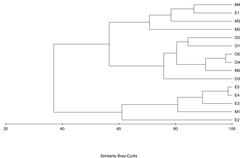
Figure 7. Cluster diagram of species composition analysis for sandy tidal flats in Königshafen, August 2002. (O=Oddewatt, M=Möwenbergwatt, E=Ostfeuerwatt) Index of similarity used: Bray-Curtis.
