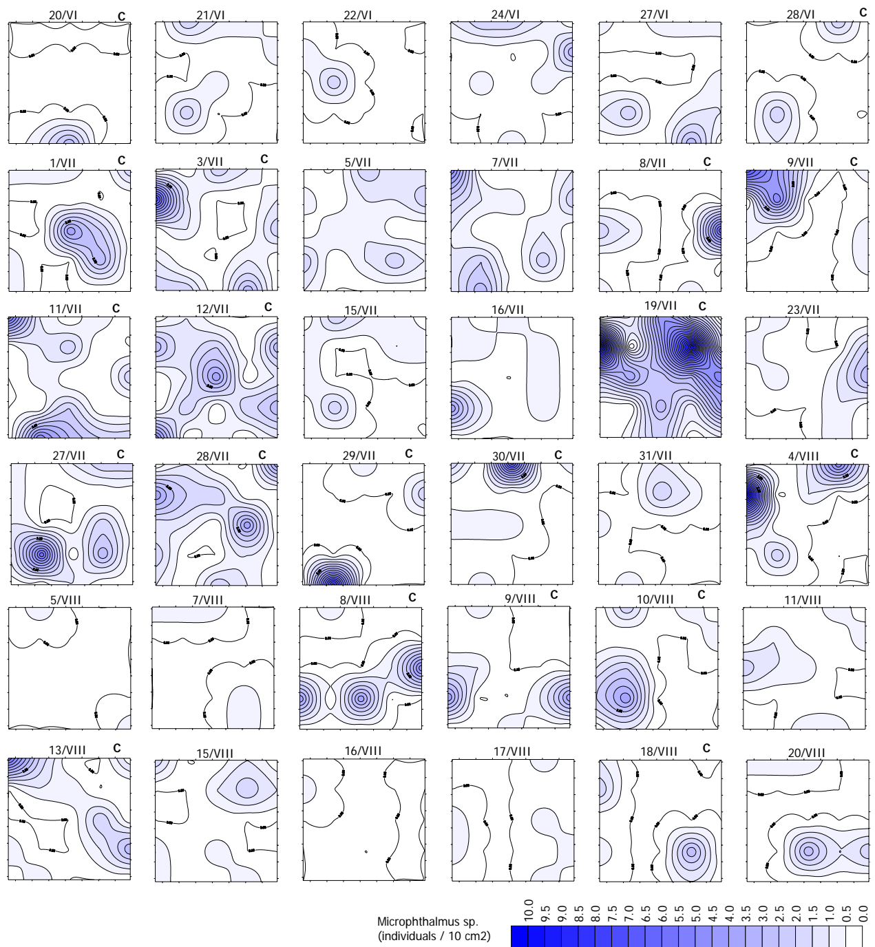
Figure 3. Dispersion of juvenile Microphthalmus sp. on 4 m 2 of a sand flat.
