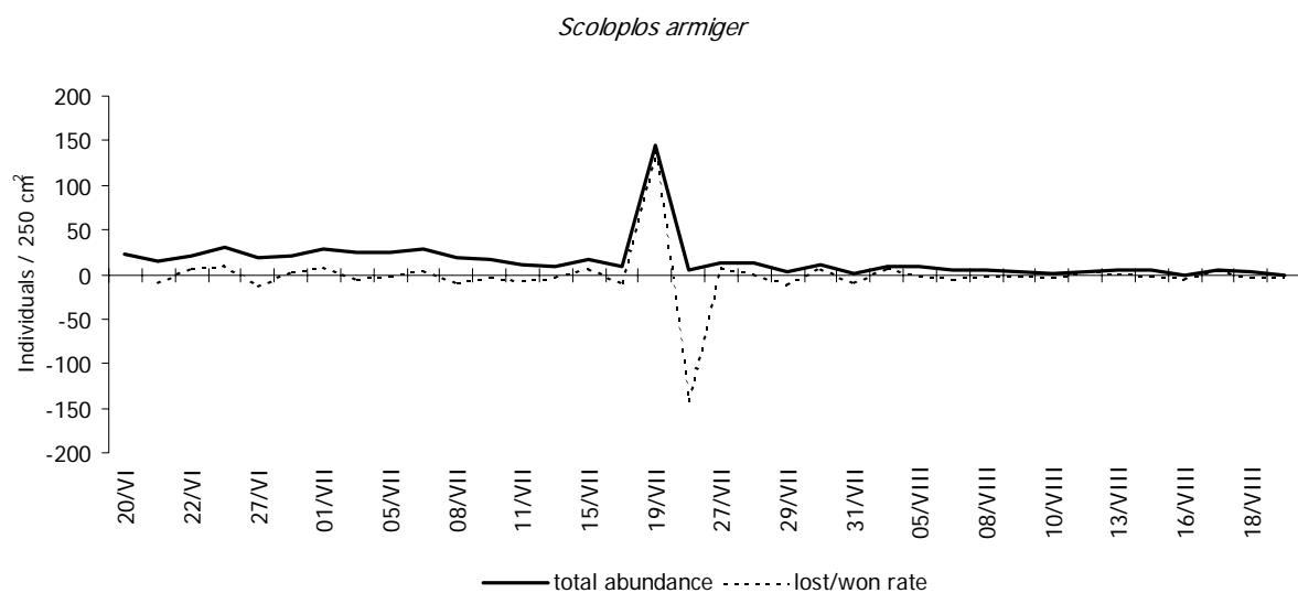
Figure 4. Temporal variability of abundance in juvenile Scoloplos armiger on a 4 m 2 plot sampled at 25 evenly distributed points. Rate of lost/won individuals is shown as dotted line.
