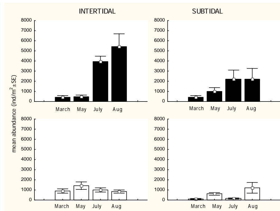
Figure 9. Temporal variability of juvenile and adult Scoloplos armiger in 2001 in Königshafen (sites A, B, C, E and D in Fig. 1 respectively) (black bars=juvenile, white bars= adults).
