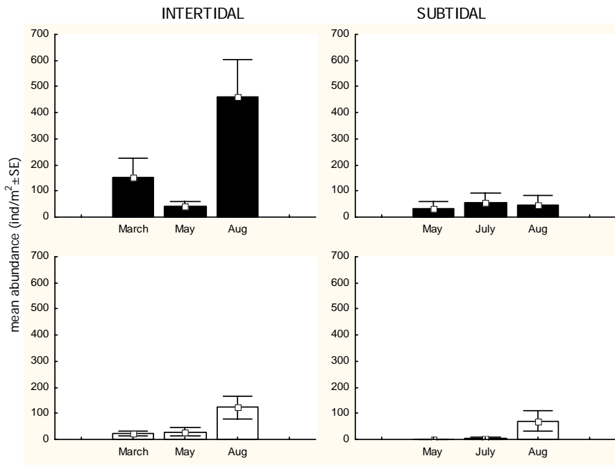
Figure 10. Temporal abundance variability in 2001 of N. virens at inter- and subtidal flats in Königshafen (sites A, B, C, E and D in Fig. 1 respectively) (black bars=juveniles, white bars=adults).
