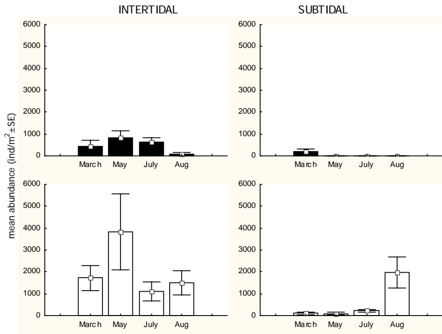
Figure 13. Temporal abundance variation in 2001 of juveniles and adults of Microphthalmus sp. in Königshafen (sites A, B, C, E and D in Fig. 1 respectively) (black bars=juveniles, white bars=adults).
