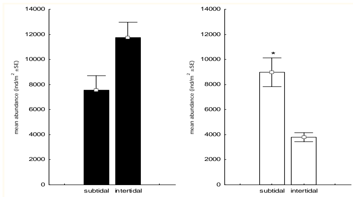
Figure 8. Mean abundance \pm SE of juvenile and adult polychaetes in both sub- and intertidal flats in Königshafen (August, 2001. Sites A, B, C, and D in Fig. 1). Black bars=juveniles, white bars= adults (subtidal n=16, intertidal=32).
