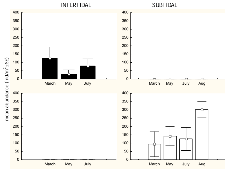
Figure 12. Temporal abundance variation of juvenile and adult O. rathkei in intertidal and subtidal regions around Königshafen (sites A, B, C, E and D in Fig. 1 respectively) (black bars=juveniles, white bars=adults).
