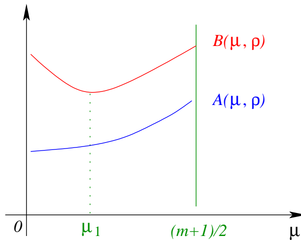
Figure 4.6: Functions A(\mu, \rho) and B(\mu, \rho) in CASE 3.2.1 .
