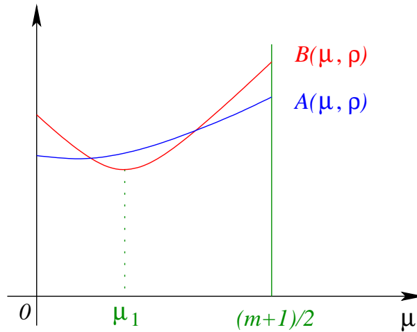
Figure 4.10: Functions A(\mu, \rho) and B(\mu, \rho) in CASE 3.2.3 .
