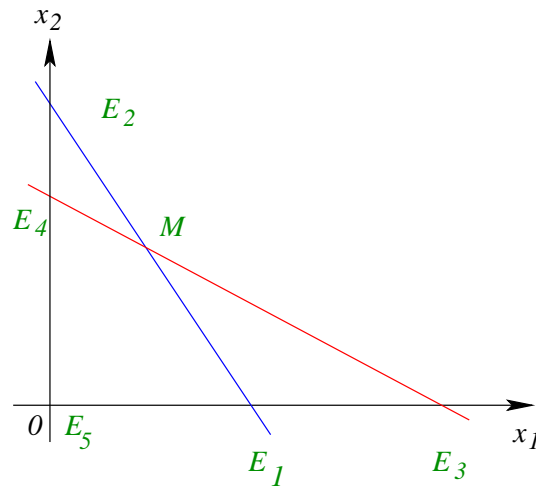
Figure 4.16: Polytope of CASE 2 .
