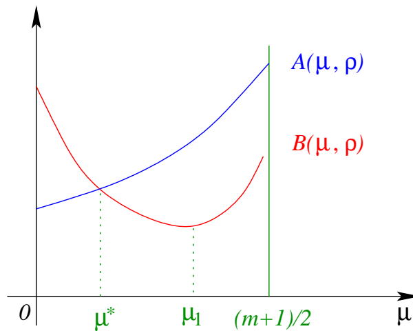
Figure 4.7: Functions A(\mu, \rho) and B(\mu, \rho) in one case of CASE 3.2.2 .
