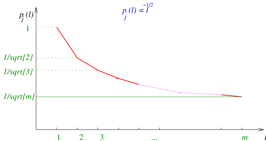
Figure 4.19: An example of our new model (processing time versus number of processors).
