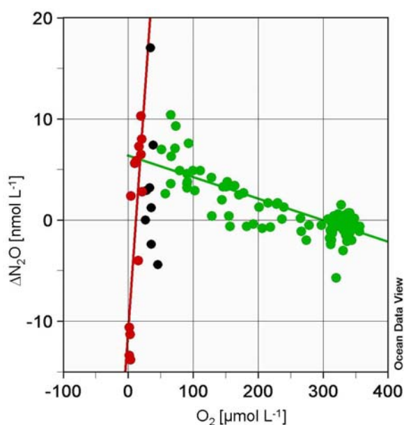
Fig. 8. Correlation between \Delta N_2O and O_2 in the Baltic Sea. Correlations were calculated for oxic waters with O_2 concentrations > 50 \mu\text{mol L}^{-1} (green coloured, y = -0.019x + 5.41 , R^2 = -0.70 ) and < 20 \mu\text{mol L}^{-1} (red coloured, y = 1.038x - 11.36 , R^2 = 0.81 ). These concentrations were empirically tested and gave the best fittings for both correlations.
