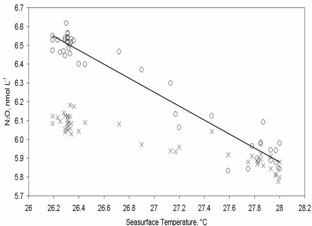
Fig. 3: Correlation ( r^2 = 0.94 , n = 46 ) of SST and N_2O concentration in the equatorial upwelling area ( 0-2^\circ N , 23.5-26^\circ W ). Open circles stand for in-situ measurements and crosses stand for the corresponding equilibrium concentrations calculated as a function of the actual SST, salinity, atmospheric dry mole fraction, and ambient pressure.
