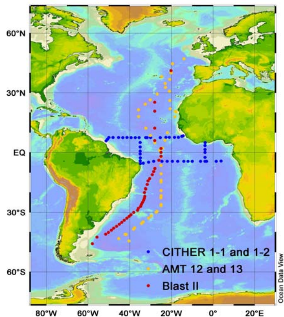
Fig. 4: Recent measurements of vertical N_2O profiles of the last 25 years.
