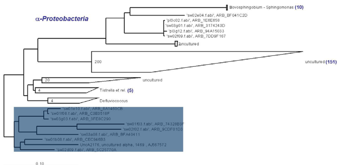
Fig. 7: Phylogenetic tree of 16S rDNA sequences affiliated to \alpha - Proteobacteria exported from ARB (Maximum Parsimony); signatures of sequences obtained during this study start with the letters “sw” and “pl”; the number of sequences in each group is given in parentheses; groups of sequences highlighted in blue were found at station 175; uncoloured groups contain sequences of both stations
