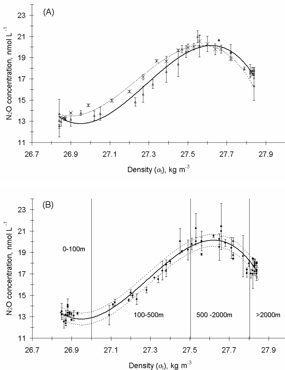
Fig. 2: \text{N}_2\text{O} concentrations vs. density ( \sigma_t ) during EIFEX. (A) Out-stations: Triangles stand for stations 546 and 587 and crosses stand for station 514. The bold solid line represents a 3 rd order polynomial fit based on stations 546 and 587 (see text for statistical details). The thin solid line represents a 3 rd order polynomial fit based on station 514. (B) In-stations: 513, 544, 570, and 580 (symbols) compared with the polynomial fit based on out-stations 546 and 587 (bold line, see panel A). The dashed lines indicate the standard error of the predicted \text{N}_2\text{O} . Depths intervals are indicated.
