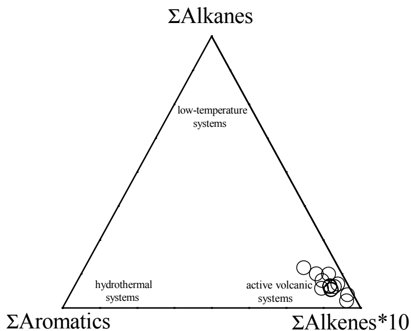
Fig. 6 ΣAlkene*10-ΣAlkanes-ΣAromatics ternary diagram for gas samples from Mombacho volcano. The gas fields for low temperature, hydrothermal and active volcanic systems (Capaccioni et al. 1995) are also reported
