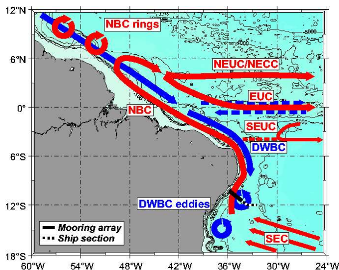
Figure 1.2.: Circulation in the western tropical Atlantic. Schematic representation of mean currents and eddy generation at the western boundary of the tropical Atlantic with warm water pathways in red and North Atlantic Deep Water pathways in blue. Black bar and dotted black line at 11°S indicate positions of the measurement program. Current branches indicated are the South Equatorial Current (SEC), the North Brazil Current (NBC), the South Equatorial Undercurrent (SEUC), the Equatorial Undercurrent (EUC), the North Equatorial Undercurrent (NEUC) merged with the north equatorial counter current (NECC) and the Deep Western Boundary Current (DWBC) with altering zonal flows marked at the Equator. Modified after Dengler et al. (2004).
