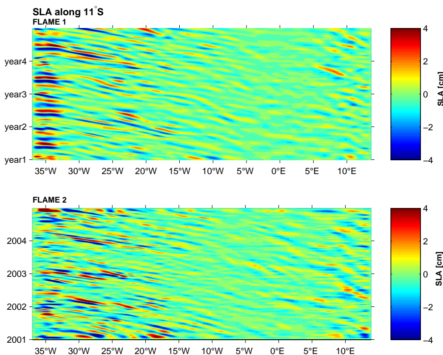
Figure 3.26.: Time-longitude plot of sea level anomalies (SLA) along 11°S for FLAME 1 (upper panel) and FLAME 2 (lower panel). A band-pass filter in time (10-150 d) and space (100-1500 km) is applied.
