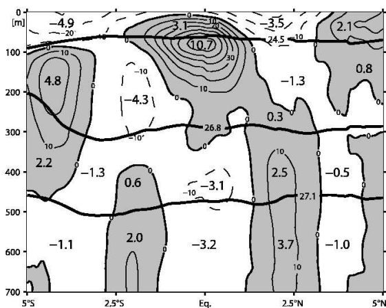
Figure 5.24.: Mean zonal current distribution from 11 section at 26^\circ\text{W} (in \text{cm/s} ), with layer transports (in \text{Sv} = 10^6 \text{ m}^3 \text{ s}^{-1} ) of different current branches overlaid on potential density (thick solid lines). After Brandt et al. (2006).
