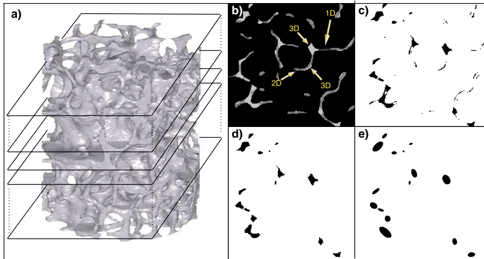
Figure 2.23: From a high resolution scan of a continuous network to a set of point process realisations and related measures: a) binarised volume, b) voxel set classified into one, two and three-dimensional types, c) projection to 3D elements, d) opening of the dataset to exclude small groups of voxels not belonging to a junction, e) fitted ellipsoids mark the locations of junctions and thus form a (marked) point process, from which measures like J and K -functions can be calculated. A stack of slice based realisations is retrieved by repeating b)-e) for different slices.
