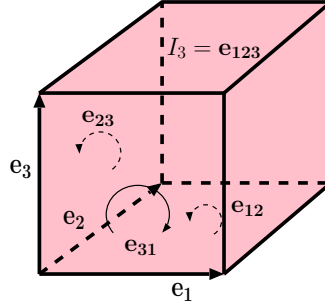
Fig. 2.4: Basis elements of \mathbb{R}_3 .
