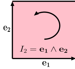
Fig. 2.2: Basis vectors e_1, e_2 and the unit pseudoscalar I_2 = e_{12} .
