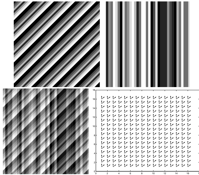
Fig. 4.4: Top row: two i1D patterns with different orientations. Bottom row: the i2D pattern superimposed by the two i1D patterns and the sampled orientation estimation by using the novel 2D rotationally invariant quadrature filter.
