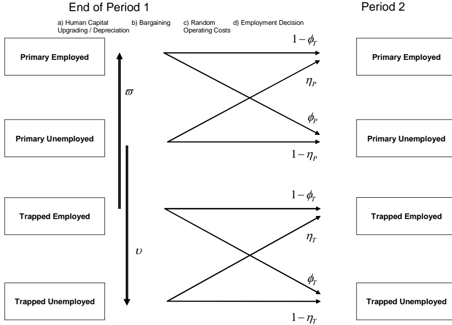
Figure 22: Transition probabilities
