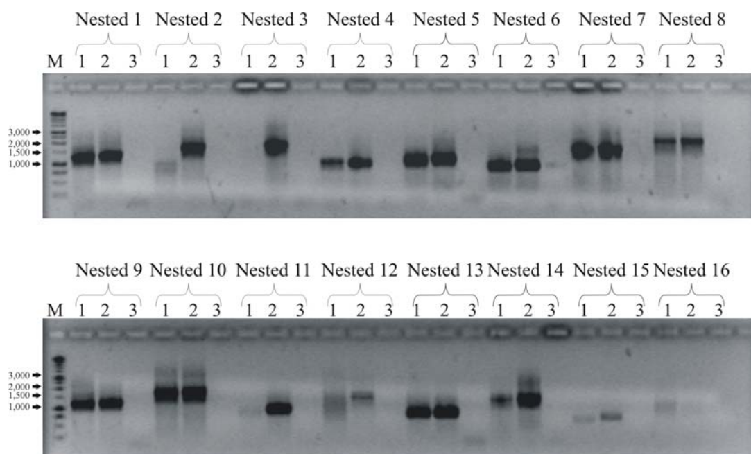
Figure II-3: amoCAB nested PCR amplification of Nitrosomonas europaea ATCC 19718 and Baltic Sea sediment with different primer combinations using amoC58f-amoB1179r PCR fragment. M = 1 kb Ladder; 1 = Baltic Sea sediment; 2 = Nitrosomonas europaea ATCC 19718; 3 = Blank.
