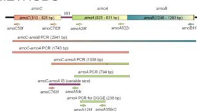
Fig. 3. New PCR reactions designed for amplifying the amoCAB operon
