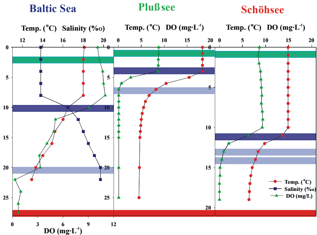
Figure III-1: Depth profiles taken at the Baltic Sea, Plußsee and Schöhsee in September 2004. Temperature (●), dissolved oxygen (▲), and salinity in the Baltic Sea (■). Samples for community analysis were taken from different depths: in the Baltic Sea from 2, 10 and 20 m; in Plußsee from 1, 4 and 7 m; in Schöhsee from 1, 11, 12, and 14 and. Samples from the sediment were taken from 27.5 (Baltic Sea), 28 (Plußsee) and 22 m (Schöhsee).
