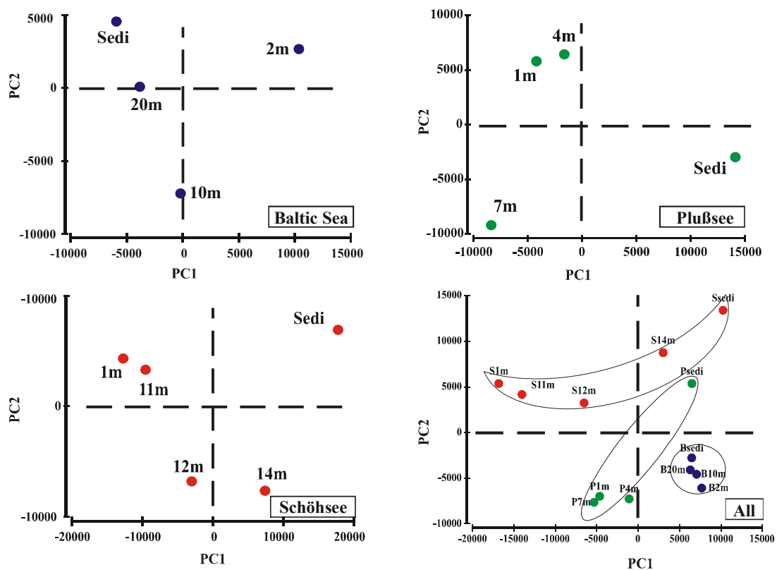
Figure V-4: Principal component analysis (PCA) of T-RFLP patterns after restriction with 5 enzymes. Samples are coded as follows: Baltic Sea, blue; Plußsee, green; Schöhsee, red.
