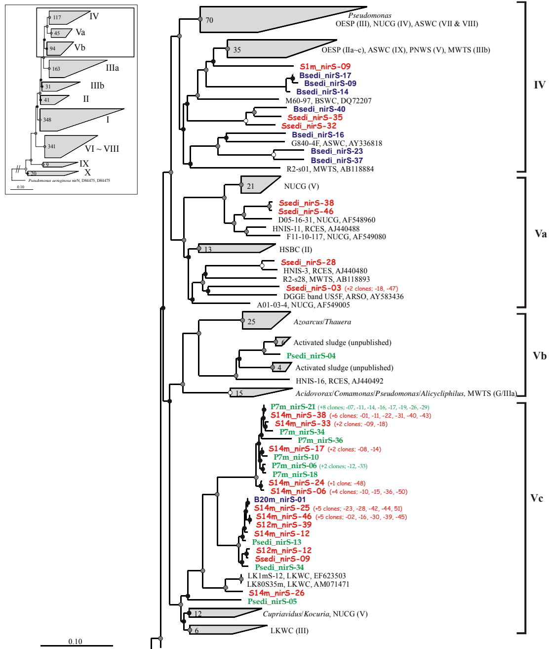
Figure V-5: Phylogenetic tree of nirS gene, based on 142 deduced amino acid sites, constructed by neighbor joining method in ARB with nirN from Pseudomonas aeruginosa (D84475) as the outgroup. For explanation see Fig. V-4.
