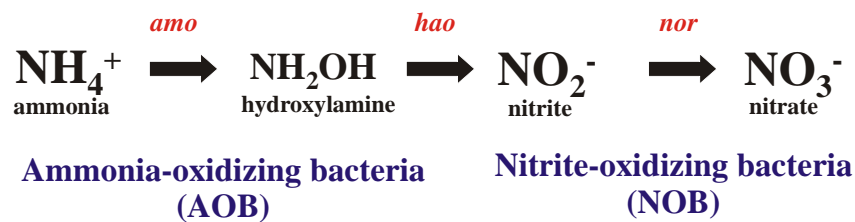
Figure 1- 2: Nitrification process
