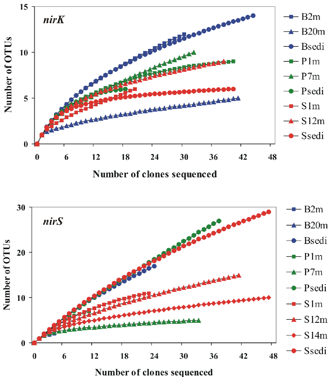
Figure V-6: Rarefaction curves indicating nirK and nirS diversity in clone libraries derived from each environment. OTUs were defined as groups of sequences differing by \leq 5\% at the DNA level. Coding of the samples with three different colors: blue=Baltic Sea; green=Plußsee; red=Schöhsee.
