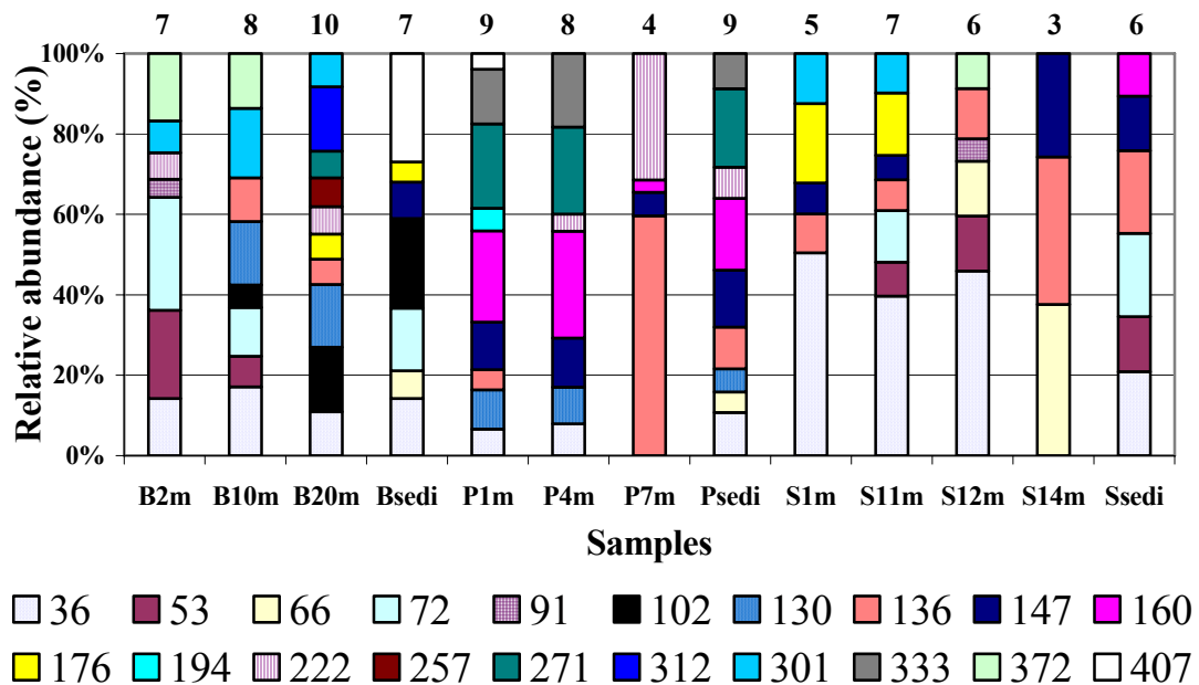
Figure VI-2: Relative abundance of T-RFs after restriction with Hae III of amplified nirS in samples from the Baltic Sea, Plußsee and Schöhsee. Number in upper of the columns indicated the number of T-RFs detected in each sample. Numbers in bottom indicate the lengths of T-RFs in base pair.
