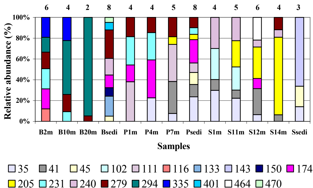
Figure VI-1: Relative abundance of T-RFs after restriction with Hae III of amplified nirK in samples from the Baltic Sea, Plußsee and Schöhsee. Number in upper of the columns indicated the number of T-RFs detected in each sample. Numbers in bottom indicate the lengths of T-RFs in base pair.
