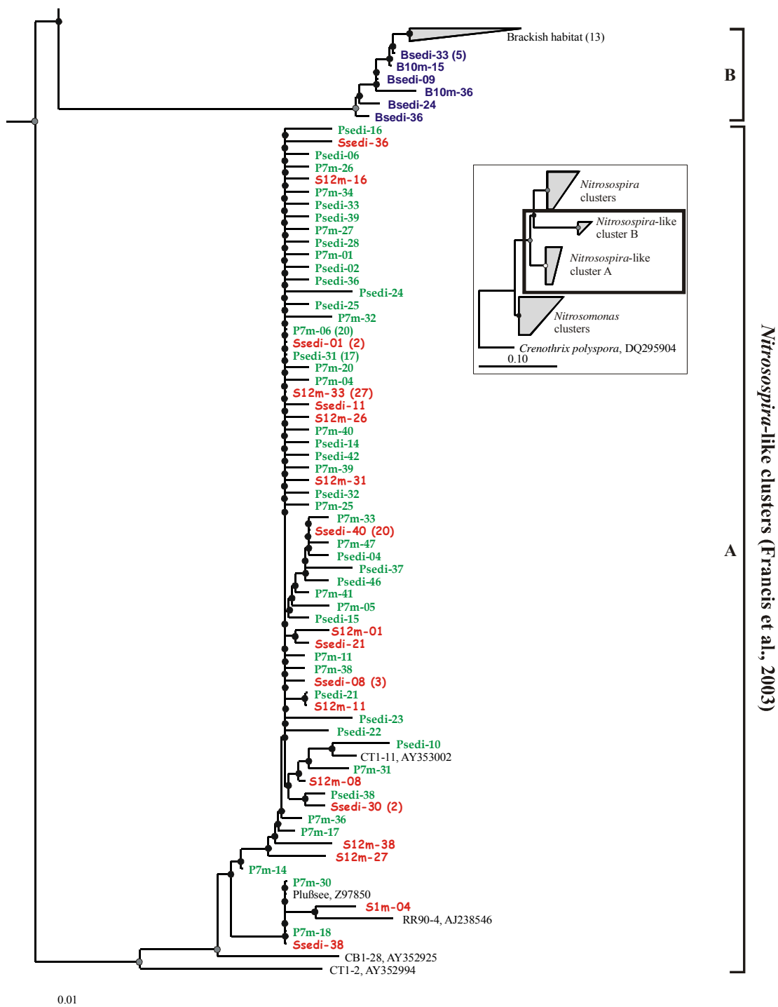
Figure IV-3: Fitch-Margoliash phylogenetic tree calculated in ARB with 263 amino acids of AmoA using PmoA from Crenothrix polyspora (Acc. No. DQ295904) as an outgroup. Nomenclature of clusters according to (Purkhold et al., 2003) and (Francis et al., 2003). Clones from this study are in bold, with the number of identical clones in brackets, and their origin coded with three different letter types: Arial for Baltic Sea with blue, Book Antiqua for Plußsee with green, and Comic Sans MS for Schöhsee with red. Bootstrap values for \geq 90 replicate trees are indicated at the nodes with three different colors: black (100%), gray (95 - 99%) and white (90 - 94%).
