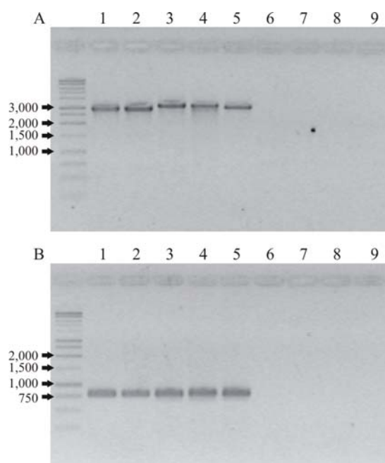
Figure II-2: Agarose gel electrophoresis of PCR products from amoCAB (approximately 3,000-bp) (A) and of 789-bp fragments of the amoA (789-bp) (B) from ammonia-oxidizing bacteria and methane-oxidizing bacteria. Lane 1: Nitrosomonas europaea ATCC 19718; lane 2: Nitrosomonas eutropha ; lane 3: Nitrospira briensis ; lane 4: Nitrosovibrio tenuis ; lane 5: Nitrosomonas sp. L13; lane 6: Nitrosococcus oceani ATCC 19707; lane 7: Methylococcus capsulatus ; lane 8: Methylocystis parvus ; lane 9: Blank.
