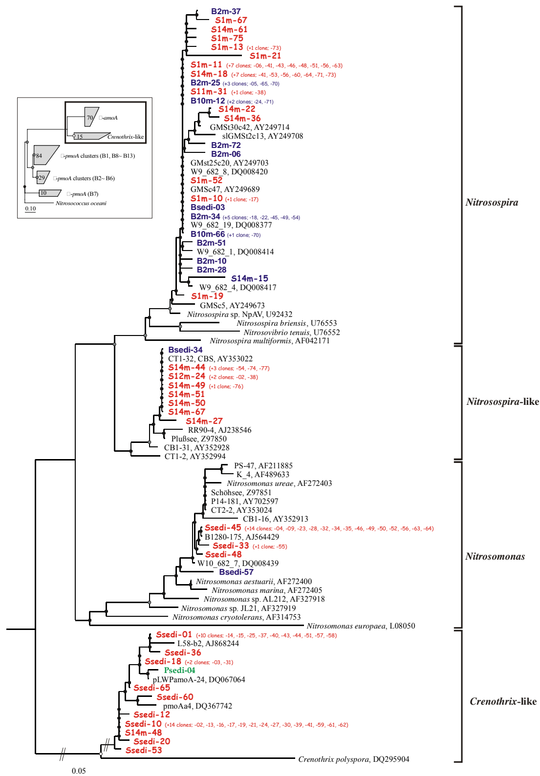
Figure V-2: Phylogenetic tree calculated with 177 amino acids of AmoA and PmoA using Fitch Margoliash method in ARB. Nomenclature of clusters follows (Francis et al., 2003) for amoA and (Pester et al., 2004) and (Bussmann et al., 2006) for pmoA . Clones from this study are in bold and typed with three different fonts: Arial for Baltic Sea with blue , Book Antiqua for Plußsee with green and Comic Sans MS for Schöhsee with red . Bootstrap values \geq 90 replicate trees are indicated at the branch with three different colors: black (100%), gray (95 - 99%) and white (90 - 94%).
