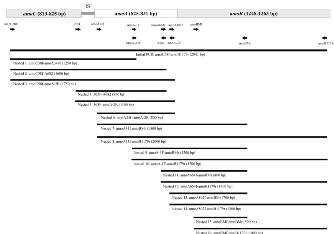
Figure II-1: Structure of amoCAB operon in \beta -AOB including intergenic space (IS) between amoC and amoA and designed PCR for this study. Initial PCR and 16 nested PCRs are described. The expected length of fragments is given in parenthesis.
