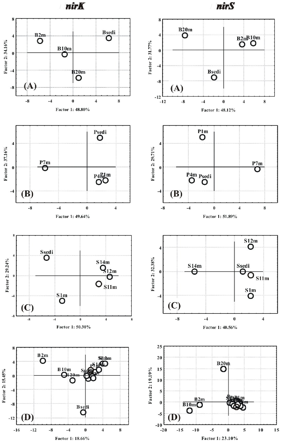
Figure VI-3: Principal component analysis of T-RFLP of nirK (left) and nirS (right) from samples of the Baltic Sea (A), Plußsee (B), Schöhsee (C) and all samples (D).
