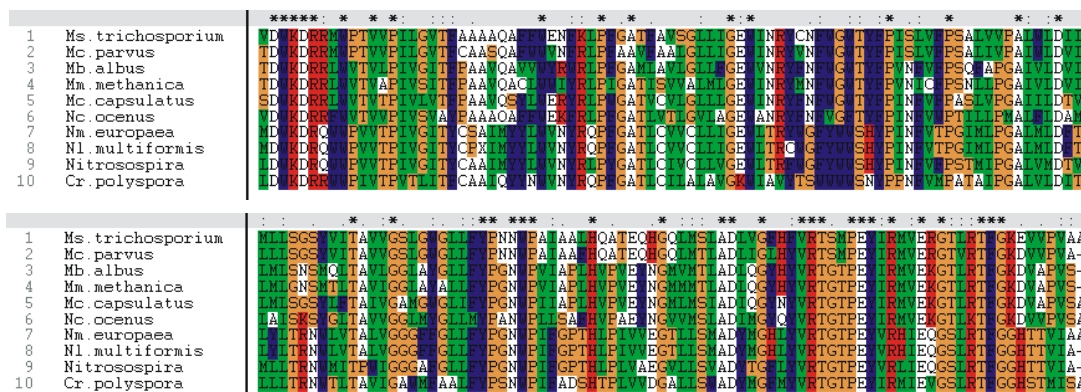
Figure 1- 3: Alignment of predicted amino acid sequences of amoA and pmoA genes from ammonia-oxidizing bacteria, methane-oxidizing bacteria and Crenothrix polyspora .
