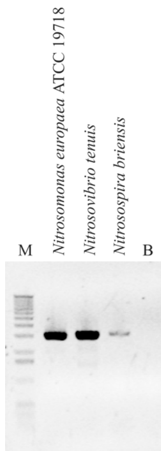
Figure I-4. Agarose gel electrophoresis of PCR products amplified with the primers amoC58f-amoB1179r from genomic DNA of recognized AOB species (A) and environmental samples (B). M= 1 Kb ladder; B=Negative control.
