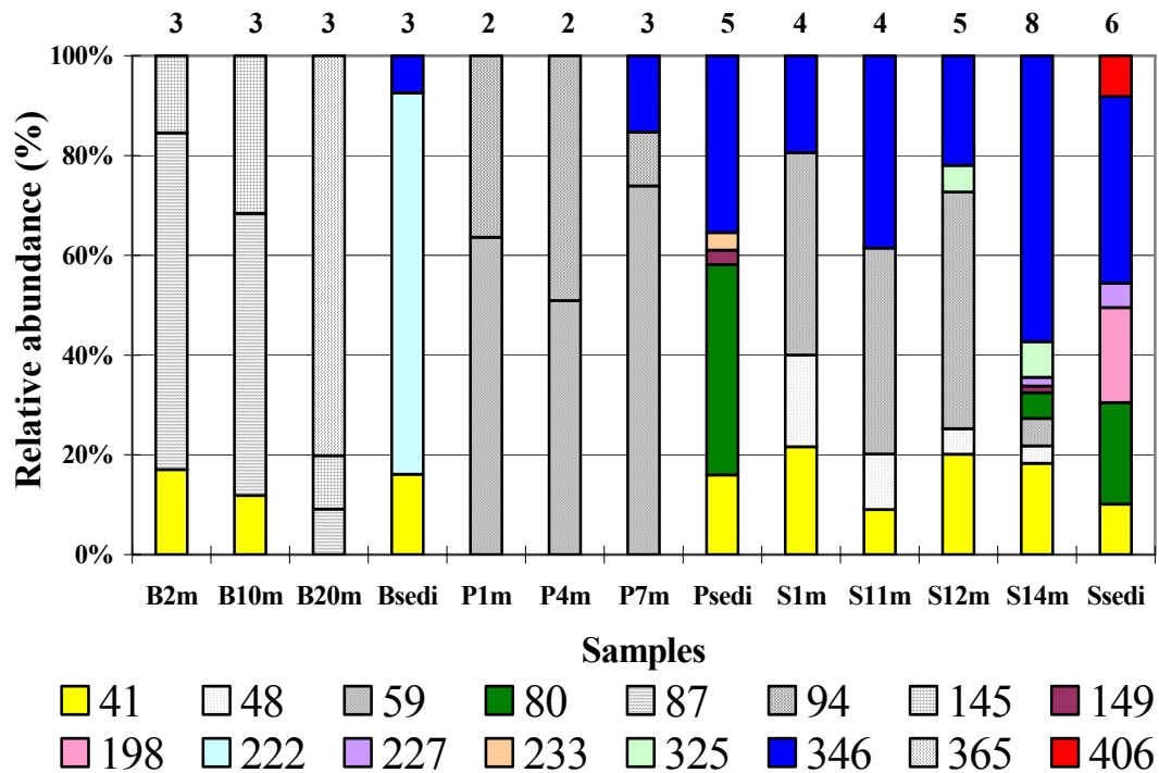
Figure V-3: Relative abundance of T-RFs after restriction with HaeIII . Number in upper of the columns indicated the number of T-RFs detected in each sample. Length of the different fractions is coded according to the panel on the bottom. For the colored T-RFs a corresponding clones was identified in the clone libraries by simulated.
