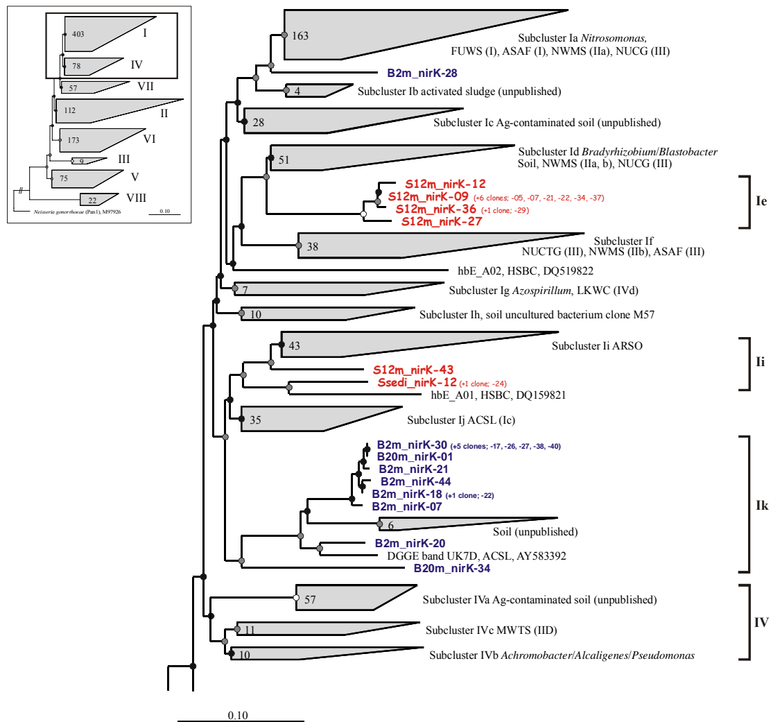
Figure VI-4: Phylogenetic tree of nirK gene, based on 158 deduced amino acids, constructed by neighbor joining method in ARB with aniA from Neisseria gonorrhoeae (M97926) as the outgroup. Clones from this study are shown in bold and designated as B , Baltic Sea in Arial with blue; P , Plußsee in Book Antiqua with green; S , Schöhsee in Comic Sans MS with red. and followed by depth. Sedi=sample from sediment-water interface. Bootstrap values for 1,000 replicates are indicated at the branch points by circles: black (100%), gray (95 - 99%) and white (90 - 94%). PNWS, Pacific Northwest sediment (Braker et al., 2000); RCES, River Colne estuary sediment (Nogales et al., 2002); FUWS, forested upland and wetland soil (Priemé et al., 2002); SDAC, incubated soil with different ammonia concentration (Avrahami et al., 2002); NWMS, northwestern Mexico sediment (Liu et al., 2003); NUCC, nitrate- and uranium-contaminated groundwater (Yan et al., 2003); BSCB, Baltic Sea cyanobacterial bloom (Tuomainen et al., 2003); MWTS, metallurgic wastewater treatment systems (Yoshie et al., 2004); ASAF, arable soil receiving artificial fertilizer (Wolsing and Priemé, 2004); ASWC, Arabian Sea water column (Jayakumar et al., 2004); ARSO (arable soil), ACSL (activated sludge) and PESO (peat soil) (Throbäck et al., 2004); OESP, OMZ in the eastern South Pacific (Castro-González et al., 2005); HSBC, Huntington State Beach, California (Santoro et al., 2006); BSWC, Baltic Sea water column (Hannig et al., 2006); AGCS, Ag-contaminated soil (unpublished); LKWC, Lake Kinneret water column (Junier et al. submitted)
