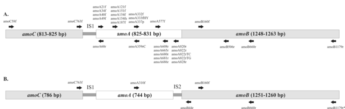
Figure I-1: Schematic diagram of the amoCAB operon in beta- (A) and gamma-AOB (B). IS= intergenic regions. The position and orientation of the different primers are shown by arrows. For primer designation see Tab. 1.
