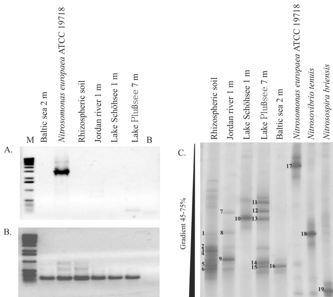
Figure I-5: Evaluation of the nested PCR approach and the DGGE for analyzing AOB in environmental samples. A. PCR with the primers amoC58f-amoB1179r directly from DNA. B. Nested PCR with the primers amoA121fgc-amoA359rC from the products shown in A. C. DGGE profiles of PCR amplicons obtained with the primers amoA121fgc-amoA359rC from environmental samples and Nitrosomonas europaea shown in B. Amplicons from Nitrosospira briensis and Nitrosovibrio tenuis were included in the DGGE. M= 1 Kb ladder; B=Negative control.
