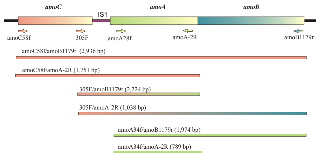
Figure IV-1: Structure of the amoCAB operon and position of the primers used in this study. Initial PCR amplification with 6 different primer pairs was used as templates for nested amoA amplification. Predicted size of the PCR-products in parenthesis.
