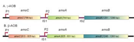
Fig. 1. The amoCAB operon in ammonia-oxidizing bacteria
