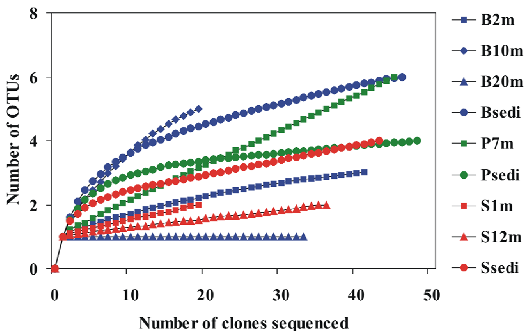
Figure IV-2: Rarefaction curves of amoA -based OTUs at 5% cutoff. Coding of the samples with three different colors: blue=Baltic Sea; green=Plußsee; red=Schöhsee.
