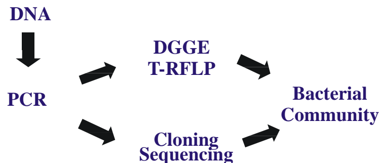
Figure 1- 5: Simplified scheme of molecular methods for studying bacterial communities.
