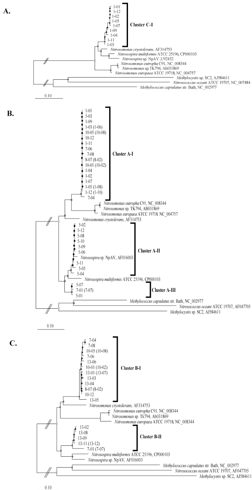
Figure II-4: Phylogenetic tree based on AmoC (A), AmoA (B) and AmoB (C) sequences. Phylogenies were constructed with the PHYLIP subroutine by Fitch-Margoliash in ARB using Amo from Nitrosococcus oceani and Pmo from Methylococcus capsulatus and Methylocystis as outgroups. Clones in this study are shown in bold. Bootstrap values \geq 90\% (100 replicates) are indicated at the branch points in two different colors: black (100%), gray (95 - 99%) and white (90 - 95%).
