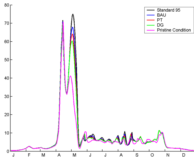
Figure 3.14: Modelled time-series of chlorophyll-a ( \text{mg chl m}^{-3} ) related to input box 78 for different scenarios (BAU, PT, DG) compared to the standard run 1995 and the pristine conditions (Hofmann et al., 2005).
