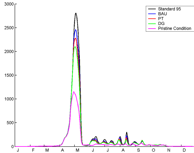
Figure 3.15: Modelled time-series of flagellate concentration ( \text{mg C m}^{-3} ) related to input box 78 for different scenarios (BAU, PT, DG) compared to the standard run 1995 and the pristine conditions (Hofmann et al., 2005).
