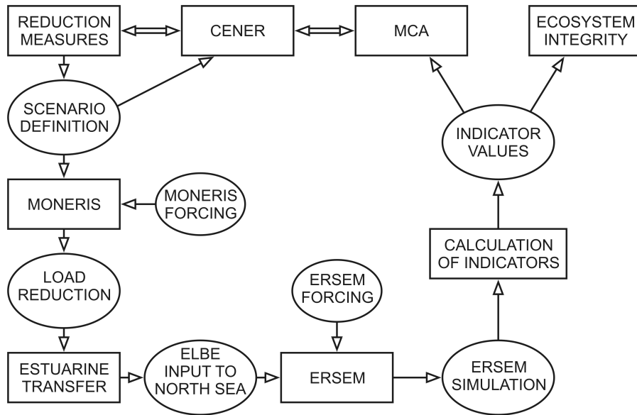
Figure 3.6: Model integration and information exchange (Hofmann et al., 2005).
