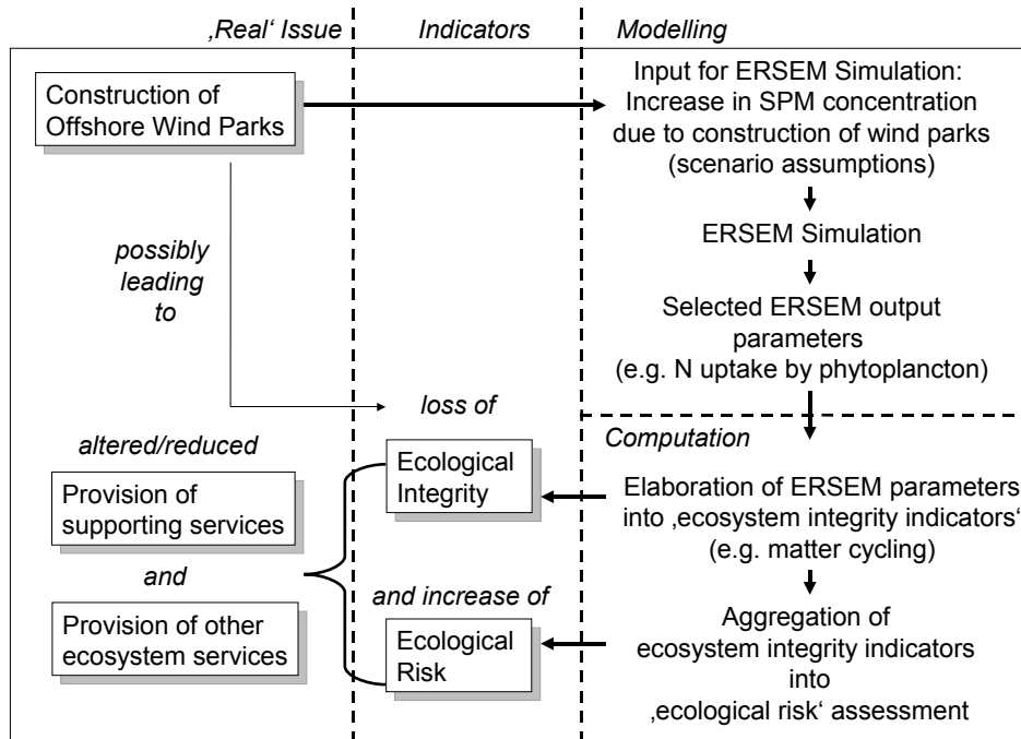
Figure 3.30: Role of modelling for assessing ecosystem functioning by selected indicators. Observable issues (left) are translated into scenarios and enter the model in the form of assumptions (e.g. increased SPM concentrations). The ERSEM simulation (right upper side) provides output parameters that can be used for computing integrity indicators (right lower side) and ultimately assessing ecological integrity and ecological risk (middle).
