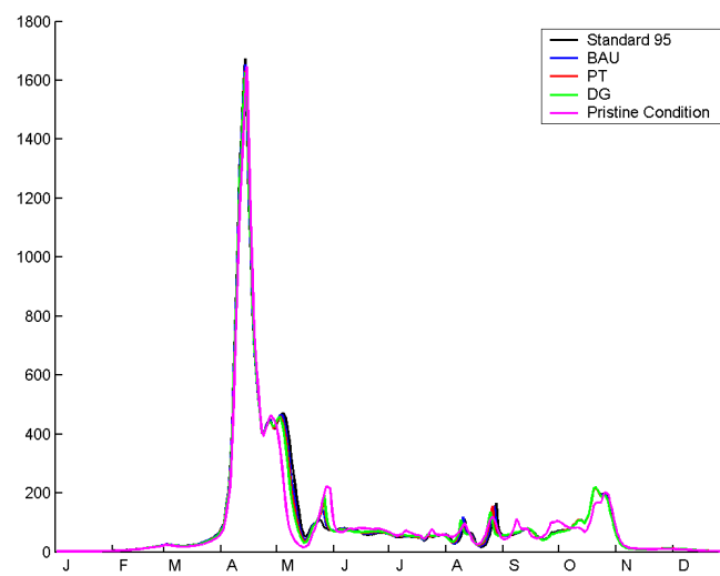
Figure 3.16: Modelled time-series of diatom concentration ( \text{mg C m}^{-3} ) related to input box 78 for different scenarios (BAU, PT, DG) compared to the standard run 1995 and the pristine conditions (Hofmann et al., 2005).
