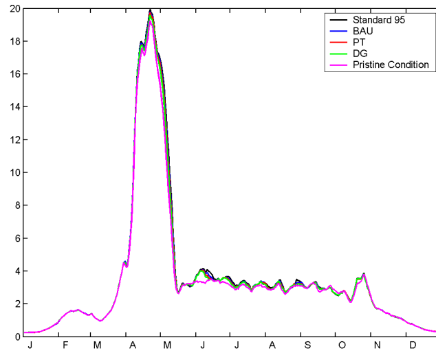
Figure 3.13: Modelled time-series of chlorophyll-a ( \text{mg chl m}^{-3} ) related to the aggregated Elbe box for different scenarios (BAU, PT, DG) compared to the standard run 1995 and the pristine conditions (Hofmann et al., 2005).
