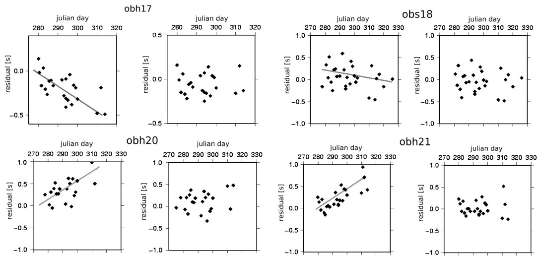
Figure 4.2: Residuals between observed first arrival travel times and synthetic travel times (final calculation with fmtomo ) over duration of deployment. For all plotted stations a linear trend (grey line) was observed (left plot). After a removal of the linear drift, a new calculation with fmtomo was carried out (right plot).
