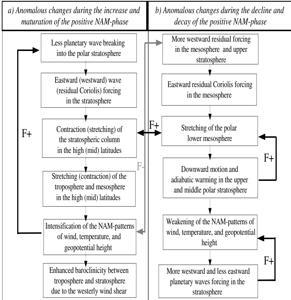
Figure 6.1: Schematic diagram showing the mechanisms that contribute to (a) the strengthening and (b) the weakening of the positive anomalies of the stratospheric polar jet and its impact on the tropospheric circulation during the evolution of the strong positive stratospheric NAM-phase. F+ ( F- ) represents positive (negative) feedback.
