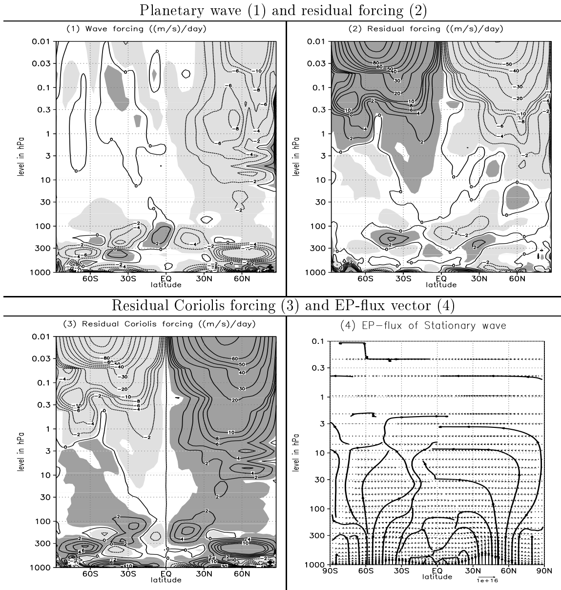
Figure 2.4: The January climatology of (1) planetary wave forcing, (2) residual forcing, and (3) residual Coriolis forcing in MAECHAM5. The forcing interval is 10 (m/s)/day for values above (below) 10 (-10) (m/s)/day, and 2 (m/s)/day for values between -10 and 10 (m/s)/day. Light (dark) shading indicates values less (greater) than -0.5 ( +0.5 ) (m/s)/day. (4) shows the EP-flux vector in both stream and vector representations.
