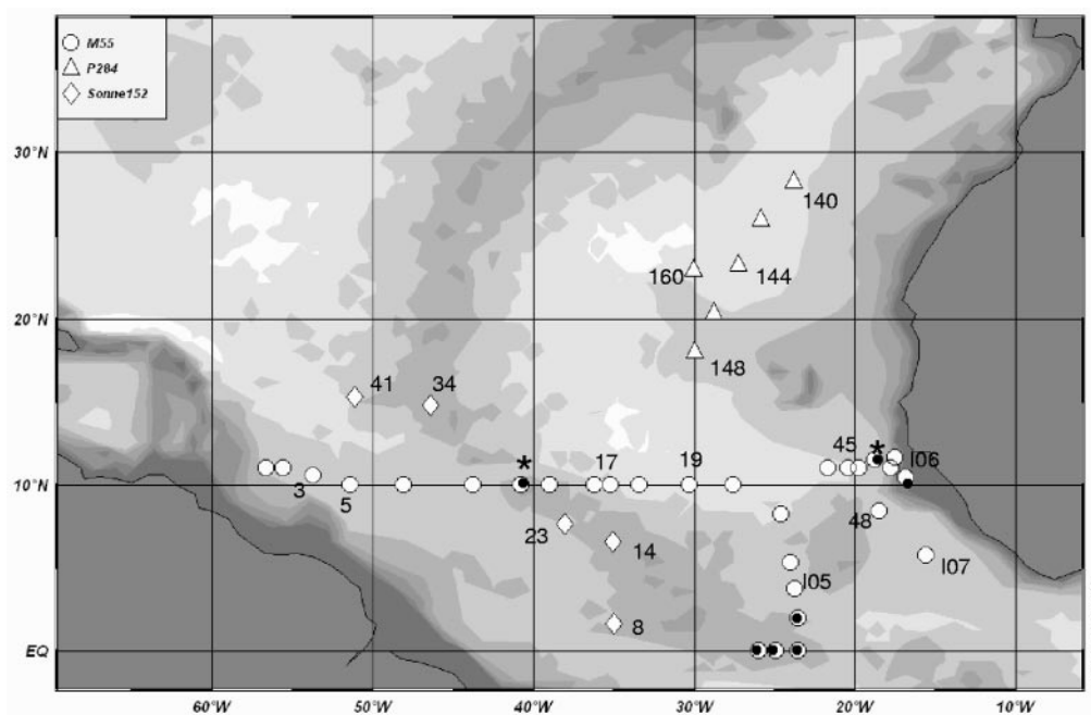
FIG. 1. Cruise tracks and stations analyzed. Stations which produced a negative nifH signal are indicated by a black circle within the station mark. Surface samples for stations marked with * were unavailable for analysis and deepwater samples were negative. The numbered stations indicate stations from which the nifH amplicons were cloned and sequenced, and the numbers correspond to those listed in Table 2 and Fig. 2.
