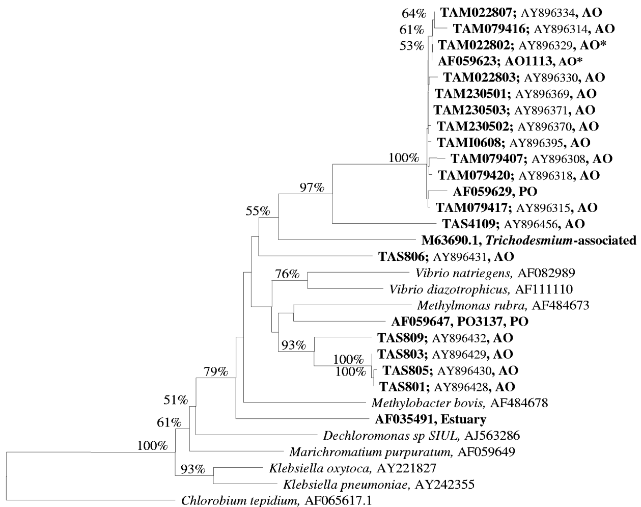
FIG. 6. Phylogenetic relationships between \gamma -proteobacteria nifH nucleotide sequences. Sequence names in boldface type indicate environmental sequences and are marked according to recovery from the Pacific Ocean (PO) or the Atlantic Ocean (AO). Sequence names beginning with "TA" were obtained in this study. AY896329 and AF059623, indicated by asterisks, represent several sequences which were identical. The tree was bootstrapped 1,000 times, and values over 50% are shown.
