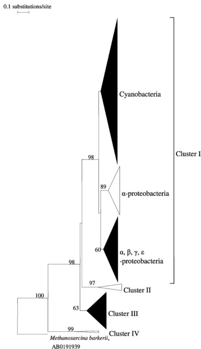
FIG. 3. Phylogenetic tree of global NifH protein sequences. To better visualize the relationship between the groups and clades with significant bootstrap values (>60) were shown. Sizes of the triangles reflect the number of sequences in that clade. Clades that contained sequences from our study are shown in black. Cluster I includes cyanobacteria, \alpha -proteobacteria, \beta -proteobacteria, \gamma -proteobacteria, and \epsilon -proteobacteria. Cluster II consists of \delta -proteobacteria, spirochaetes, and members of the Archaea . Members of the Firmicutes , Spirochaeta , \delta -proteobacteria, chlorobi, and Archaea comprise cluster III. Cluster IV is formed by archaeal sequences. The tree was bootstrapped 100 times with Methanosarcina barkerii AB0191939 as the outgroup.
