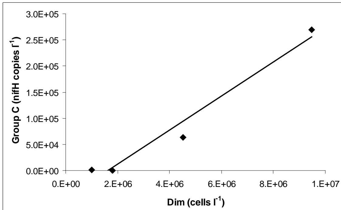
Figure IV-1: Correlation of Group C with Dim Synechococcus Abundances. Group C abundances were estimated by qPCR and are reported as nifH copies l -1 . Dim Synechococcus cell abundances (cells l -1 ) were determined by analytical flow cytometry.
