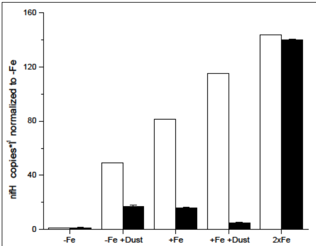
Figure 4. Differences in Trichodesmium nifH abundances after 3 Days (60 hours). Average DNA (white bars) and cDNA (black bars) abundances ( nifH copies l^{-1} ) were normalized to the -Fe control. Standard error bars are shown.
