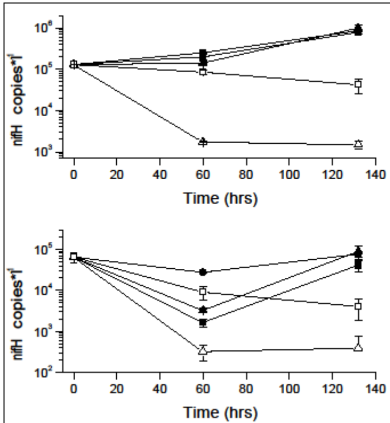
Figure 3. Effects of dust and/or iron on nifH DNA and cDNA. Average abundances of nifH DNA (a) and cDNA (b) ( nifH copies l^{-1} ) during the culture experiment. Error bars indicate standard error. Symbols refer to the treatments as follows: 2x Fe-black circles, +Fe-black triangles, Dust+Fe-black squares, -Fe-white triangles, and Dust-Fe-white squares.
