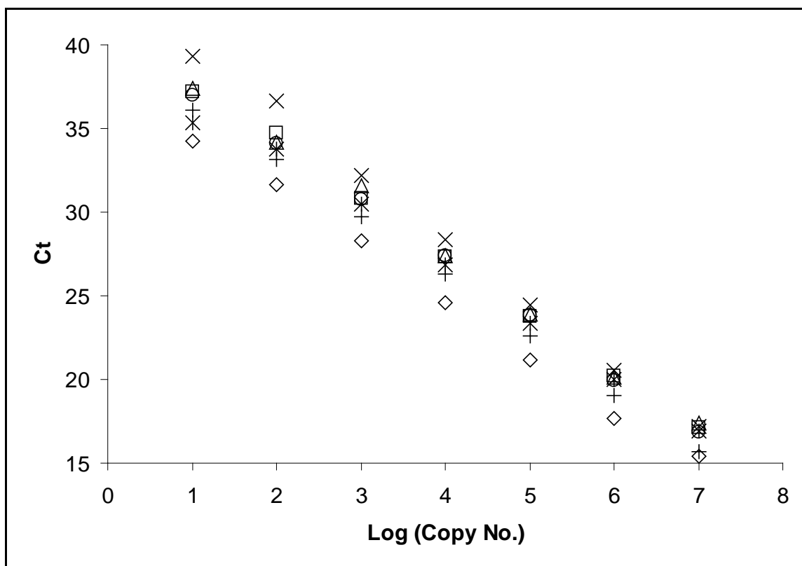
Figure II-1: Average Standard Curves Standard curves for the filamentous ('o', y=-3.47x + 40.8 , R^2=0.999 ), Group A ('+', y=-3.45x + 39.9 , R^2=0.999 ), Group B ('Δ', y=-3.42x + 41 , R^2=0.998 ), Group C ('x', y=-3.8x + 43.6 , R^2=0.998 ), Gamma A ('□', y=-3.43x + 41 , R^2=0.998 ), Gamma P ('◇', y=-3.27x + 37.7 , R^2=0.997 ), and CIII ('*', y=-3.21x + 39.5 , R^2=0.994 ) plasmids are shown. Error bars have been omitted to improve visualization.
