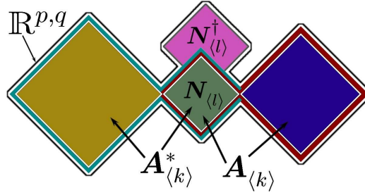
Fig. 2.8: Null blades: if N_{\langle l \rangle} is part of \mathbf{A}_{\langle k \rangle} then N_{\langle l \rangle} is part of \mathbf{A}_{\langle k \rangle}^* as well. The perpendicularity of the subspaces is indicated by the right angles between the rhombi. N_{\langle l \rangle} and N_{\langle l \rangle}^\dagger are parallel (perpendicular) w.r.t the inner product (Euclidean scalar product), although N_{\langle l \rangle}^\dagger \wedge N_{\langle l \rangle} \neq 0 .
