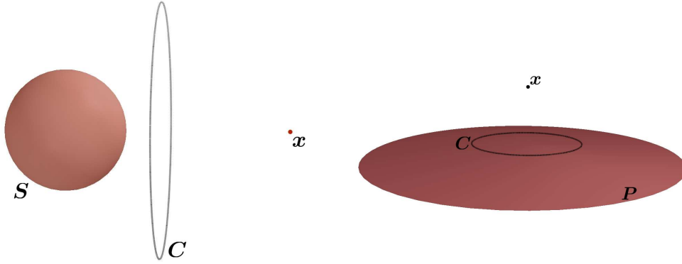
Fig. 3.7: Degenerate circles: points, here x , are treated as spheres with radius zero. The outer product C = x \wedge S , where S might be imaginary, gives the imaginary circle C . The same holds if a plane P is used.
