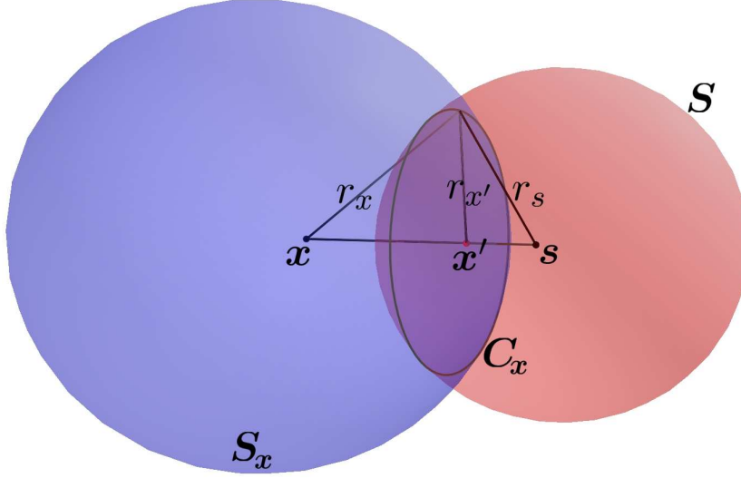
Fig. 3.6: Inversion: the inversion \mathbf{x}' of point \mathbf{x} ( \mathbf{s} ) in the sphere \mathbf{S} ( \mathbf{S}_x ) represents the center of the circle \mathbf{C}_x = \mathbf{S} \wedge \mathbf{S}_x , where \mathbf{S}_x := \mathbf{x} + (\mathbf{x} \cdot \mathbf{S})\mathbf{e} .
