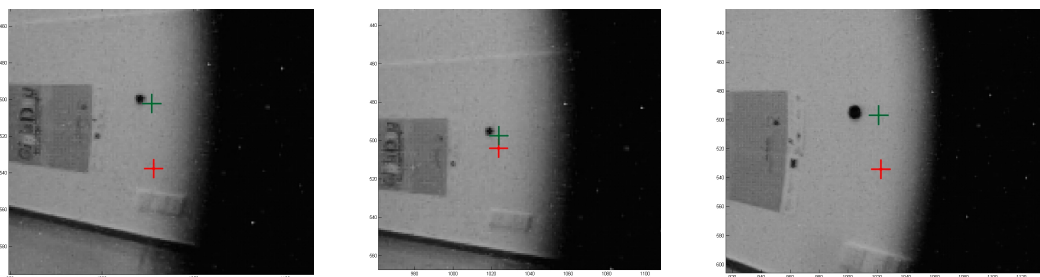
Fig. 8.20: Estimated epipoles: magnification for the scenarios 4x5 (l), 3x5 (c) and 7x8 (r). The differences in pixel are 34, 7 and 37, respectively. Scenario 3x5 represents an average situation.
