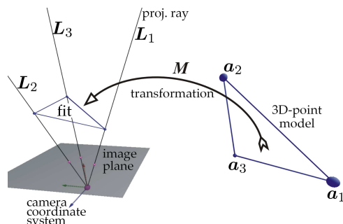
Fig. 4.3: 3-point pose estimation in 3D
