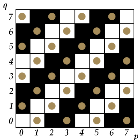
Fig. 2.6: Pseudoscalar: a white square denotes an algebra \mathbb{R}_{p,q} where \mathbf{I} \in \mathbb{R}_{p,q} squares to plus one, so that \mathbf{I}^{-1} = \mathbf{I} . A disc indicates that the pseudoscalar \mathbf{I} commutes with all elements of that algebra.
