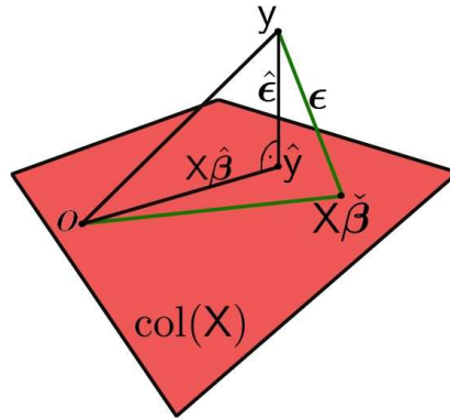
Fig. 5.1: LS principle for the linear model: orthogonal projection of y onto the expectation surface \text{col}(X)(\beta) = X\beta for the homoscedastic case; \hat{y} = X\hat{\beta} is most plausible if y was observed.
