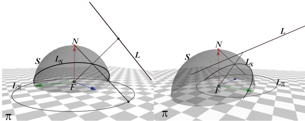
Fig. 8.3: Two views of the mapping of line L to L_\pi via great circle L_S on \mathcal{S} . The mapping of a sample point on L to the corresponding point on L_\pi is shown as well.
