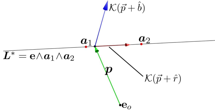
Fig. 3.10: Line L passing through the points a_1 and a_2 : the mutually orthogonal vectors \hat{r} , \vec{p} and \hat{b} form a right-handed system, \hat{b} = \hat{r} \times \vec{p}/d .
