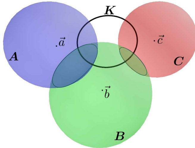
Fig. 3.3: Circle from spheres: the circle K^* = A \wedge B \wedge C hits all the spheres at right angles (it does not pass through the centers).
