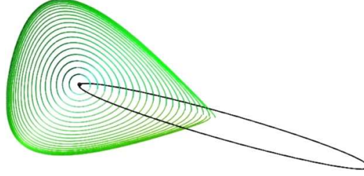
Fig. 7.1: Inner product isolines: the inner product of a point and a circle tends to be isotropic with decreasing proximity to the circle.
