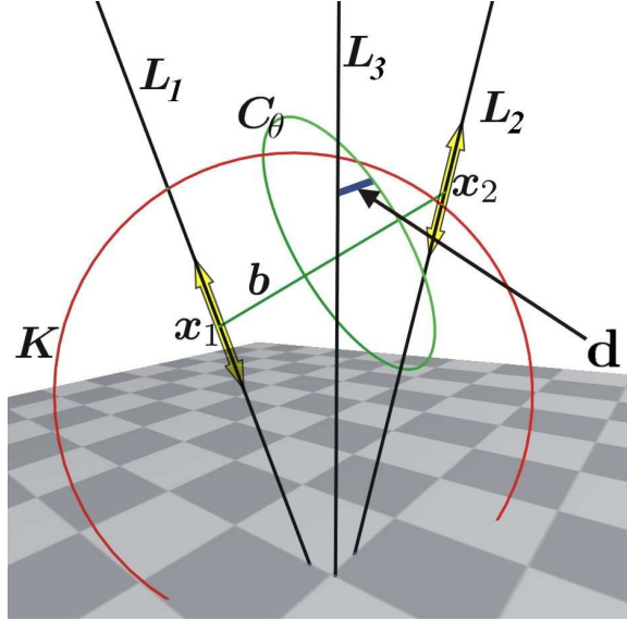
Fig. 4.6: Distance d between circle \mathbf{C}_\theta and the third projection ray \mathbf{L}_3 .
