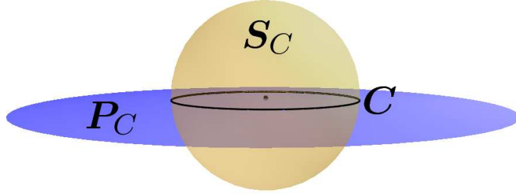
Fig. 1.1: Construction of the circle C from sphere and plane.
