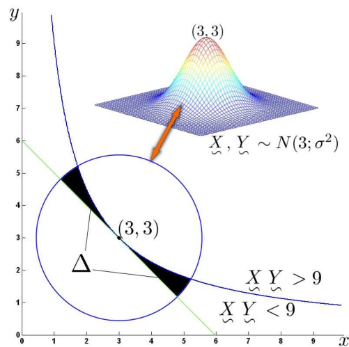
Fig. 6.1: Product of Gaussians: the random variable Z = XY , \sigma = 3/5 , cannot be Gaussian as there are more values smaller than nine (the mean of Z ) than values greater than nine, cf. figure 6.2; the difference can be thought of as twice the area denoted with \Delta .
