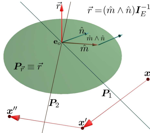
Fig. 3.15: Rotation of \mathbf{x} by \mathbf{R} = \mathbf{P}_2\mathbf{P}_1 , where \mathbf{P}_1 = \hat{n} and \mathbf{P}_2 = \hat{m} (planes indicated by lines only). The vector \vec{r} denotes the orientation (see page 25) of the rotation plane \mathbf{P}_{\vec{r}} \equiv \vec{r} = (\hat{m} \wedge \hat{n}) \mathbf{I}_E^{-1} = \hat{m} \times \hat{n} . Note that \mathbf{x} is negatively rotated, i.e. in a non-right-handed sense, regarding \vec{r} .
