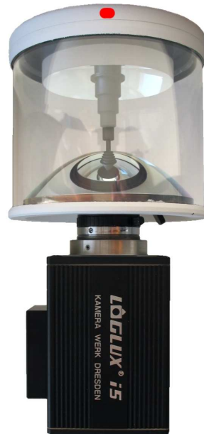
Fig. 8.1: Paracatadioptric imaging system 2
