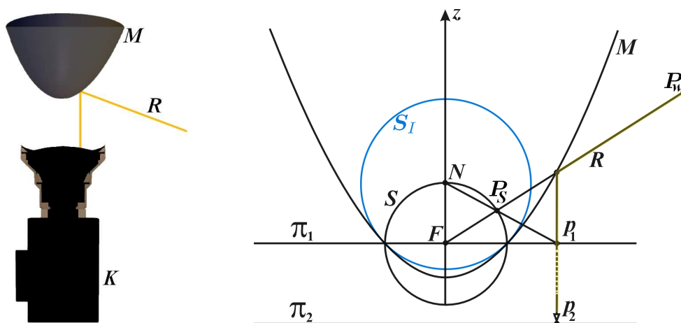
Fig. 8.2: Left: catadioptric vision sensor (camera K + parabolic mirror M ). Right: mapping of the world point \mathbf{P}_w \rightarrow the image planes \pi_1 and \pi_2 are identical.
