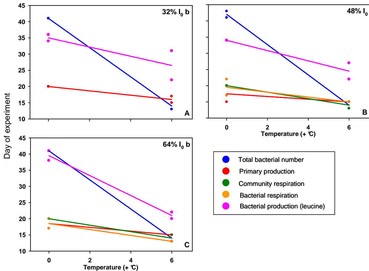
Figure 5: Acceleration of peaks of the different parameters for the temperature increase of \Delta T +0^\circ\text{C} to +6^\circ\text{C} at the respective light treatments from the 2008 experiment. The day of each peak is plotted against its respective temperature and the relationship is assessed by linear regression. For equations see Annex Table 1.
