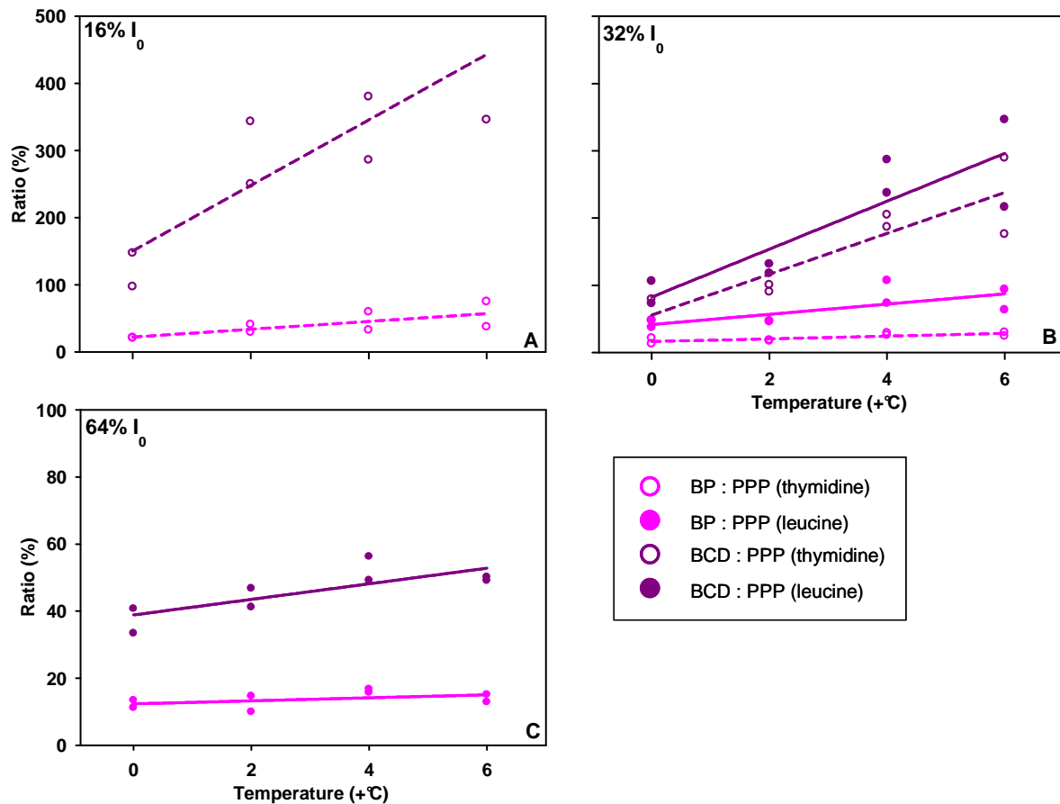
Figure 19. Ratios of bacterial production (BP) and bacterial carbon demand (BCD) to particulate primary production (PPP) at the individual peak periods, plotted against the respective temperatures. Results from the 2005-2007 experiments. The relationship between the ratios and temperature is assessed by linear regression. For equations see Annex Table 13. Note the different scales on the y-axis.
