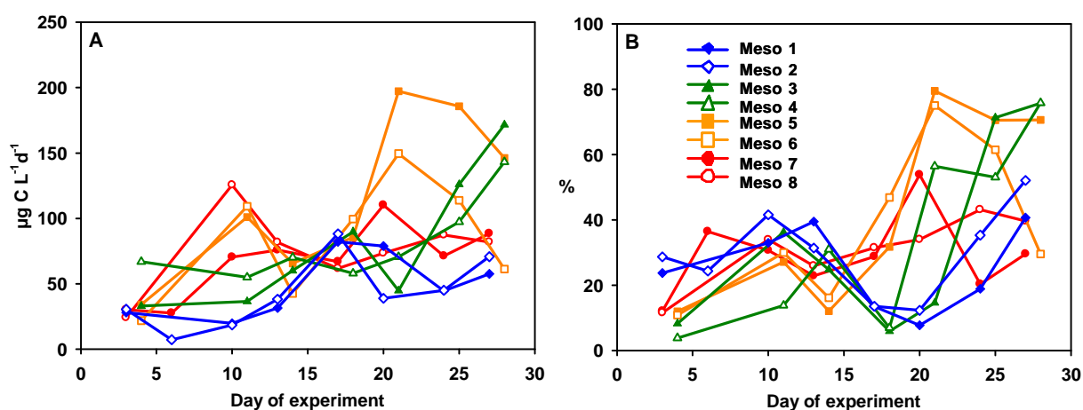
Figure 3. Dynamics of bacterial carbon demand (A) and bacterial growth efficiency (B) during the course of the experiment. Same colours represent the two replicate mesocosms run at the same temperature: blue: in situ temperature (2.5°C), green: 4.5°C, orange: 6.5°C, red: 8.5°C.
