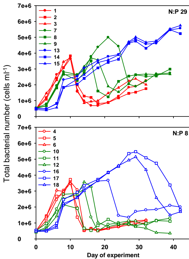
Figure 6. Dynamics of total bacterial numbers (cells ml -1 ) during the course of the experiment in the high-N (N: P 29) and low-N (N: P 8) treatments.
