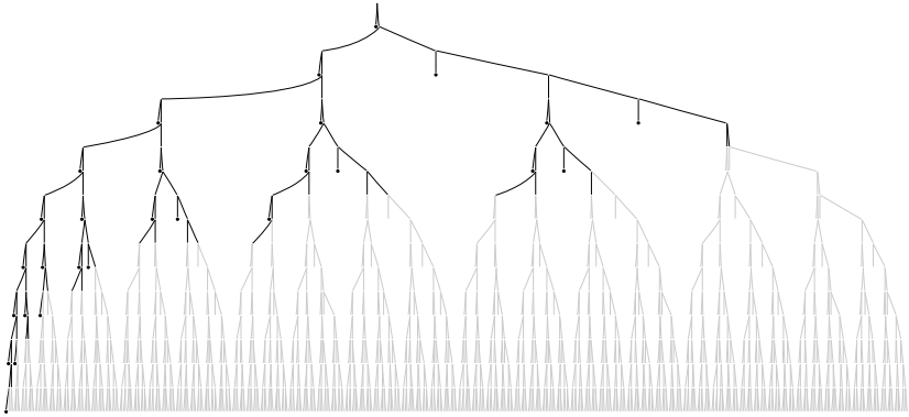
Figure 3.2: Level diagonalisation of [Bool] values
