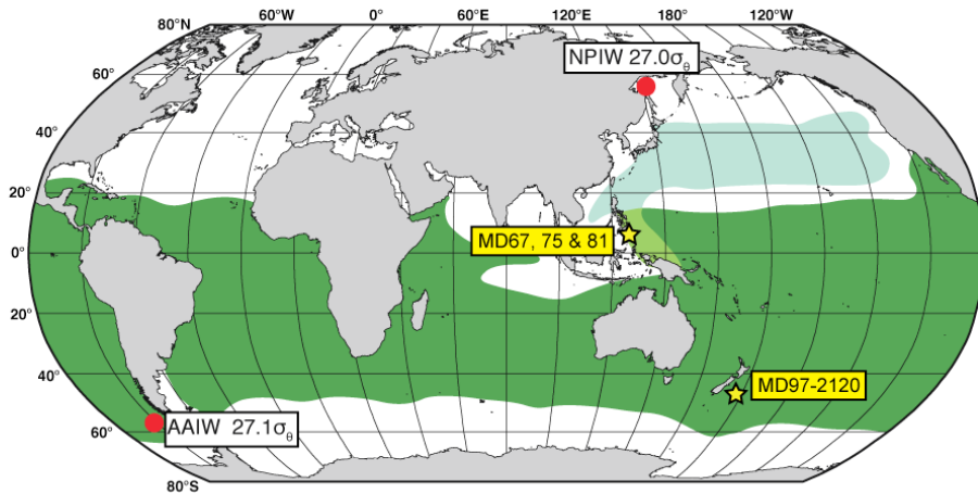
Fig. 2 – Locations of AAIW (dark green) and NPIW (light green) salinity minima in the world ocean (modified from Talley, 1999). Yellow stars indicate the position of cores MD06-3067, MD06-3075 (this study), MD98-2181 (Stott et al., 2007a) and MD97-2120 (Pahnke and Zahn, 2005). Red dots indicate the position of AAIW and NPIW production zones. Note the overlap of AAIW and NPIW in the western equatorial Pacific.
