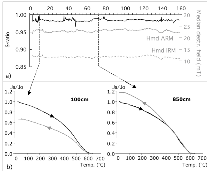
Fig. 3: Magnetic parameters defining the magnetic mineralogy in Core MD06-3067. a) S_{ratio-0.3T} (black line) and median destructive fields of ARM and IRM (Hmd IRM in dashed grey line and Hmd ARM in continuous grey line); b) two representative thermomagnetic curves obtained from different horizons with the heating curve in black and the cooling curve in grey. All indicate that the main carrier is low Ti-content magnetite.
