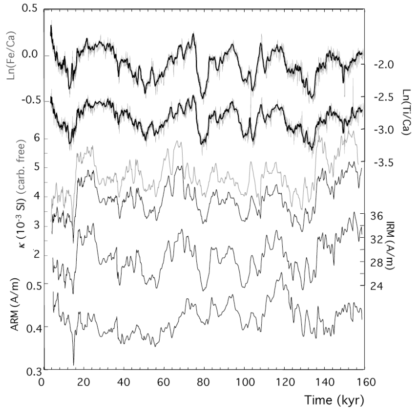
Fig. 6: Ti/Ca and Fe/Ca log-ratio (and a 7 points-running average) and bulk magnetic parameters ( \kappa , IRM and ARM) curves versus time in Core MD06-3067. The magnetic susceptibility calculated on a carbonate-free basis is also reported on the same vertical scale as \kappa by the grey curve.
