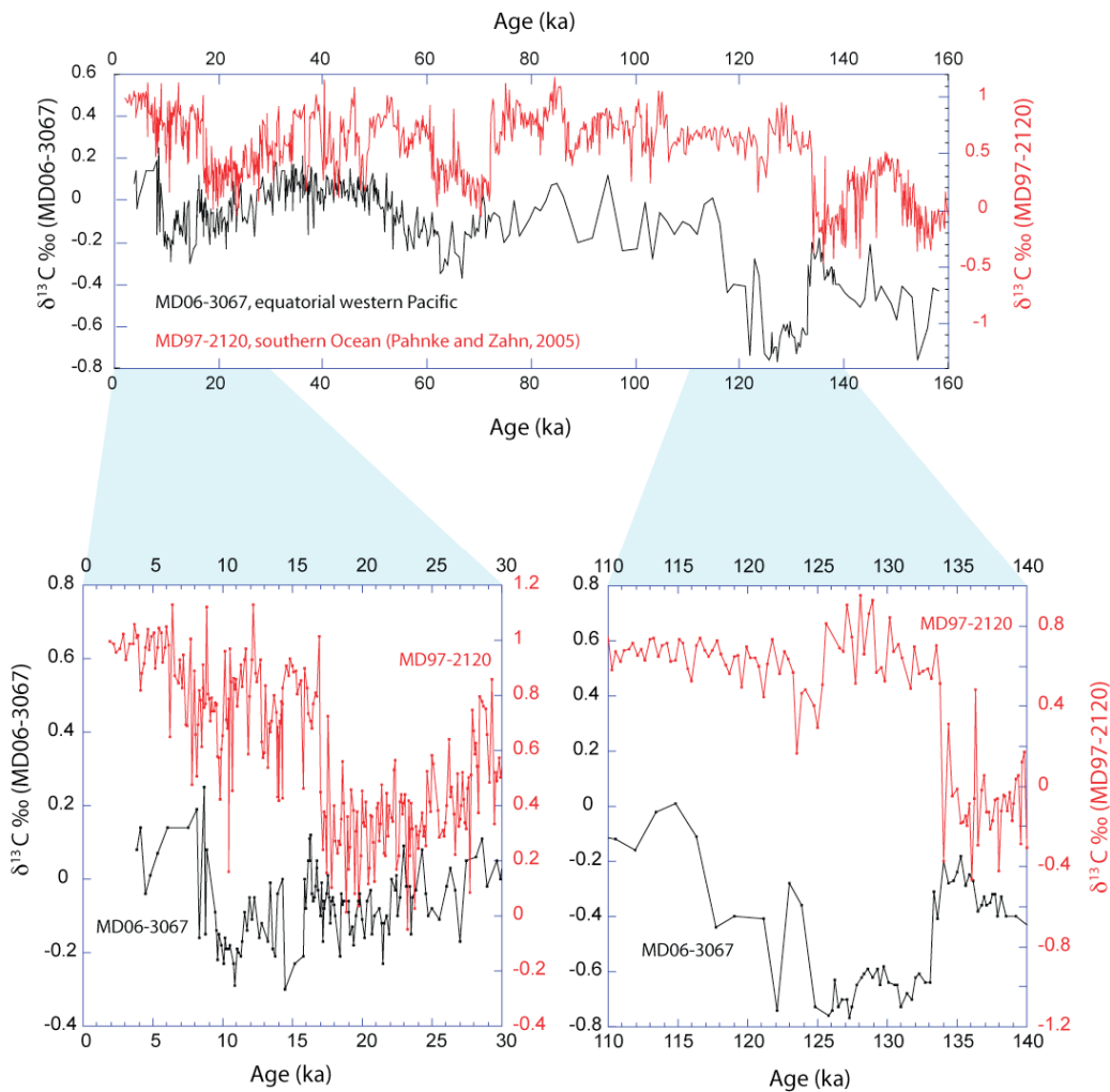
Fig 6 – Benthic \delta^{13}\text{C} signals from Core MD06-3067 (black solid line) and MD97-2120 (red solid line; Pahnke and Zahn, 2005) over the last 160 kyrs (top). Bottom right and left figures are a zooming in on terminations II and I, respectively.
