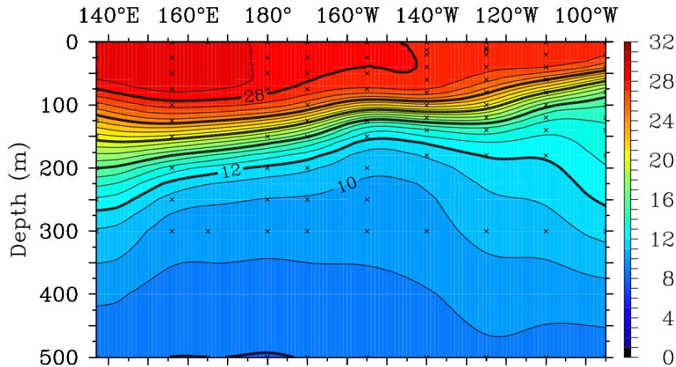
Fig. 9 – Monthly mean upper water temperature (°C) in the equatorial Pacific (5°N) for June 2007. Note the deepening of the thermocline in the western part of the basin. Data from TAO/NOAA
