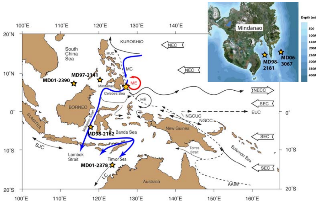
Figure 1. Location of Core MD06-3067 (orange star), bathymetry, and regional circulation in the Australasian area (modified from Fine et al., 1994). Solid blue lines indicate main path of Indonesian Throughflow. Red circular arrow indicates Mindanao Eddy generating Mindanao Dome. NEC is North Equatorial Current, NECC is North Equatorial Counter Current, SEC is South Equatorial Current, EUC is Equatorial Undercurrent, NGCC is New Guinea Coastal Current, NGCUC is New Guinea Coastal Undercurrent, MUC is Mindanao Undercurrent, AAIW is Antarctic Intermediate Water, SJC is South Java Current, LC is Leeuwin Current, MC is Mindanao Current, ME is Mindanao Eddy, and HE is Halmahera Eddy. Positions of cores discussed in this study are also shown: Core MD97-2141 (de Garidel-Thoron et al., 2001; Dannemann et al., 2003; Oppo et al., 2003; Rosenthal et al., 2003), Core MD01-2390 (Steinke et al., 2010), Core MD98-2181 (Stott et al., 2002; Saikku et al., 2009), Core MD98-2162 Visser et al., (2003), and Core MD01-2378 (Xu et al., 2006, 2010).
