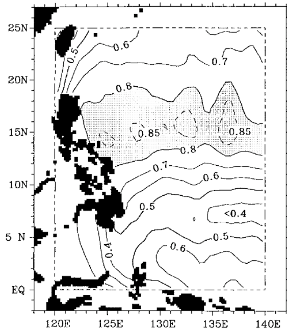
Fig. 7 – Distributions of probability of NPTW around the Philippines (Qu et al., 1999), defined as a salinity maximum ( 34.85 psu) in potential density range of 23.0 - 25.0 \sigma\theta .
