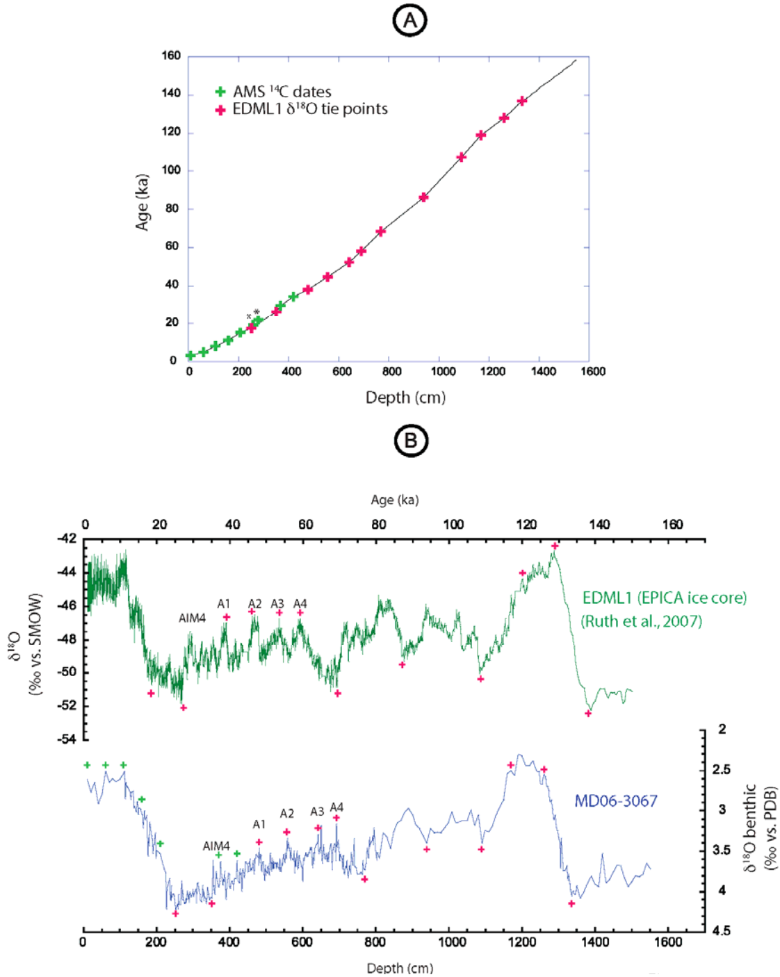
Figure 3. Age model based on seven accelerator mass spectrometry (AMS) ^{14}\text{C} dates and 12 \delta^{18}\text{O} events for Core MD06-3067 (Table 1).
