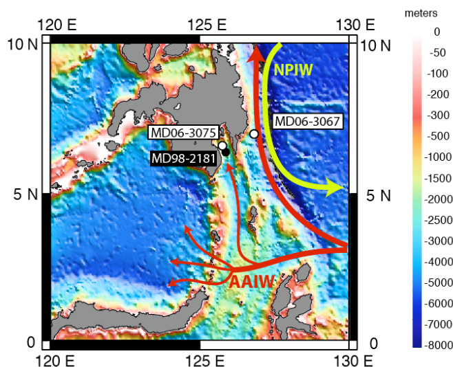
Fig. 1 – Location of cores MD06-3067 and MD06-3075 (this study) as well as MD98-2181 (Stott et al., 2007a). Note the relatively shallow sill extending south of Mindanao Island isolating the Davao Gulf from the open ocean. AAIW: Antarctic Intermediate Waters; NPIW: North Pacific Intermediate Waters. Map modified from Liu and Dittert (2010), generated from the ETOPO2 v.2 (NGDC) database.
