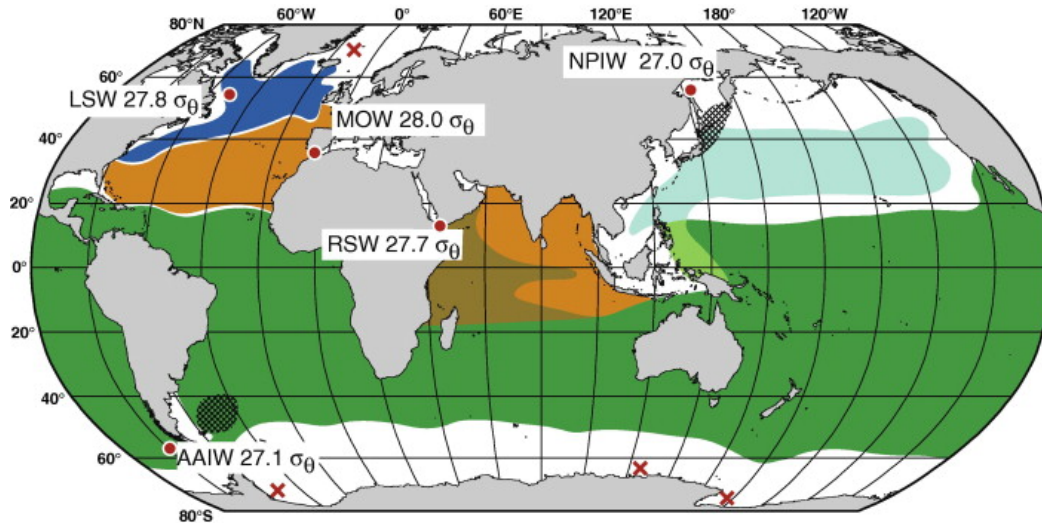
Fig. 4 – Schematic of low salinity (blue, green and blue-green) and high salinity (orange) intermediate water masses, after Talley (1999). The overlap of Red Sea Water and AAIW is shown in brown; the overlap of NPIW and AAIW is shown with an intermediate shade of green. Red dots represent intermediate water sources; these are sites of open ocean convection (LSW and AAIW), or sill overflow (MOW and Red Sea Water), or shelf brine rejection (NPIW). Potential density at each source is listed. Red X's represent deep and bottom water sources.
