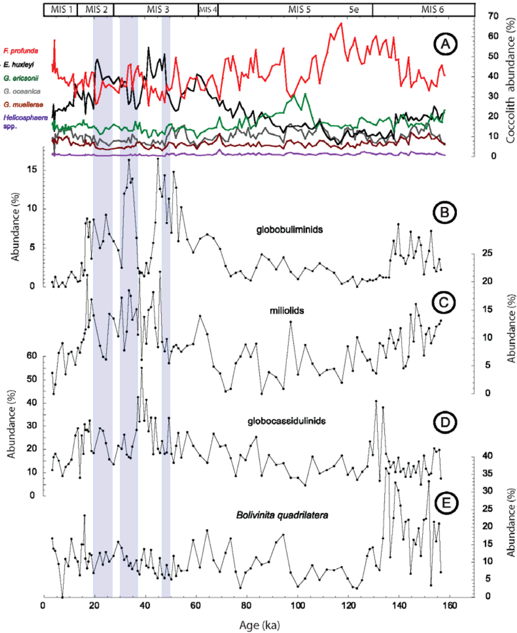
Figure 6. Relative percentage abundance of major coccolith and benthic foraminiferal high-productivity index taxa in Core MD0-3067. Blue bars indicate periods of intense surface and upper thermocline cooling, implying a reduced upper ocean temperature gradient.
