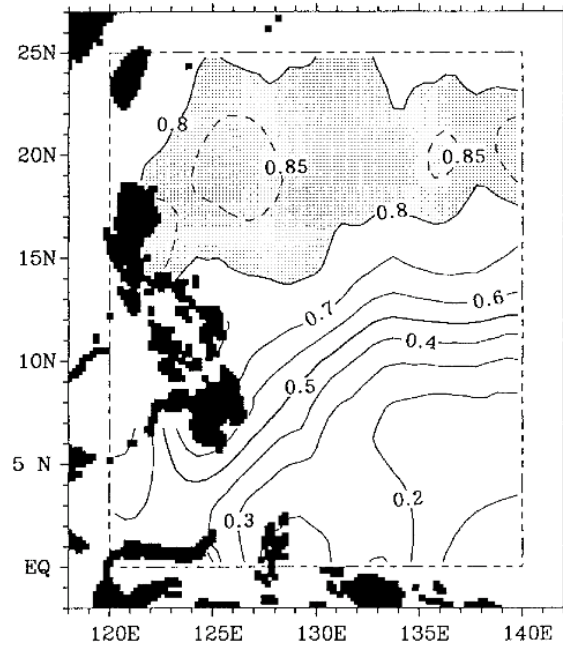
Fig. 6 – Distributions of probability of NPIW around the Philippines (Qu et al., 1999), defined as a salinity minimum ( <34.45 psu) in potential density range of 26.4 - 27.0 \sigma\theta .
