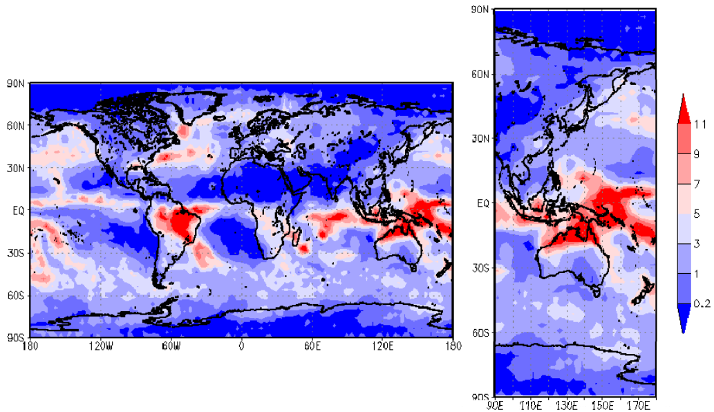
Fig. 1 – a) Winter position of the ITCZ revealed by monthly precipitation rates (mm/day) on a worldwide (left) and regional (right) scale. Data for february 2004 from Global Precipitation Climatology Project ( http://cics.umd.edu/~yin/GPCP/main.html ). Note the rainbelt reaching north of Australia, whereas low precipitation prevails over India and China during the South Indian and East Asian monsoons.
