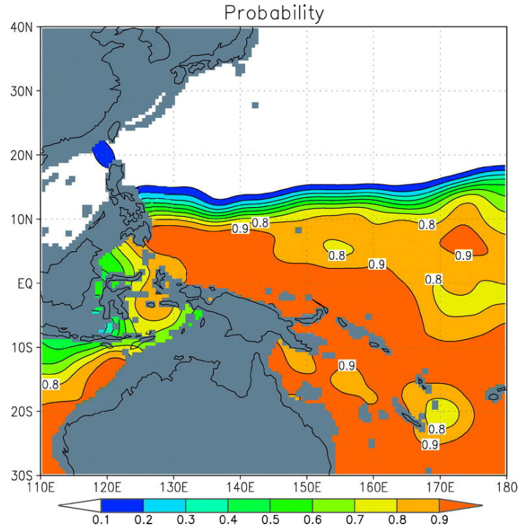
Fig. 5 – Probability of AAIW in the Australasian region, defined as the percentage of salinity profiles that contain at least one salinity minimum at the potential density range of 27.0–27.4 \sigma\theta (modified from Qu et al., 2004).
