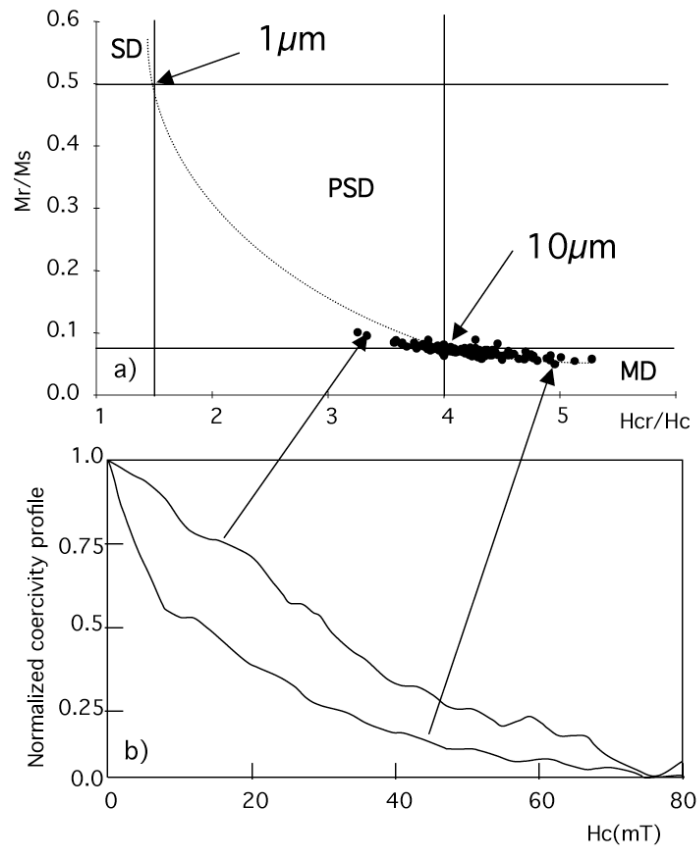
Fig. 5: Magnetic hysteresis parameters in Core MD06-3067 reported in a) as M_r/M_s versus H_{cr}/H_c ratios (Day et al., 1977) with the hyperbole (dashed line) corresponding to magnetite grain size distribution between SD (single domains), PSD (pseudo-single domains) and MD (multi-domains). b) two coercivity profiles from FORC diagrams (profiles along H_u=0 ) showing the different distribution of coercivities in samples characterized by the mean finest grains (grey) and coarsest grains (black).
