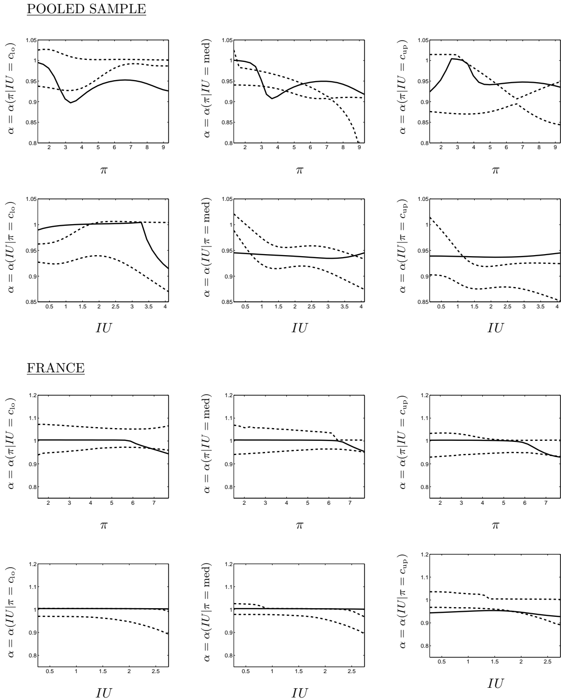
Fig. 9.2: Functional coefficient estimates for the pooled sample and France
