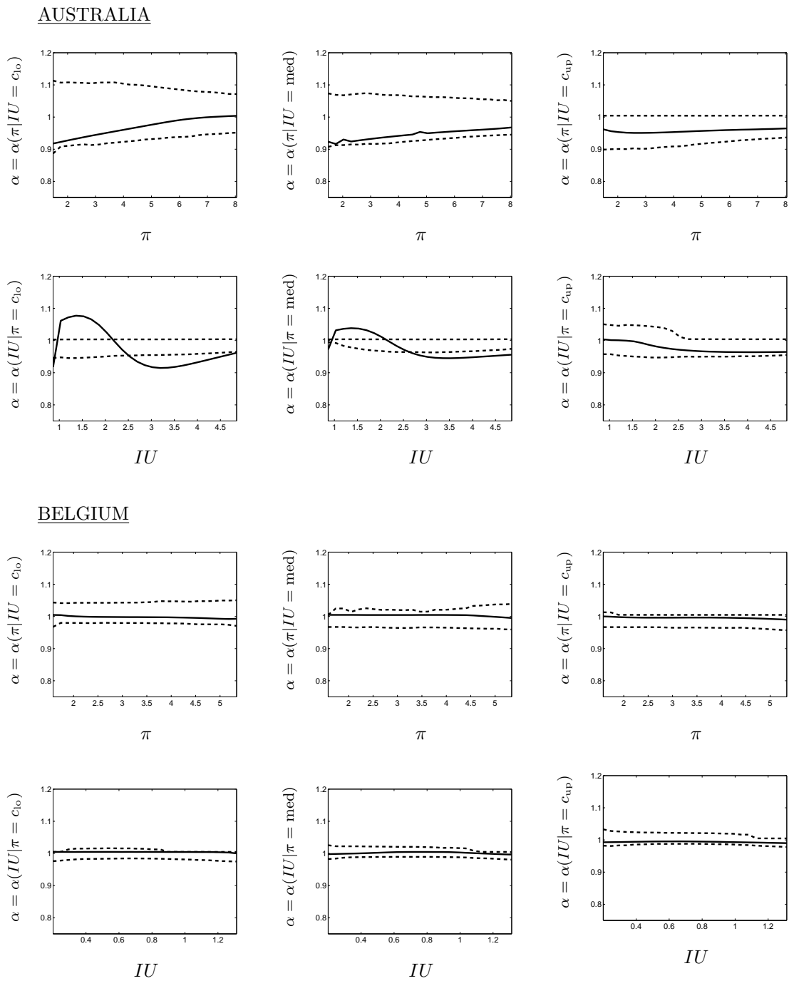
Fig. 11.1: Functional coefficient estimates for Australia and Belgium
