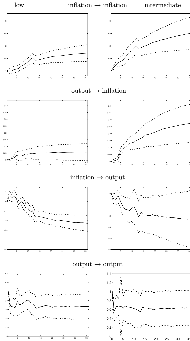
Fig. 4.2: Average accumulated impulse response functions for subgroups Considered subgroups are economies with low ( < 2.5\% ) and intermediate inflation rates (between 2.5\% and 5\% ). For further descriptions see Figure 1.
