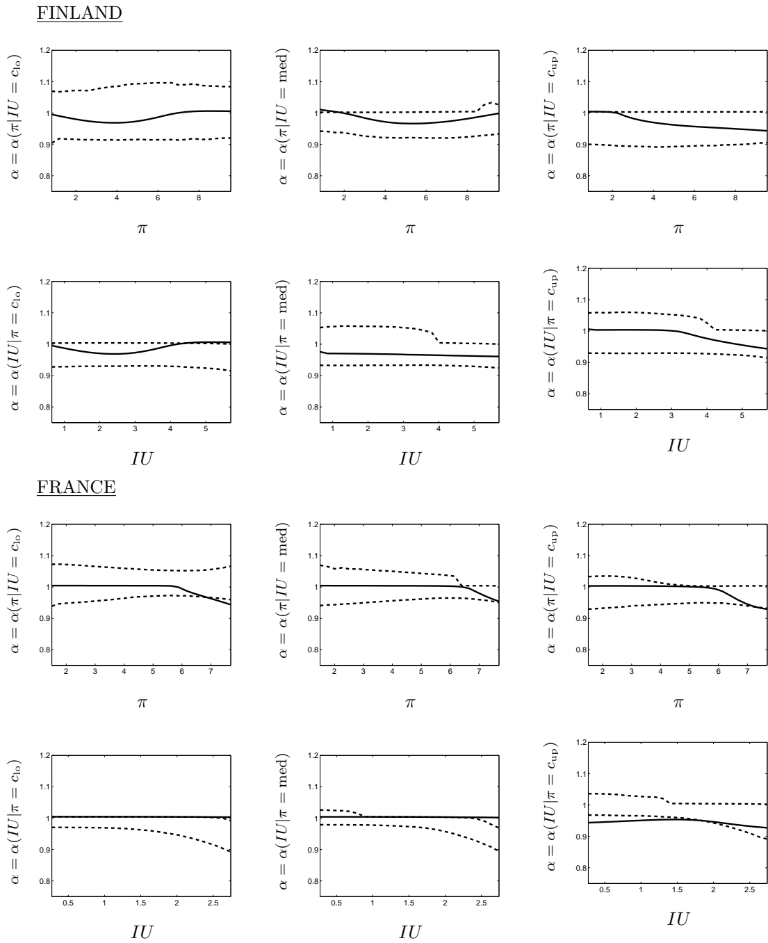
Fig. 11.3: Functional coefficient estimates for Finland and France
