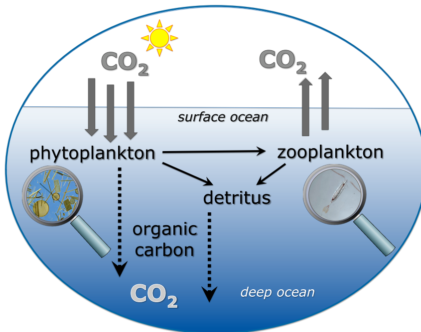
Figure 1.1: Sketch of the biological pump. CO 2 enters the ocean and is converted into biomass via photosynthesis. Part of the biomass is cycled through the food-web and CO 2 is re-released into the atmosphere; part of the biomass sinks into the deep ocean, where it is slowly remineralised to CO 2 . Image sources: National Geographic (diatoms), oceanexplorer.noaa.gov (copepod).
