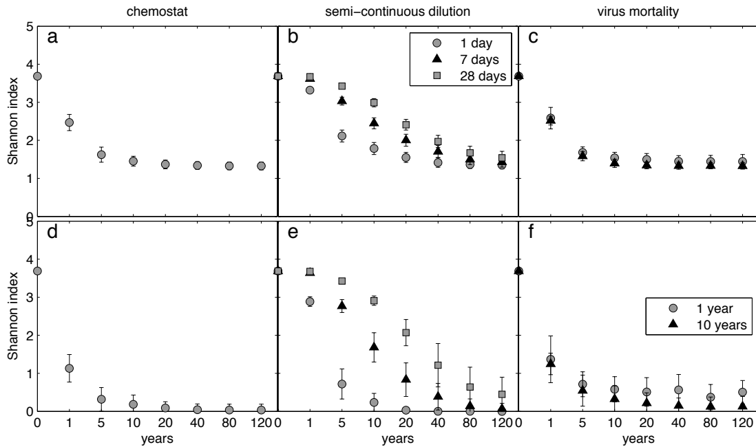
Figure 4.2: 40 phytoplankton species on 4 resources; Shannon diversity index after 1, 5, 10, 20, 40, 80 and 120 years, respectively, mean and standard deviation of replicate runs. Top row: simulations using equilibrium conditions on stoichiometry ( C_{eq} ), bottom row: Redfield stoichiometry ( C_{Redf} ). The different disturbance modes are: (a),(d) perfect chemostat; (b),(e) semi–continuous culture with dilution every 1, 7, 28 days; (c),(f) chemostat with ”virus infection” every 1 and 10 years.
