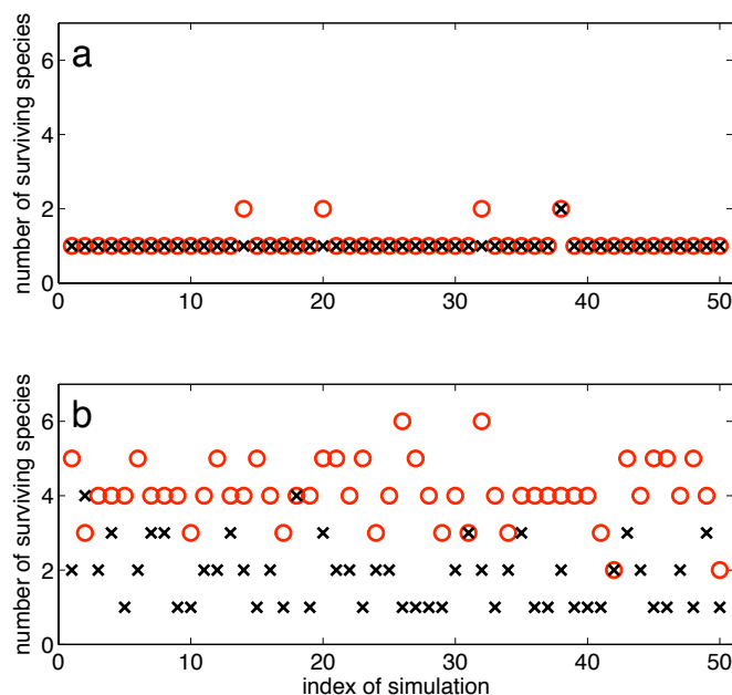
Figure 3.2: Number of surviving species at the end of 50 simulations over 20 years each; a: configurations C_{\text{Redf}}K_{\text{rand}} (black crosses) and C_{\text{Redf}}K_{\text{rank}} (red circles) and b: configurations C_{\text{eq}}K_{\text{rand}} (black crosses) and C_{\text{eq}}K_{\text{rank}} (red circles). Model configurations are described in table 3.4.
