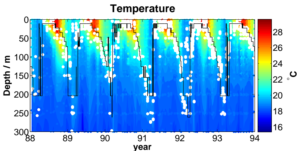
Figure 2.1: Temperature (contours) and modelled (black line) and observed (white dots) mixed layer depth, defined as the deepest point at which the density difference to the surface is less than 0.1 \text{ kg/m}^3 , at BATS.
