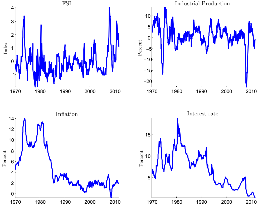
Figure 4.6: Variables included in the MSBVAR
