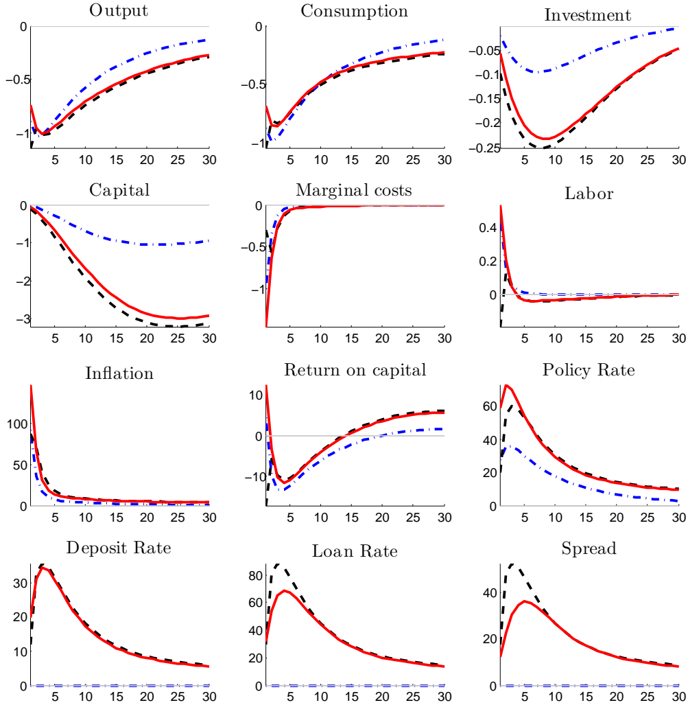
Figure A1: Impulse response functions to a shock in the level of TFP
