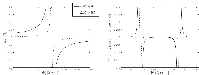
Figure 5.11. Linearization error for PD relocalization. Left graph: linearization error \mathcal{L}\mathcal{E}_f(p, \Delta p) in percent (see section 3.4.3). Right graph: remainder of the first order Taylor expansion for relocalization f of disparity.
