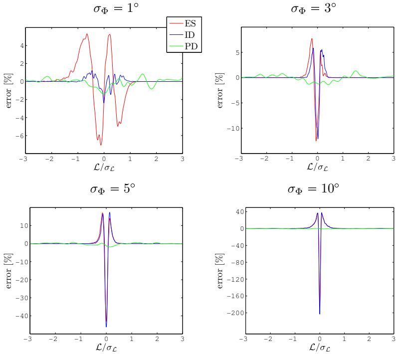
Figure B.3. Error of PDFs in percent of maximum density ( \max(\hat{\varphi}_\mathcal{L}) ) for distant landmarks (20 baselines). Horizontal axis represents the first component of landmarks view direction ( \mathcal{L} = \{\mathcal{X}^{\text{ES}}_{(1)}, \phi, x^{\text{PD}}_{(1)}\} ) normalized by its standard deviation. PDFs are cross sections for \Phi_{(2)} = 0 of distributions for (\Phi_{(2)}, \mathcal{L}) . Used initialization setup \Phi = 1^3 , x = 0_2 , y = (0.05 \ 0) . Positions standard deviation 0.05 baselines.
