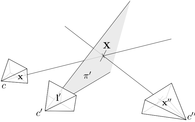
Figure 2.5. Visualization of TFFT mapping. Point-line correspondence \mathbf{x} \leftrightarrow \mathbf{l}' in c and c' respectively to \mathbf{x}'' in c'' . Mapping via the back projected plane \pi' for \mathbf{l}' . \mathbf{X} marks corresponding 3-space point.
