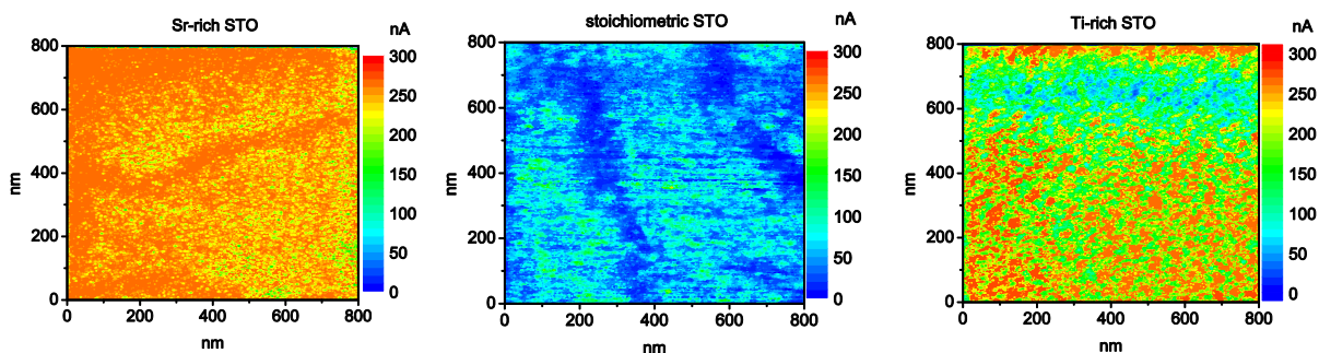
Figure 8-8: SET-process characteristics of STO films with different stoichiometries with a set-voltage of V_{\text{SET}} = +1.3\text{V} .
