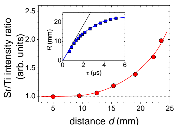
Figure 5-21: Sr/Ti emission intensity ratio as a function of the distance d from the STO target surface in Argon background gas. The inset shows an R - \tau of the STO plume front. With D_{TS} = \infty , T_S = 25^\circ\text{C} , p_{Ar} = 0.2\text{mbar} , F_L = 1.5\text{J}/\text{cm}^2
