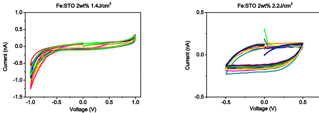
Figure 8-34: Pristine I(V) characteristics of Fe:STO (2wt%) films deposited at a) 1.4J/cm 2 and b) 2.2J/cm 2 . Measurements performed by Chencheng Xu.
