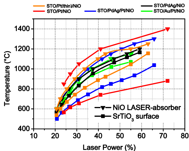
Figure 3-10: Substrate temperature (STO) and absorber temperature (NiO) versus IR-laser energy for different heat sink materials and combinations of Pt (80 \mu m), Pt-thin (20 \mu m), PdAg (20 \mu m) and Au (20 \mu m).
