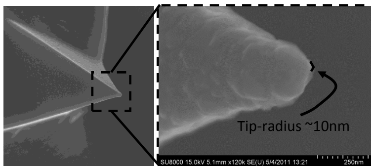
Figure 4-11: Diamond (boron doped) coated Si tip. Only the outermost tip touches the surface and therefore the tip has a radius of \sim 10 nm
