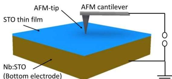
Figure 8-1: Schematics for resistive switching of STO films on Nb:STO by LC-AFM. The AFM-tip constitutes the top electrode whereas the Nb:STO describes the bottom electrode.
