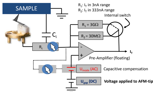
Figure 4-13: Circuit diagram for low conductivity AFM (LC-AFM) with Pre-Amplifier. R_C : contact resistance, C_i : internal capacitance, U_{gap} : applied voltage, I_T : Pre-Amplifier Signal
