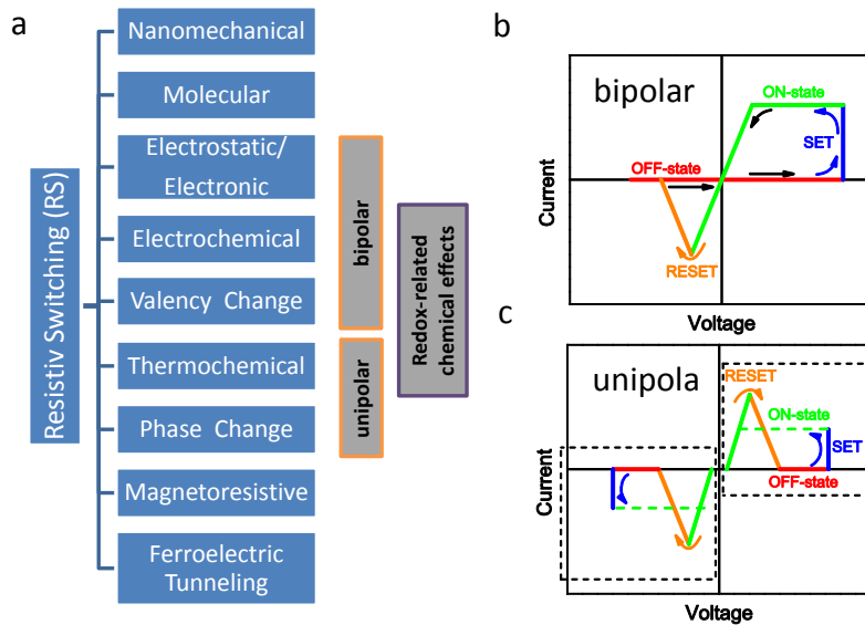
Figure 2-6: a) Resistive switching operation mechanisms b) Bipolar RS schematics c) Unipolar RS schematics. Adopted from [38]
