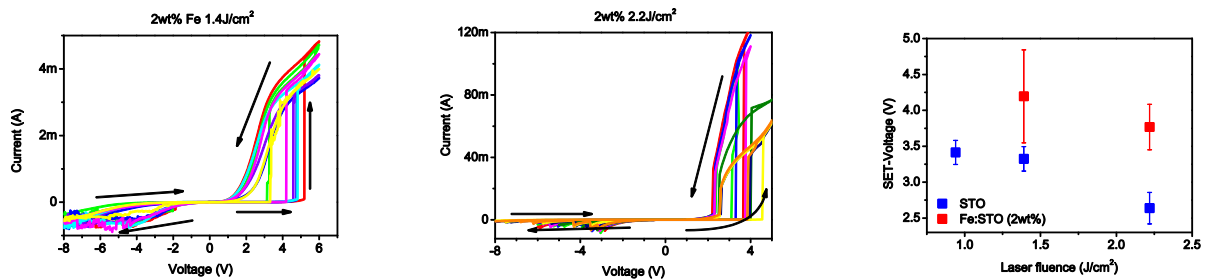
Figure 8-35: RS characteristics of MIM structures (Pt/Fe:STO/Nb:STO) for 2wt% Fe:STO deposited at different laser fluence. a) 1.4J/cm 2 , b) 2.2J/cm 2 , c) Set-voltage statistics. Measurements performed by Chencheng Xu.
