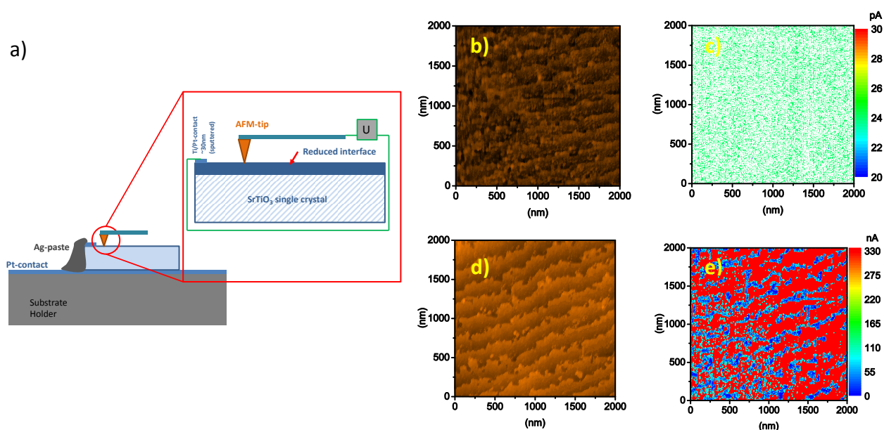
Figure 8-6: a) LC-AFM measurement setup to probe the effect of oxygen vacancies on the conductivity of a STO single crystal. Topography (b) and conductivity (c) of the STO single crystal annealed at T_s = 950^\circ\text{C} in atmosphere for t = 4 hrs with U_{\text{tip/read}} = +0.1\text{V} . Topography (d) and conductivity (e) of the STO single crystal annealed at T_s = 700^\circ\text{C} with P_{\text{ambient}} = 4 \cdot 10^{-8}\text{mbar} for t = 45\text{min} with U_{\text{tip/read}} = +0.3\text{V} .
