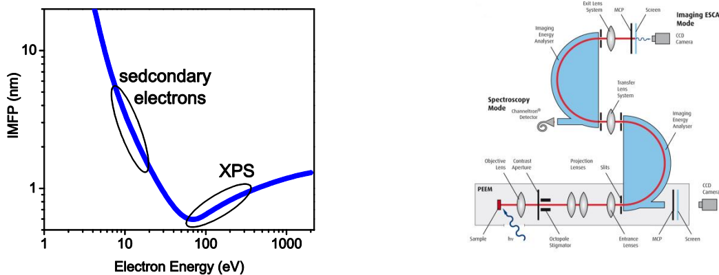
Figure 4-10: a) Inelastic mean free path (IMFP) of photo electrons adopted from [61] . b) Schematic working principle of a PEEM setup - Taken from Omicron Brochure for NanoESCA 500-V01/2007.
