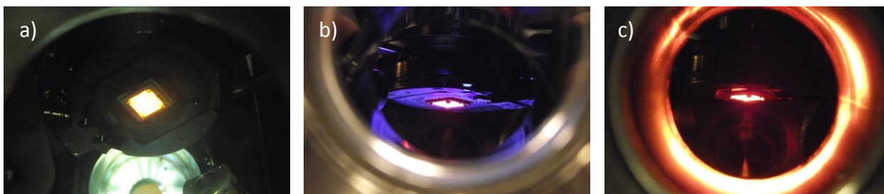
Figure 3-11: SrTiO 3 Substrat (10x10x1mm) clamped inside the high temperature holder with a substrate temperature of T_s = 1200^{\circ}\text{C} . a) Bottom view, b),c) Side view
