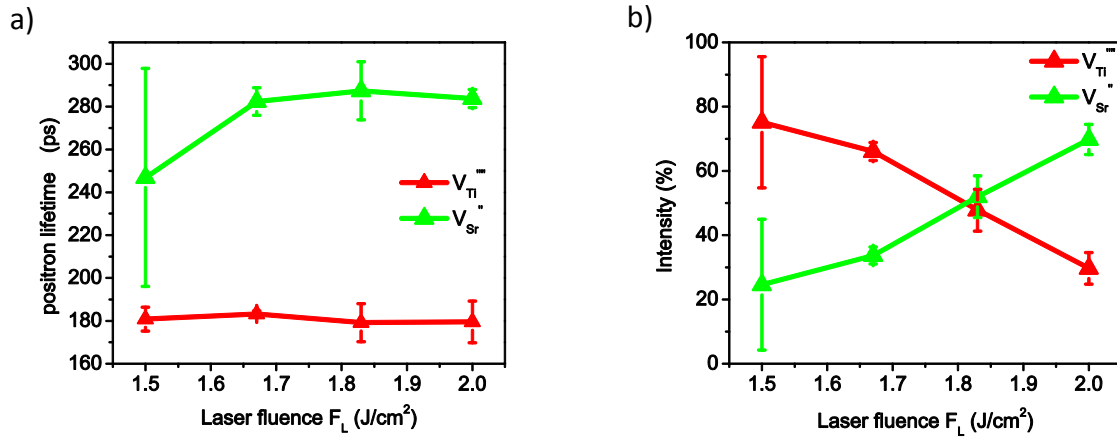
Figure 5-4: a) Deconvolved positron lifetimes vs. laser fluence for STO films with F_L > 1.5 J/cm 2 . b) Relative lifetime intensities of the deconvolved positron lifetimes vs. laser fluence.
