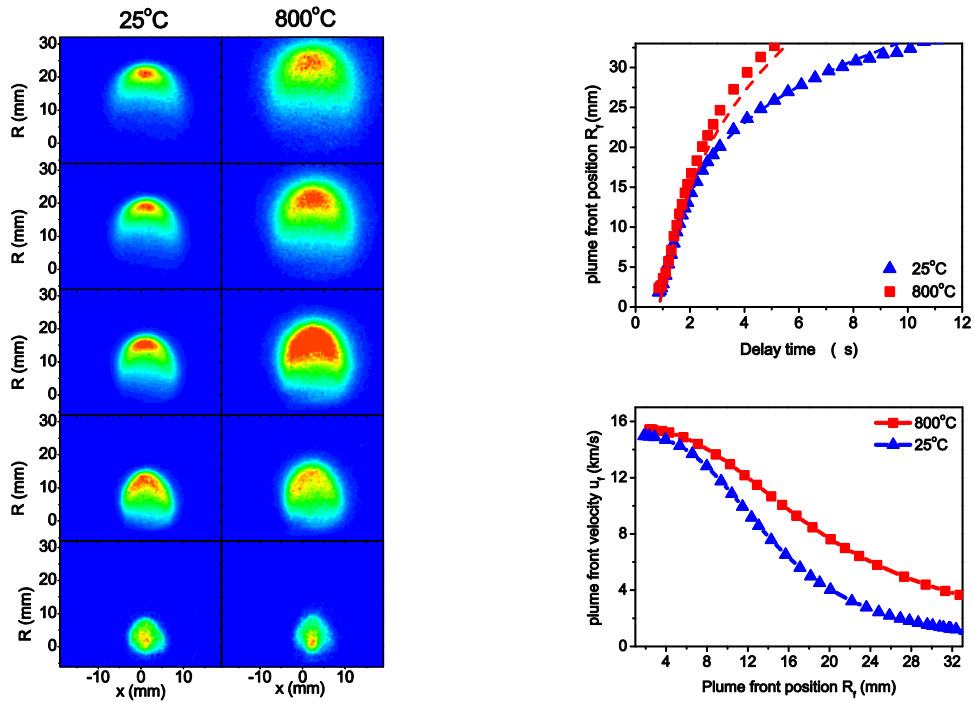
Figure 5-29: a) 2D plume images for different substrate temperatures. b) Plume front positions z_f for different substrate temperatures. c) Plume front velocity. F_L : 2.5J/cm 2 , p_{O_2} : 0.1mbar.
