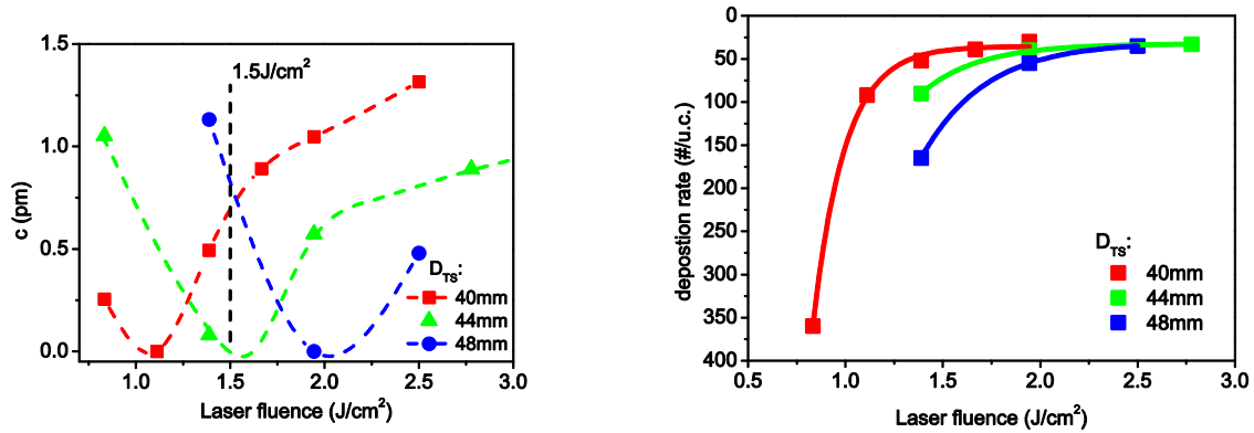
Figure 5-9: a) c-axis expansion of STO thin films d_{\text{STO}} \sim 200 nm at different laser fluencies and various target to substrate distance D_{\text{TS}} b) Growth rates of the STO films. All samples were grown on STO with TS: 800^\circ\text{C} , p_{\text{O}_2} : 0.1\text{mbar} , f_L : 5\text{Hz}
