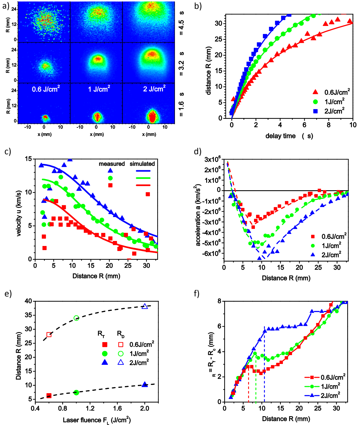
Figure 5-17: a) 2D images of the STO plume for different delay times \tau and laser fluencies F_L . b) R - \tau plots for the plume fronts at different laser fluencies c) Simulated plume front velocity u_f d) Simulated plume front acceleration a_f e) Transition points R_T from free expansion to shock-wave like expansion, R_D from shock-wave like to diffusion-like expansion f) Difference between plume front and plume center vs. travelled distance R . With p_{O_2} : 0.1mbar, T_s : 800°C.
