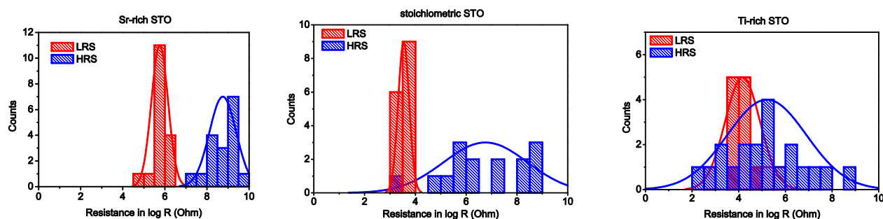
Figure 8-33: Statistics of the LRS and HRS values for different stoichiometries. a) Sr-rich STO with HRS/LRS \sim 1500, b) stoichiometric STO with HRS/LRS \sim 1800, c) Ti-rich STO with HRS/LRS \sim 11.
