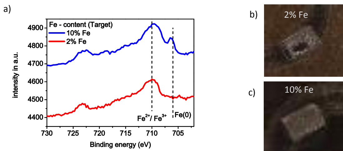
Figure 6-2: a) XPS signals within the ablation spot of a 2% and a 10% Fe doped STO target. F_L = 1.4\text{J}/\text{cm}^2 , #500, F_L = 5\text{Hz} . b) & c) Photographs of the ablation spots on the Fe:STO target after laser irradiation.
