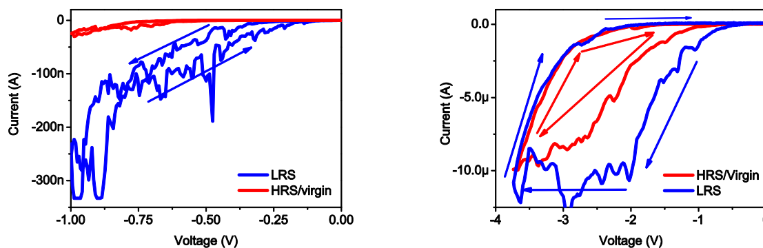
Figure 8-15: I(V) characteristics of the reset process for a LRS and HRS area. a) Low voltage characteristics of LRS and HRS. b) Higher voltage characteristics of the LRS and HRS area. The LRS exhibits eventually a NDR and resets into the HRS.
