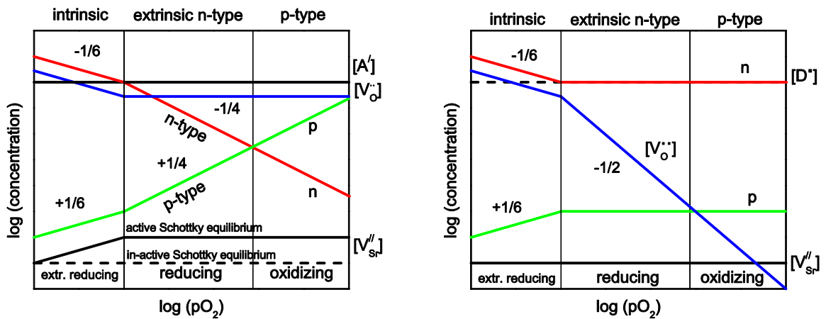
Figure 2-2: Schematic diagram of the charge carrier concentration in a) acceptor doped SrTiO_3 and b) donor doped SrTiO_3 as a function of oxygen pressure for 750K < T_S < 1250K .
