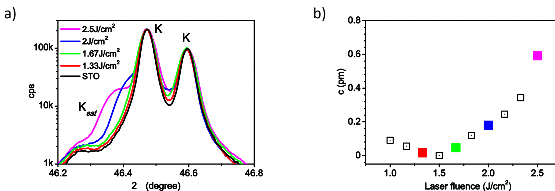
Figure 5-1: a) 2\Theta - \omega XRD intensity profile around the STO (002) peak for different laser fluencies. b) c-axis lattice expansion \Delta c = c_{film} - c_{STO-bulk} for different laser fluencies. T_S : 720°C, p_{O_2} : 0.2 mbar, f_L : 5Hz.
