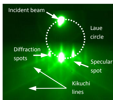
Figure 4-3: RHEED diffraction pattern of a vicinal SrTiO_3 surface recorded on the phosphor screen. The radius of the Laue-circle and the number of the diffraction spots depends on the incident angle of the e^- -beam.
