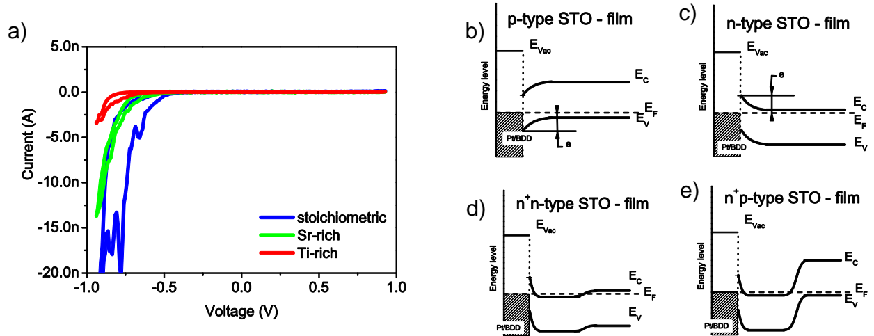
Figure 8-2: a) I(V) curves for pristine STO films with different stoichiometry and d_{\text{STO}} = 16 \text{ u.c.} Energy band diagrams for b) p-type STO in contact with Pt or BDD in equilibrium forming a Schottky contact ( \phi_m < \phi_{\text{STO}} ), c) n-type STO in contact with Pt or BDD in equilibrium forming a Schottky contact ( \phi_m > \phi_{\text{STO}} ), d,e) Ohmic contact between n + -type STO and Pt with a n-type or p-type STO below the n + -type STO.
