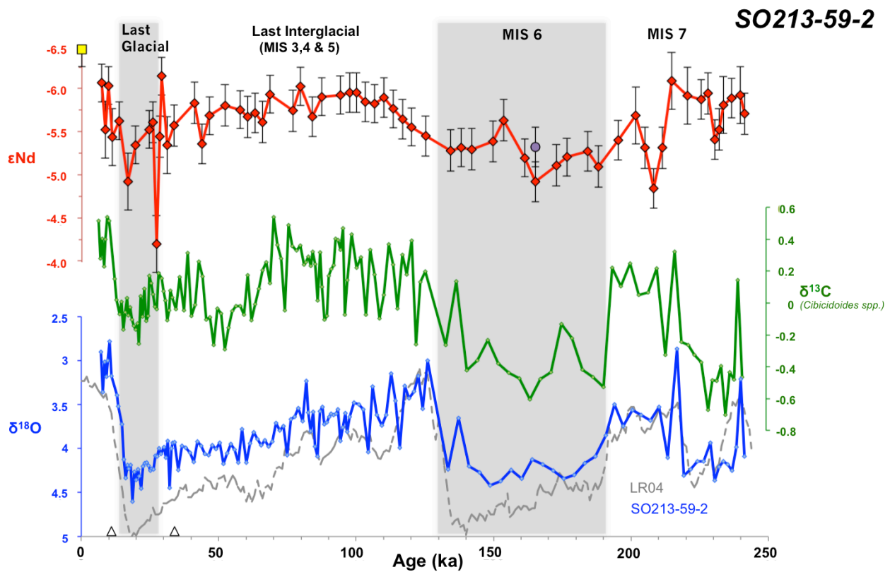
Figure 5.2. Nd (red), carbon (green) and oxygen (blue) isotope compositions of Core SO213-59-2, which covers the past ~240 ka. Nd isotope compositions ( \epsilon_{Nd} ) with error bars ( 2\sigma ) correspond to: Fe-Mn coatings of ‘unclean’ planktonic foraminifera (red diamonds), a fish tooth (purple dot), and present day seawater (yellow square: data from Molina-Kescher et al., 2014). Carbon ( \delta^{13}\text{C} ) and oxygen ( \delta^{18}\text{O} ) isotopes were obtained from benthic foraminifera ( Cibicidoides wuellerstorfi ). The global \delta^{18}\text{O} stack LR04 (grey dashed line: Lisiecki and Raymo, 2005) is shown for comparison. Grey bars indicate glacial periods identifiable in the \delta^{18}\text{O} data of core SO213-59-2.
