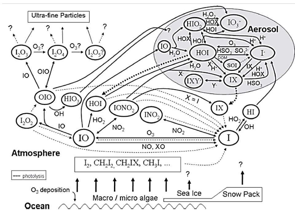
Figure III-11. Schematic of the atmospheric iodine photochemistry (Saiz-Lopez et al., 2012) with X and Y as halogen atoms and SOI standing for soluble organic iodine.
