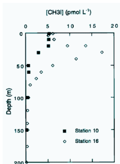
Figure III-4. The production by phytoplankton leads to similar depth profiles as observed for \text{CHBr}_3 and \text{CH}_2\text{Br}_2 with pronounced maxima in the Chl a maximum (Moore and Groszko, 1999).
