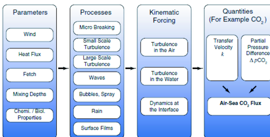
Figure III-8. Factors influencing the air-sea gas exchange of CO 2 , modified from Garbe et al. (2014).
