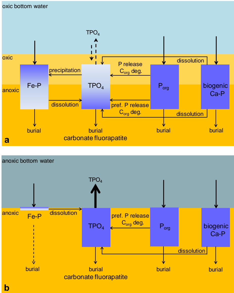
Fig. 1.2: Benthic P cycle under a oxic and b anoxic bottom-water conditions, considering the depositional fluxes of Fe oxyhydroxide-bound P (Fe-P), organic P (P org ) and biogenic calcium phosphate (biogenic Ca-P). Transformations (dissolution, precipitation, release) between the different P pools of the solid phase and dissolved P in the pore water (TPO 4 ) are indicated. Within the color graded Fe-P and TPO 4 pools, dark blue indicates higher concentrations of P. For anoxic conditions, only a small Fe-P pool is indicated at the sediment surface. Under oxic conditions, the presence of Fe oxyhydroxides in the sediment surface impedes the benthic release of TPO 4 or even results in TPO 4 uptake from the bottom water (dashed arrows). In contrast, under anoxic conditions, the retention capacity is diminished, resulting in high TPO 4 fluxes (thick arrow). It was refrained from indicating the magnitude of input and burial fluxes, as well as transformation processes in the sediment. For details see text.
