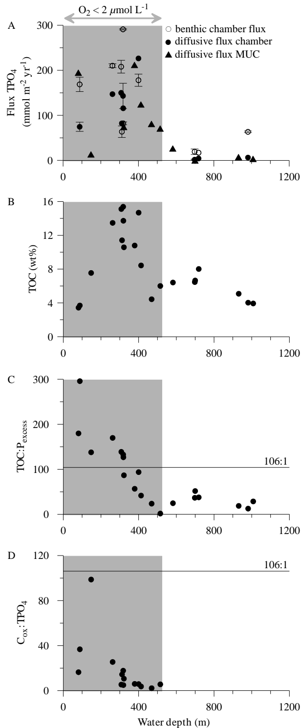
Fig. 2.6: Benthic TPO_4 fluxes and various parameters along the 11^\circ\text{S} transect. (A) Fluxes of dissolved phosphate ( TPO_4 ; \text{mmol m}^{-2} \text{yr}^{-1} ). Error bars correspond to minimum and maximum values of double measurements in lander deployments. (B) TOC contents (wt%) in surface sediments (0-1 cm). (C) TOC:P_{\text{excess}} ratios in surface sediments (0-1 cm). The black horizontal line depicts the TOC:P Redfield ratio of 106:1. (D) C_{\text{ox}}:TPO_4 flux ratios. The black horizontal line depicts the C:P Redfield ratio of 106:1. The gray array in each panel represents the OMZ where O_2 concentrations were < 2 \mu\text{mol L}^{-1} .
