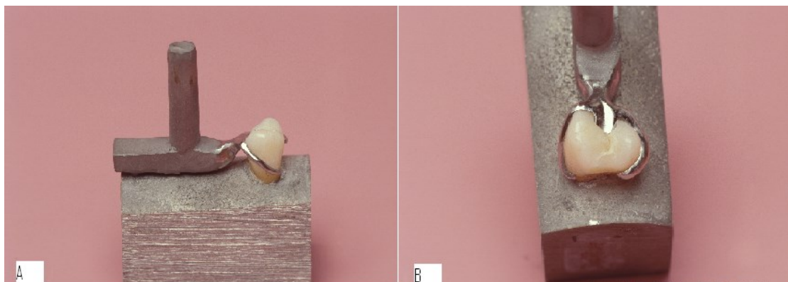
Fig. 8. Framework of E-clasp within the testing model, (A) lateral view and (B) frontal view.
