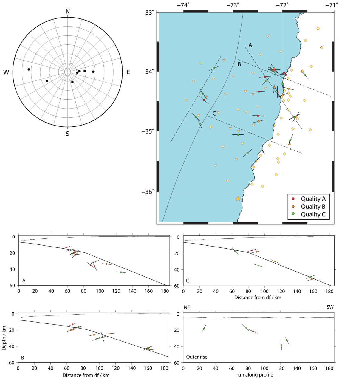
Figure 7.9.: Azimuth and plunge of maximum compressive stress axes (P). Map: colour coded by quality class of focal mechanisms. Plunges were rotated into the cross-section plane. df = deformation front, yellow star = location of Maule main shock, yellow triangles and diamonds = OBS and land station locations, respectively. Polar projection: only axes from focal mechanisms of class A, excluding outer rise events. No vertical exaggeration in cross-sections.
