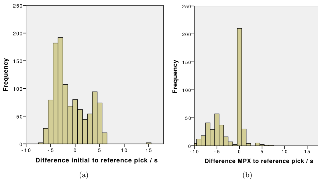
Figure 4.3.: Histograms of differences between initial to reference pick (a), and automatic to reference pick (b).
