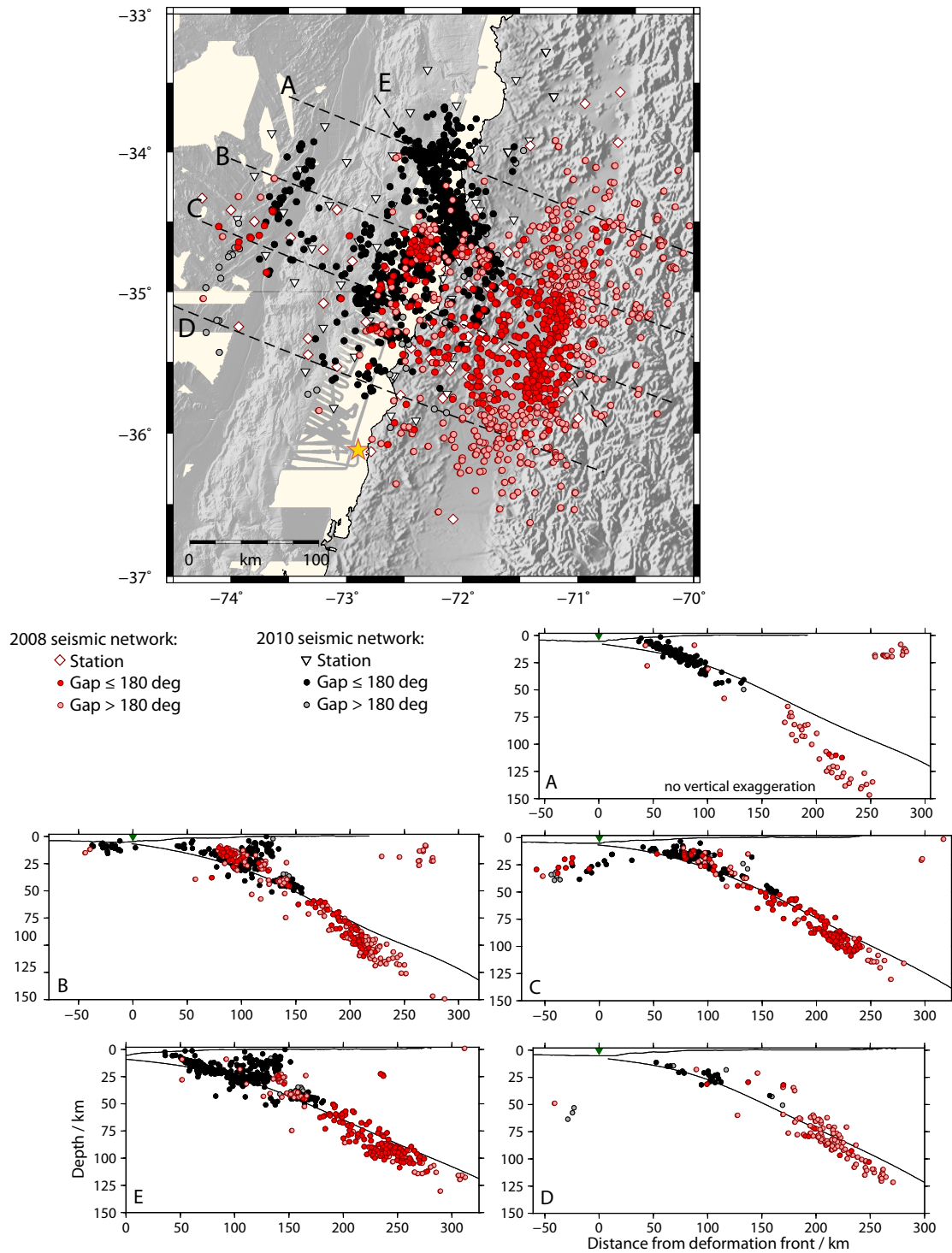
Figure 8.2.: Comparison between the seismic distributions derived from the seismic networks of 2008 and 2010, with quality classes A-C. Events within the network (gap < 180°) are displayed in opaque colours.
