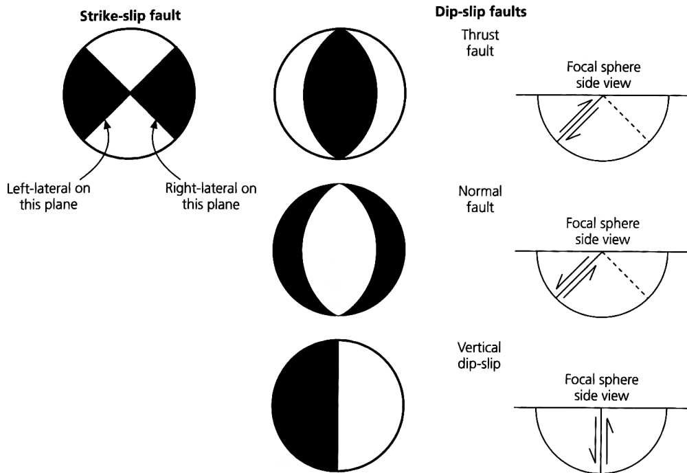
Figure 5.6.: Basis fault geometries and focal mechanisms. Black = compressional first-motions (Stein and Wysession (2009)). Copyright by 2003 by S. Stein and M. Wysession.
