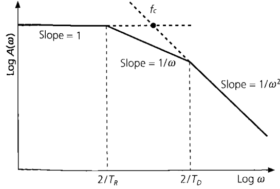
Figure 5.3.: Theoretical source spectrum of an event. From the flat part of the spectrum M_0 can be determined. For a detailed explanation see text. (Stein and Wysession, 2009). Copyright by 2003 by S. Stein and M. Wysession.
