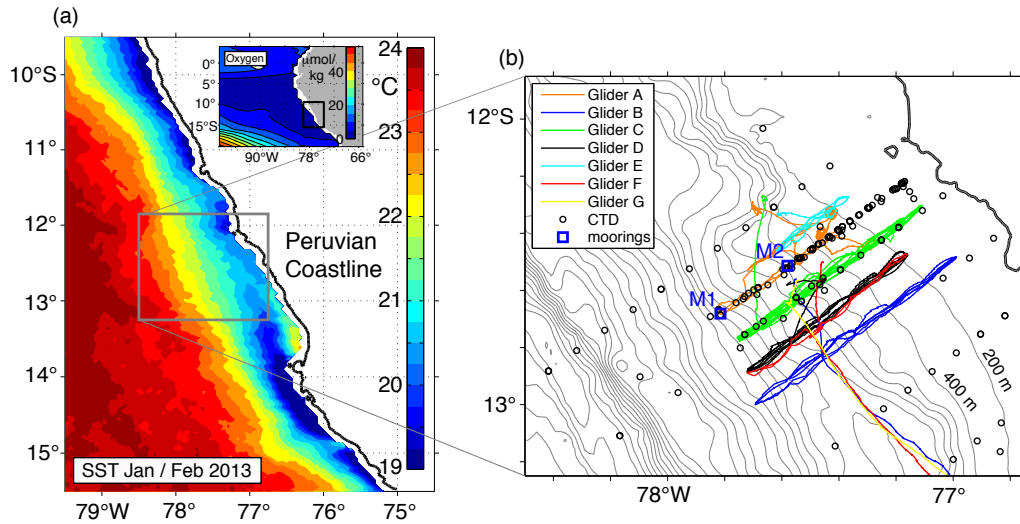
Figure 12: Mean sea surface temperature off Peru during January and February 2013 from remote sensing (Modis Aqua/Terra) is color shaded (a, large panel). The small inlet shows oxygen concentration in \mu\text{mol/kg} in the eastern tropical Pacific at \sigma_\theta = 26.8 \text{ kg/m}^3 as obtained from the MIMOC climatology ( Schmidtke et al., 2013 ) (a, small inlet). The right panel (b) shows the water depth (grey contours, 200 m interval), glider tracks (colored lines), conductivity temperature and depth (CTD) stations (black circles) and the two mooring positions (blue squares).
