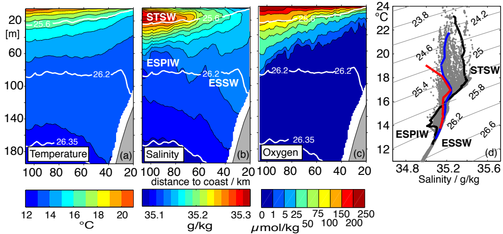
Figure 14: Mean conservative temperature in ^{\circ}\text{C} (a), absolute salinity in g/kg (b) and dissolved oxygen (nonlinear color scale) in \mu\text{mol/kg} (c) distributions near 12^{\circ}30'S between January 10 and February 27 measured by glider C (Fig. 12b). Twelve transects have been horizontally smoothed on a 1 km grid by a rectangular 5 km running mean window and subsequently temporally averaged. Isopycnals are contoured in white. All CTD measurements are shown with grey dots in the T/S diagram (d). The following water masses: Subtropical Surface Water (STSW), Eastern South Pacific Intermediate Water (ESPIW) and Equatorial Subsurface Water (ESSW) are marked in (b) and (d). Three representative glider profiles (offshore (black), (blue) and upper shelf (red)) are overlaid and can be found in the transect in Figure 21h.
