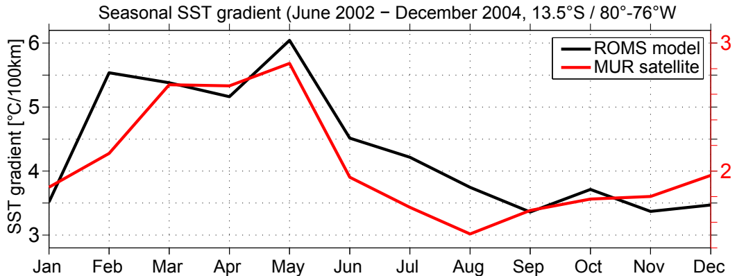
Figure 11: Seasonal cycle of magnitude of SST gradient ( |\nabla SST| = ((\partial SST/\partial x)^2 + (\partial SST/\partial y)^2)^{1/2} ) in ROMS model (black) and Multi-scale Ultra-high Resolution (MUR) satellite observations (red) averaged along a line at 13.5°S between 80° - 76°W. Note the different scales of the y-axis.
