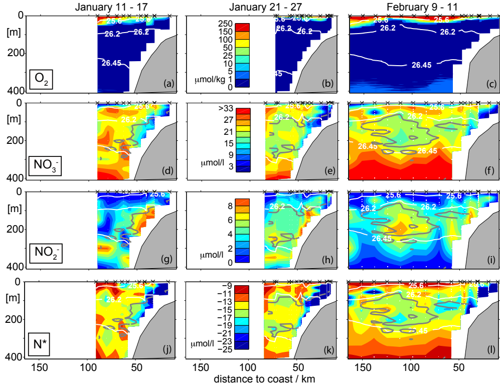
Figure 25: Oxygen in \mu\text{mol/kg} (1st row), nitrate ( NO_3^- ) in \mu\text{mol/l} (2nd row), nitrite ( NO_2^- ) in \mu\text{mol/l} (3rd row), nitrogen-deficit ( N^* = (NO_3^- + NO_2^-) - 16PO_4^{3-} ) in \mu\text{mol/l} (4th row) at three different time periods: prior to the eddy formation (left column, January 11 - 17), during the eddy formation (middle column, January 21 - 27) and when the eddy is fully developed (February 9 - 11). The positions of the nutrient measurements are marked with green dots in Figure 15a,g,m. The white dots indicate position of the nutrient measurements. The grey line shows the fPV = 1.1 \cdot 10^{-14} \text{ 1/s}^4 contour.
