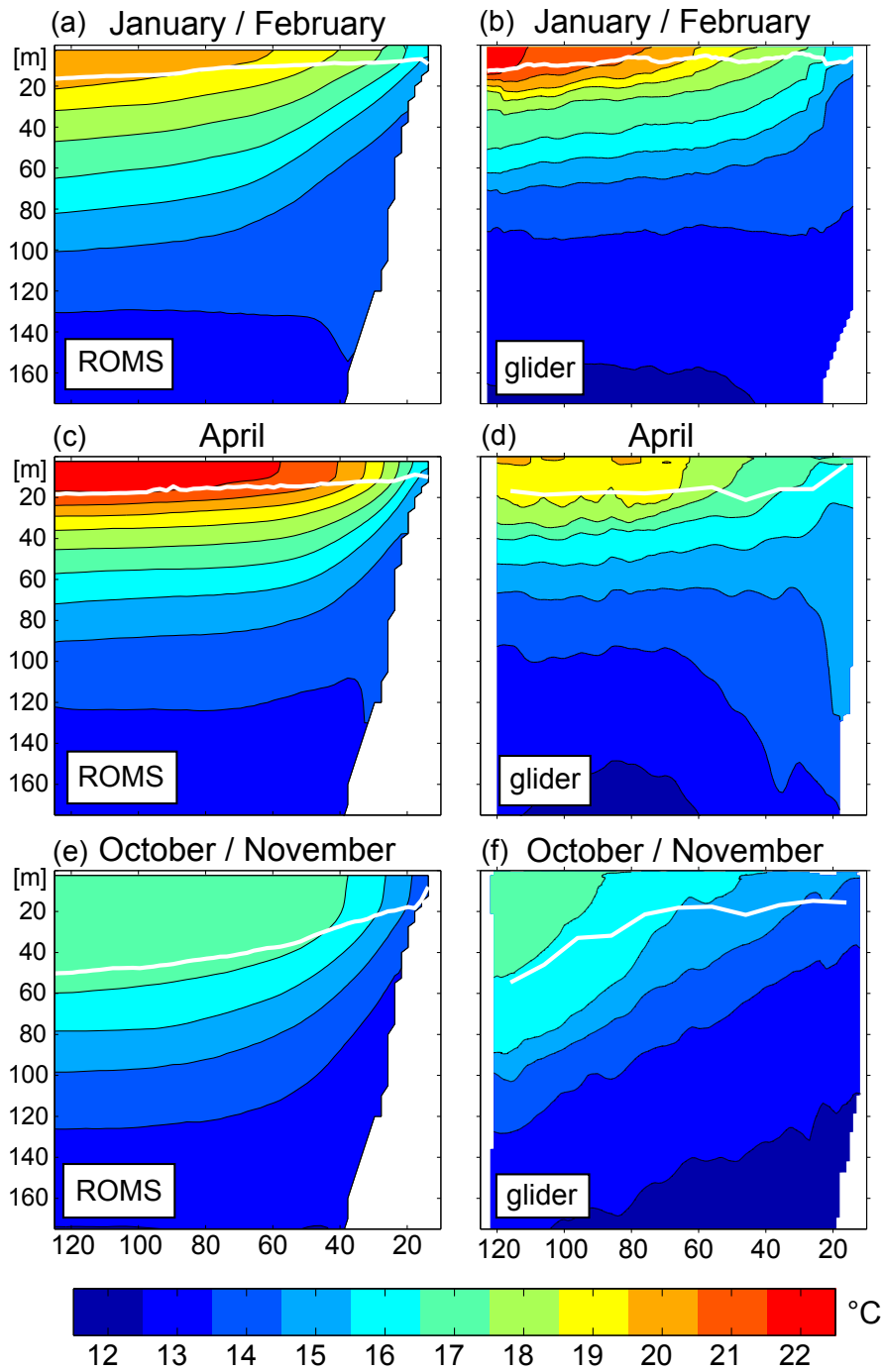
Figure 9: Average vertical temperature distribution along 14^{\circ}\text{S} off Peru ROMS model simulation (left) and from glider observations (right) in January / February (top), April (middle) and October / November (below). The mixed layer depth, defined here as the depth where the surface temperature minus 0.2^{\circ}\text{C} is found, is shown as a white line.
