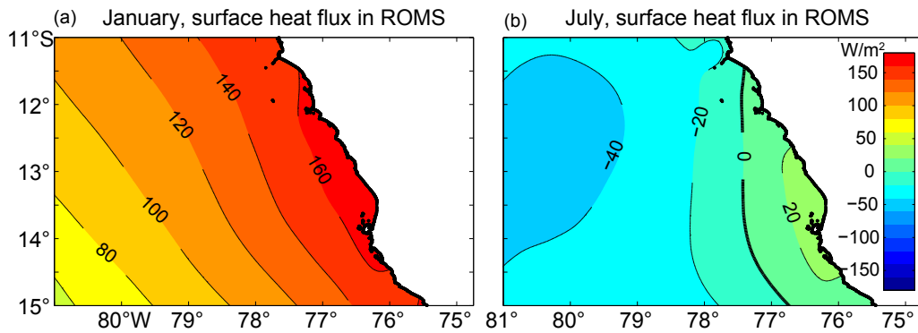
Figure 8: Surface heat fluxes in ROMS simulation in January (left) and July (right) in \text{W/m}^2 .
