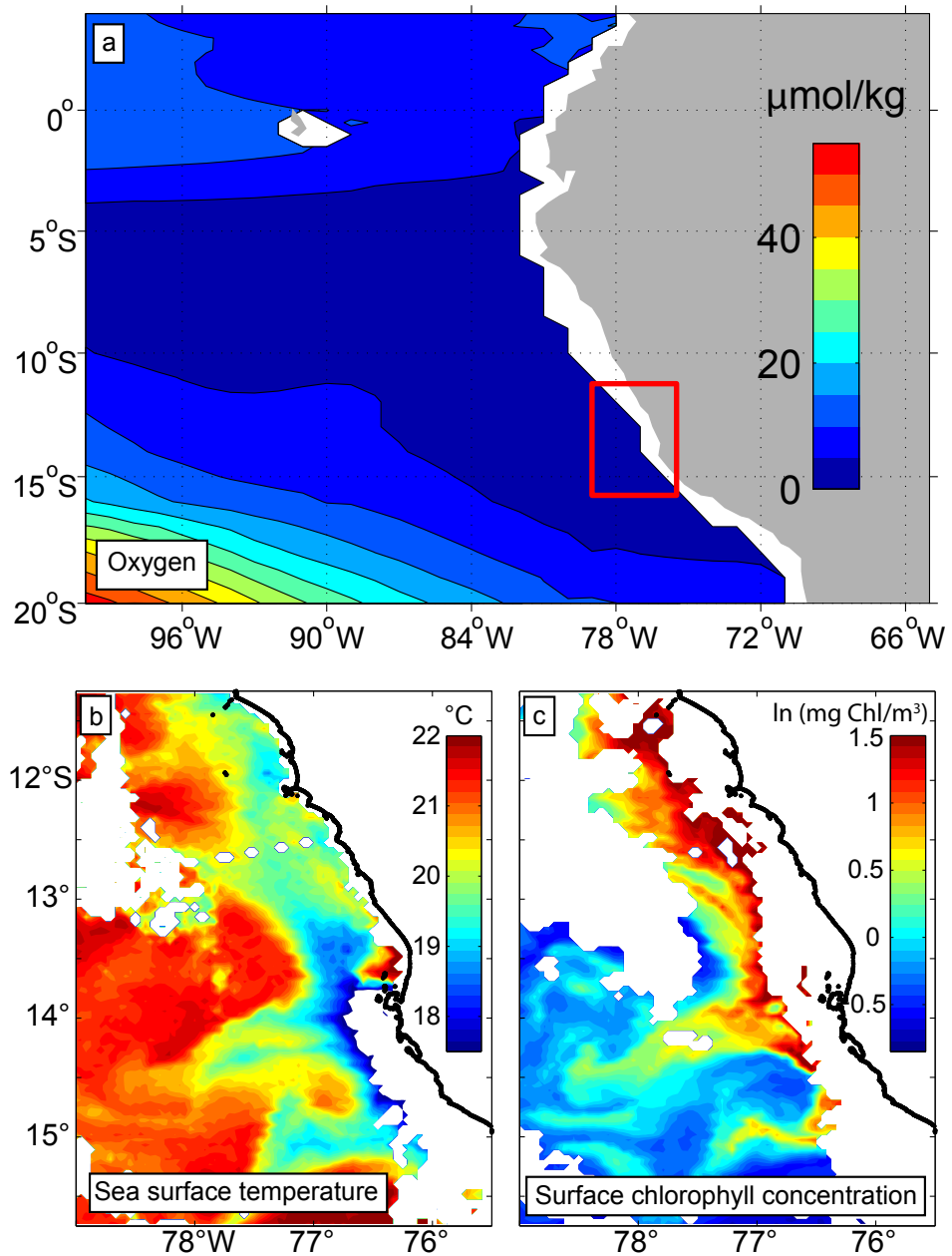
Figure 1: Oxygen concentration (a) in \mu\text{mol/kg} in the eastern tropical Pacific at \sigma_{\theta} = 26.8 \text{ kg/m}^3 as obtained from the MIMOC climatology (Schmidtke et al. , 2013). The red square indicates the region shown in (b) and (c), which represent the study area of this thesis. Sea surface temperature in ^{\circ}\text{C} (b) and surface chlorophyll concentrations (c) in logarithmic form (of unit \text{mg/m}^3 ) from MODIS Aqua satellite measurements on January 25 2013 off Peru.
