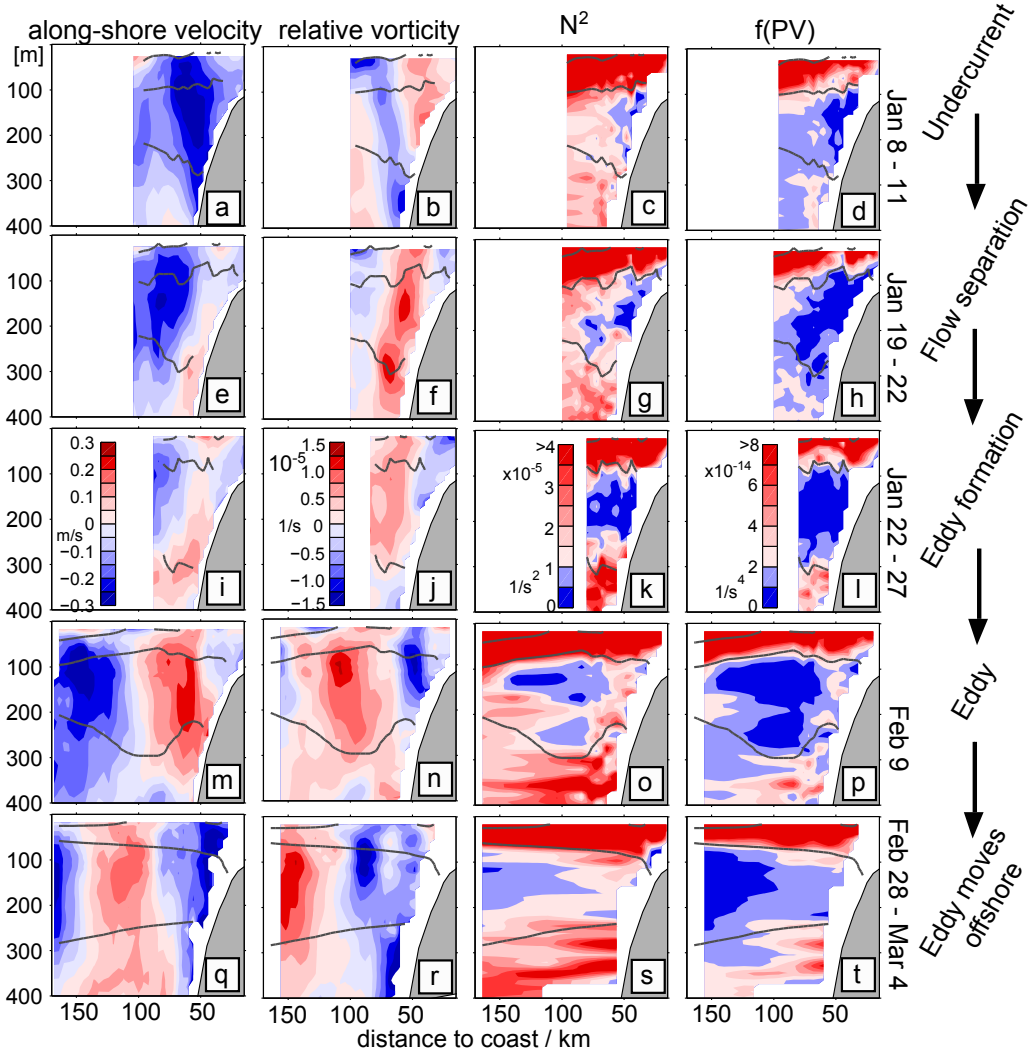
Figure 16: The first column shows the alongshore velocity ( v_{\text{ADPC}} ) in m/s where positive/negative values correspond to equatorward/poleward (into/out of the page) flow. The second column shows the two-dimensional relative vertical vorticity ( \zeta^z = \partial v / \partial x , where v is the alongshore velocity and x points towards the coast). The third column shows the stratification ( N^2 = -(g/\rho_0) \cdot (\partial \rho / \partial z) - (g/c_s)^2 , with g being the gravitational acceleration, \rho the potential density, \rho_0 a reference density and c_s the sound speed). The last column shows the PV times f , with PV = N^2(f + \partial v / \partial x) . Isopycnals (25.6, 26.2 and 26.45) are contoured in grey. All transects go along the main transects as marked with grey in the left column of Fig. 15. Only the last transect is slightly further north of the main transect to be closer to the eddy core (dashed grey line in Fig. 15s.)
