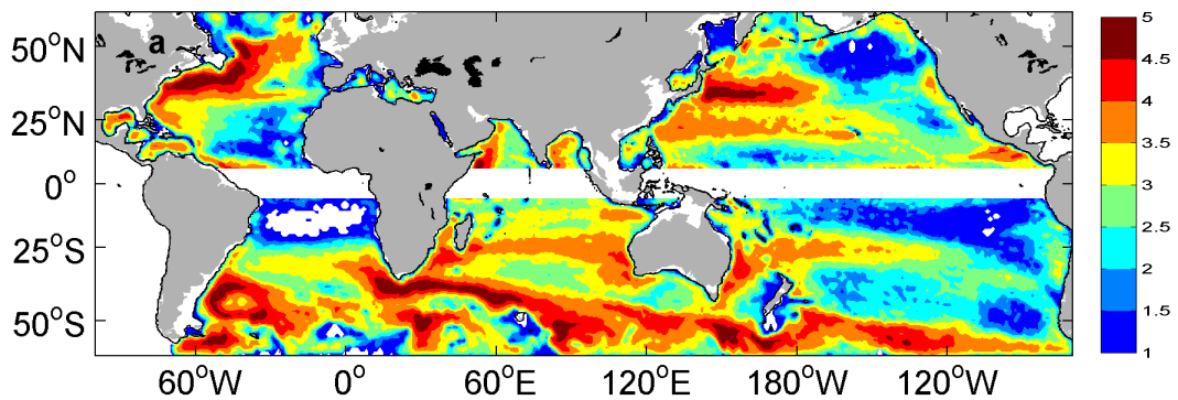
Figure 2: Global horizontal distribution of mean eddy kinetic energy in logarithmic form (of unit \text{J}/\text{m}^2 ) based on altimeter data available by the AVISO Altimetry Operations Center. Figure is taken from (Xu et al. , 2014)
