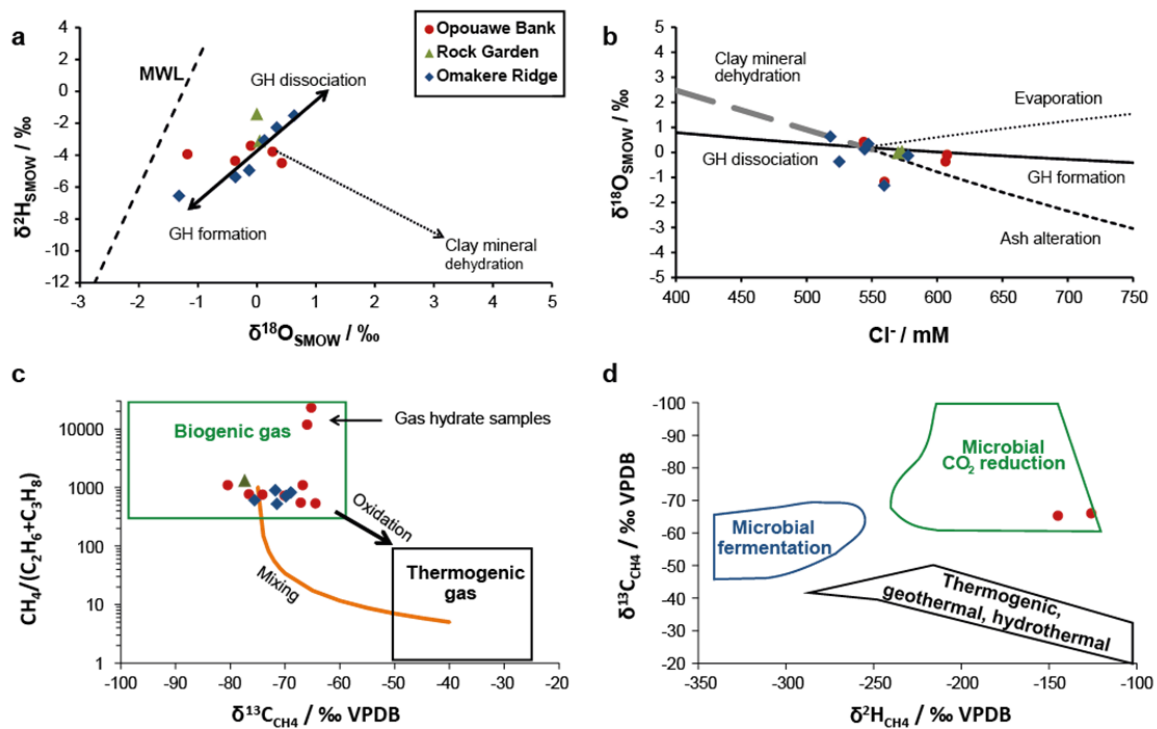
Figure 2.4: Geochemical characterization of the porefluid and gas composition as well as gas hydrates in surface sediments of cold seeps at the Hikurangi margin (Opoouawe Bank, Rock Garden, and Omakere Ridge). a Porewater isotopic composition and typical trends from gas hydrate formation and dissociation (solid line), clay mineral dehydration (dotted line), and meteoric water mixing (dashed line; MWL meteoric water line). b Porewater oxygen isotopes versus chloride concentration, and influences from typical diagenetic processes. c Bernard plot indicating the biogenic or thermogenic origin of the gas. For comparison, the theoretical mixing line between biogenic and thermogenic methane as well as the trend for oxidation are indicated. d Isotopic composition of methane in the recovered gas hydrate pieces from the Takahe seep, and process-related fields (according to Whiticar et al. 1986).
