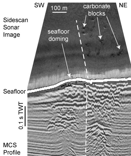
Figure 4.4: Combined view of sidescan sonar and multichannel seismic (MCS) data for Pukeko seep site (offshore New Zealand). Seafloor backscatter map of sidescan sonar shows distribution of seep carbonates which cause high backscatter (black) due to high impedance contrast and surface roughness. MCS data show that subsurface seep structure consists of two parts, with seafloor doming over western part and carbonate precipitation over eastern part.
