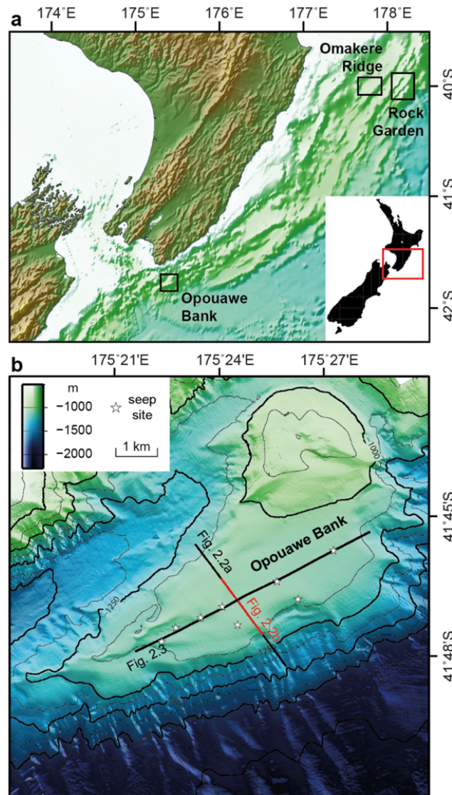
Figure 2.1: a Overview of the study area offshore New Zealand, with Opuawe Bank, Omakere Ridge, and Rock Garden. Geochemical analyses were carried out on material from a gravity corer and video-guided multiple corer in all three areas (for locations, see Table A.1 in the Appendix A.1). b Bathymetric map of Opuawe Bank, displaying the locations of the seep sites. The marked profiles are the 2D Nemesys line (Fig. 2.3), a segment of the 2D Pegasus line (Pegasus_19, Fig. 2.2a), and a section from the 3D P-Cable Cube (Fig. 2.2b).
