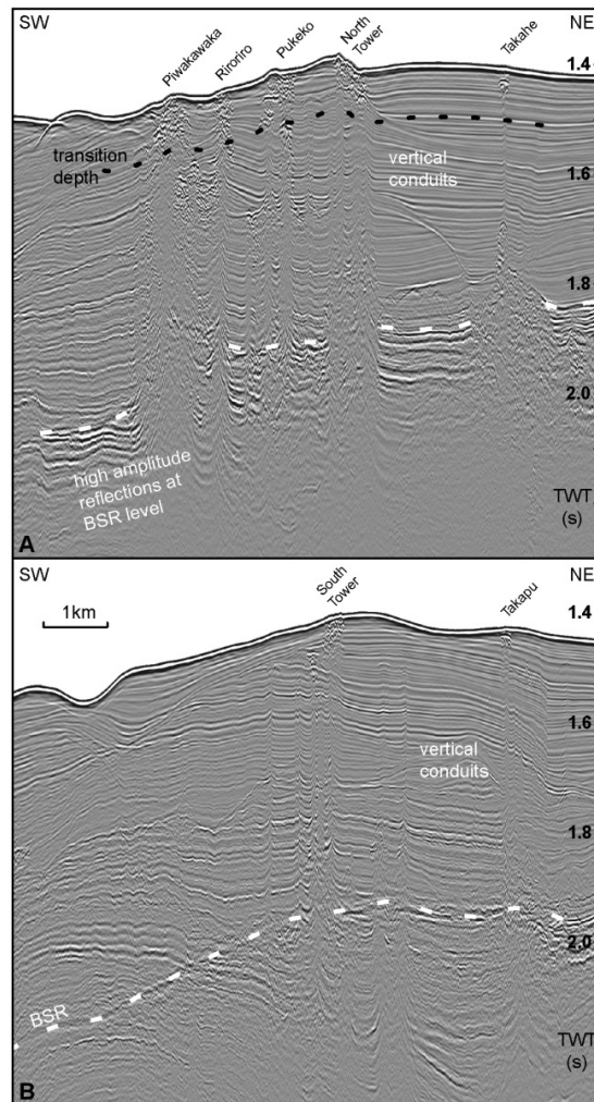
Figure 3.2: A) Northern and B) southern 2D seismic line along the main seep sites on Opuawe Bank, displaying the gas migration pathways through the accretionary ridge. These pathways appear as vertical conduits of limited extend on the 2D seismic. However, Figure 3.3 displays their spatial structure to be elongated across the ridge. Marked as dashed black line is the depth, where the gas migration structures transform to pipe-like structures.
