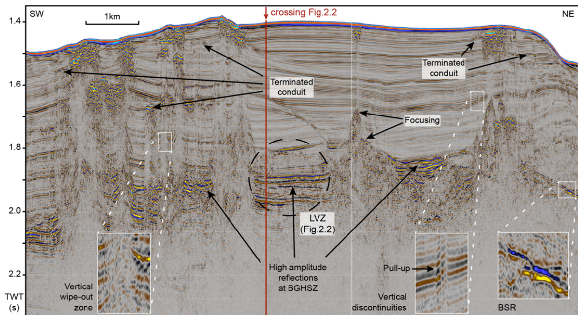
Figure 2.3: 2D Nemesys line along the Opoouawe Bank crossing the seep structures aligned along the ridge. The vertical conduits display several focusing levels, and some conduits terminate within the sediments. The interface of Figs. 2.2 and 2.3 illustrates the spatial distribution of the high-amplitude reflections at the base of the gas hydrate stability zone (BGHSZ), where the LVZ is located.
