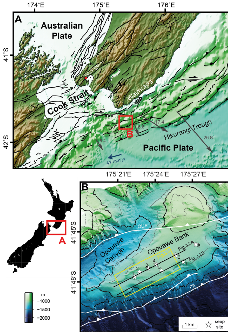
Figure 3.1: A) Bathymetric map showing the location of Opouawe Bank at the Hikurangi margin, offshore New Zealand. Geological structures are from Wallace et al. (2010). Blue arrow shows the relative plate motion vector of the Australian and Pacific plates at the southern North Island, with most of the margin normal component of the plate motion occurring on the subduction thrust and the margin parallel component as a combination of strike-slip faulting and forearc rotation (Wallace et al., 2010 and references therein). Gray arrows display the modeled relative motion (in mm/yr) between tectonic block boundaries in the east and the Pacific plate (Wallace, 2012). BBF = Boo Boo Fault; OUF = Opouawe-Uruti Fault; PF = Pahaua Fault. (B) Location of seep sites (white stars) on Opouawe Bank investigated in this study 1 = Piwakawaka; 2 = Riroriro; 3 = Pukeko; 4 = North Tower; 5 = South Tower; 6 = Takahe; 7 = Takapu; 8 = Piwakawaka. The yellow rectangle displays the outline of the 3D seismic volume (Fig. 3.3) and the black lines indicate the location of the 2D MCS data (Fig. 3.2).
