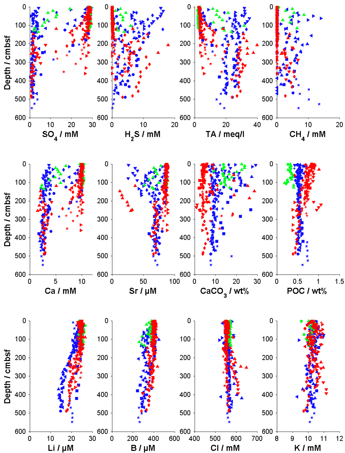
Figure A.1: Concentration-depth profiles of various dissolved porewater and solid phase species from gravity cores taken at various seep sites (different symbols) in the investigation areas (green: Rock Garden; blue: Omakere Ridge; red: Opouawe Bank) along the Hikurangi Margin (see Tab. A.1 for details).
