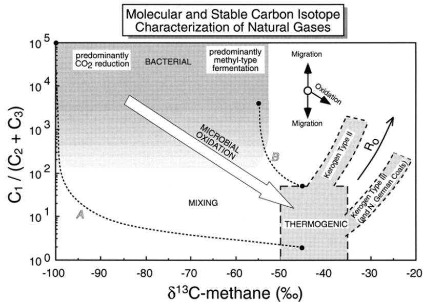
Figure 1.6: Bernard diagram (from Whiticar, 1999) combining the molecular ( C_1/(C_2 + C_3) ) and isotopic ( \delta^{13}\text{C} ) compositional information and displaying biogenic or thermogenic origin of natural gases or mixing of both. The arrows indicate the relative compositional effects of oxidation or migration.
