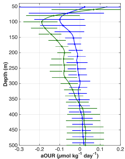
3 Figure 7: Depth profiles of a mean apparent oxygen utilization rate (aOUR, \mu\text{mol kg}^{-1} \text{d}^{-1} ) within CEs (blue) and 4 ACMEs (green) with associated standard deviation (horizontal lines).
