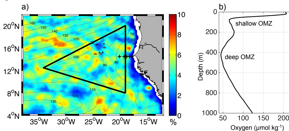
2 3 4 Figure 1: a) Map of the ETNA including contour lines of the oxygen minimum of the upper 200m (in \mu\text{mol kg}^{-1} ) as obtained from the MIMOC climatology (Schmidtko et al., 2013). The color indicates the percentage of 5 6 "dead-zone" eddy coverage per year. The black triangle defines the SOMZ. The black crosses indicate the 7 position of the CTD stations of the research cruise M97, which are used to represent the vertical oxygen profile 8 shown on the right. b) mean vertical oxygen profile showing the shallow oxygen minimum centered around 80 9 m depths and the deep oxygen minimum centered at 450 m depth.
