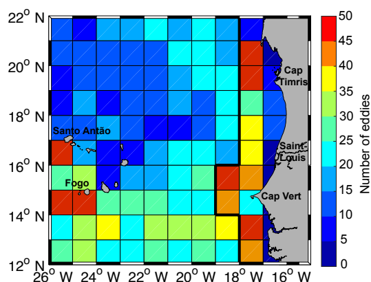
Figure 7. Number of eddies generated in 1^\circ \times 1^\circ boxes (colors) between 1995 and 2013 based on the results of the OW method. Marked are the headlands Cap Timiris (Mauretania), Saint-Louis (Senegal), Cap-Vert (Senegal), and the islands Santo Antão (Cabo Verde) and Fogo (Cabo Verde), which can be associated with high eddy generation. The thick solid black line along 18^\circ W/ 19^\circ W separates the coastal region from the offshore region.
