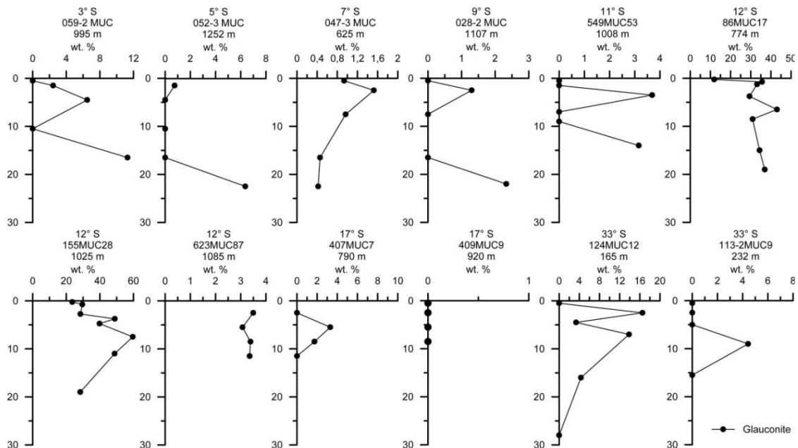
Fig. 4.4 Sedimentary glauconite content (wt. %) determined by XRD analyses for selected sediment cores from 3 to 33°S. Note that the scales are adapted to the glauconite content for better visualization.
