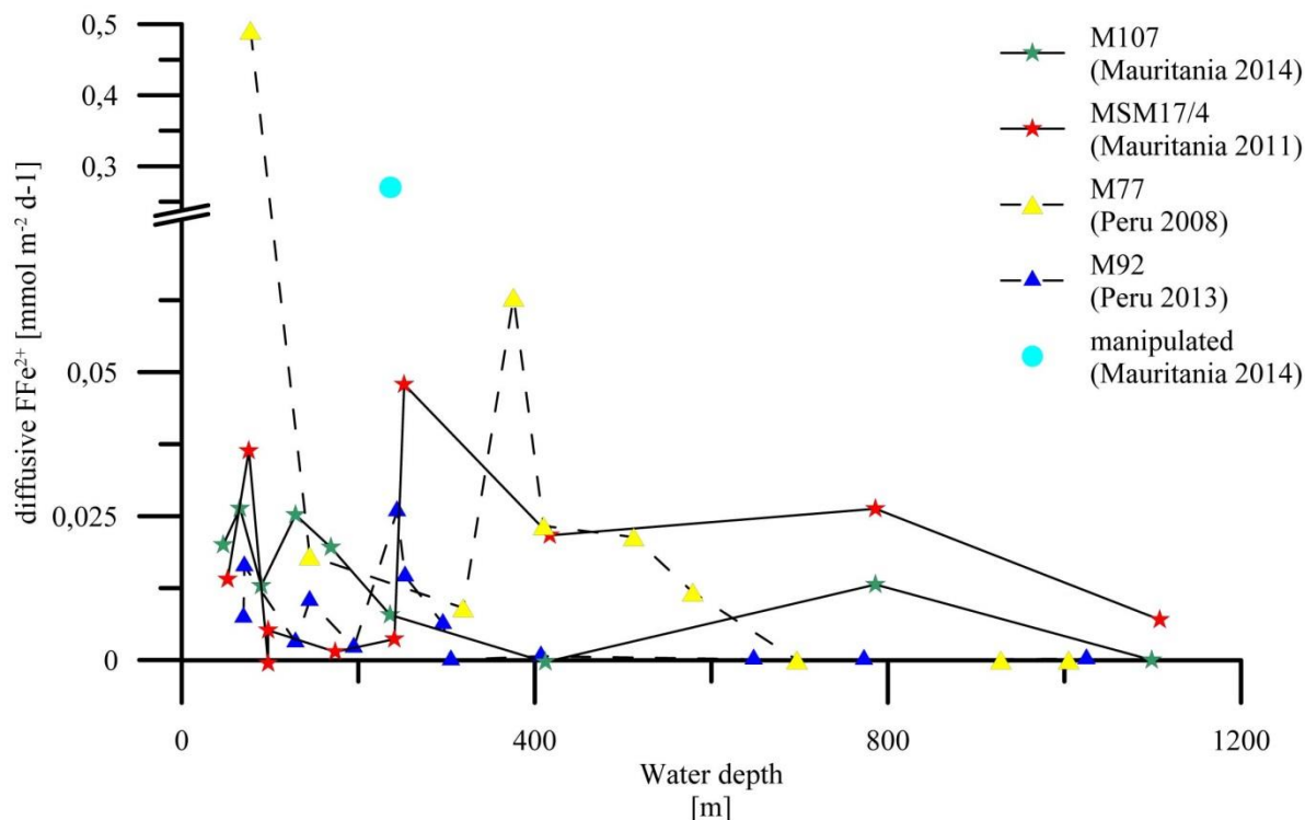
Fig. 3.9 Datasets of diffusive \text{Fe}^{2+} fluxes ( \text{mmol m}^{-2} \text{d}^{-1} ) from the Mauritanian Upwelling (MSM17/4 and M107) along the 18^\circ\text{N} depth transect and from the Peruvian Upwelling (M77 and M92) along 11 and 12^\circ\text{S} depths transects. The single blue dot denotes the Fe release determined from the \text{O}_2 manipulation experiments.
