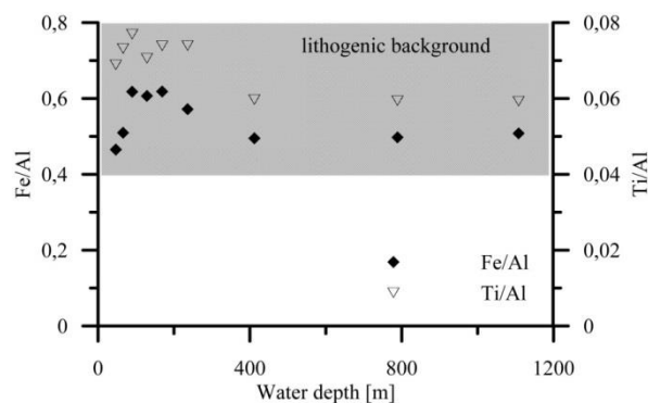
Fig. 3.4 Mean Fe/Al and Ti/Al ratios against water depth. The grey shaded area indicates the lithogenic background ratio for Fe/Al. Ti/Al indicate grain size changes along the depth transect.
