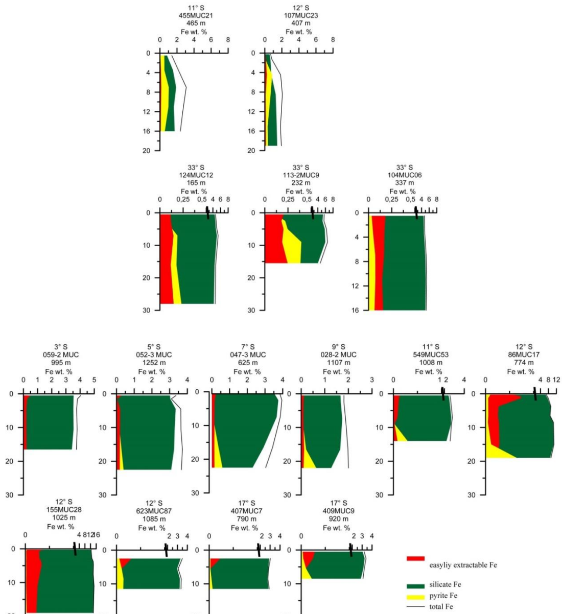
Fig. 4.3 Distribution of sedimentary Fe species (easily extractable Fe, silicate Fe and pyrite Fe) and total Fe with sediment depth. The upper two rows show Fe species in sediments retrieved within the OMZ ( O_2 ranging from 0 to 18 \mu\text{M} ) at 11, 12 and 33°S. The lower rows show selected cores between 3 and 33°S retrieved below the lower oxycline of the OMZ at bottom water oxygen concentrations O_2 > 20 \mu\text{M} .
