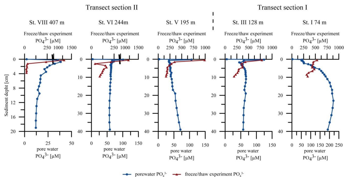
Fig. 2.7 Comparison of pore water \text{PO}_4^{3-} concentrations before (blue) and after the freeze/thaw experiments (red) in \mu\text{mol L}^{-1} .
