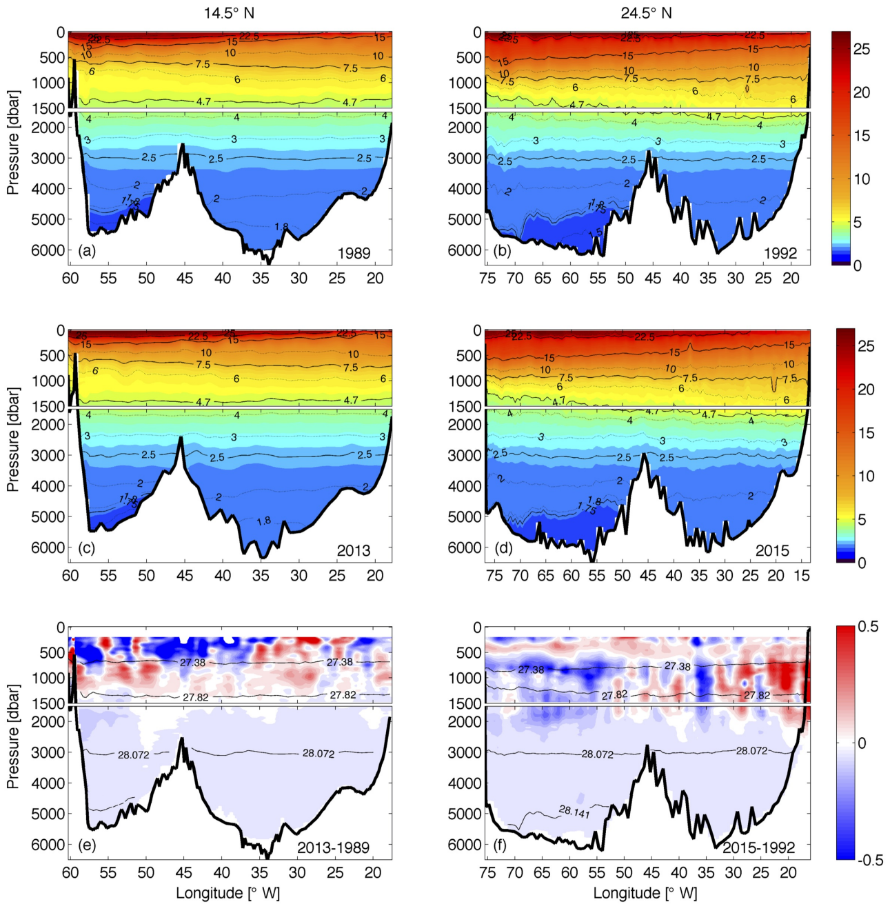
Figure. 3.4 | Vertical sections of potential temperature ( ^{\circ}\text{C} ) at 14.5^{\circ}\text{N} in (a) 1989 and (c) 2013; and at 24.5^{\circ}\text{N} in (b) 1992, (d) 2015. Further shown is the potential temperature difference at (e) 14.5^{\circ}\text{N} between 2013 and 1989; and (f) 24.5^{\circ}\text{N} between 2015 and 1992. Note that the difference is calculated first on neutral density levels, then transformed back to depth levels, and that the upper 200 m are neglected. The contours in (e) and (f) are the neutral density surfaces of 27.38, 27.82, 28.072, and 28.141 \text{kg m}^{-3} , which marks the boundaries of AAIW, UNADW, LNADW, and AABW. The upper 1500 m in each subplot are stretched.
