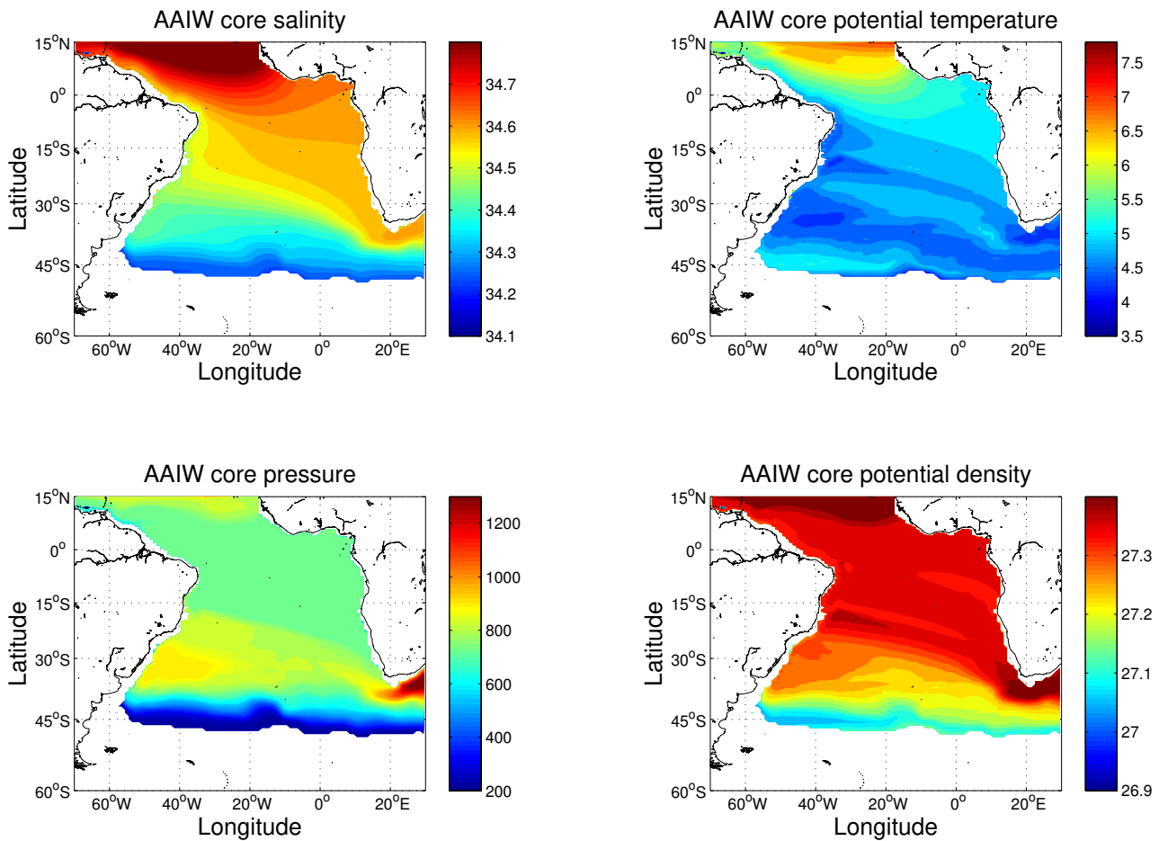
Figure. 4.1 | Climatology of the salinity, potential temperature, pressure, and potential density at the AAIW core, estimated from GECCO2.
