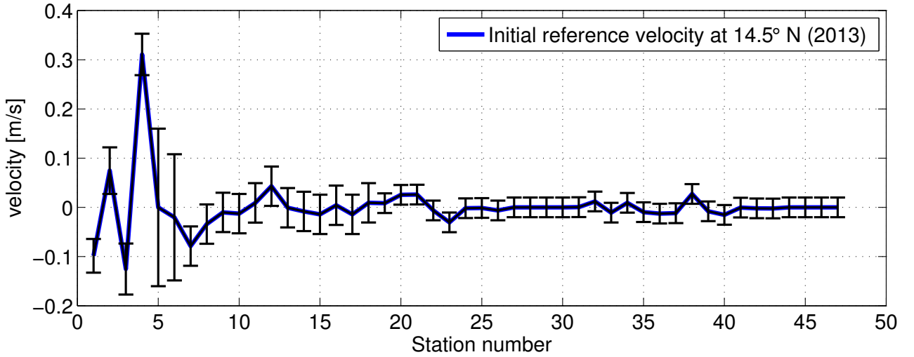
Figure. 3.7 | Initial reference velocity with error bars for the 2013 realization at 14.5° N, estimated from a combination of SADCP and LADCP (see text for details).
