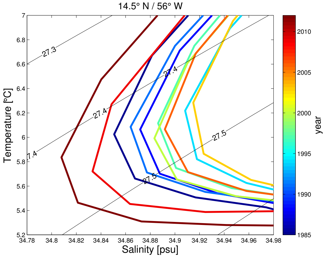
Figure. 4.2 | Annual mean \theta/S diagram focusing on the salinity minimum at 14.5^\circ \text{ N}/56^\circ \text{ W} in GECCO2, plotted every 3rd year from 1985. The years are marked with different colours.
