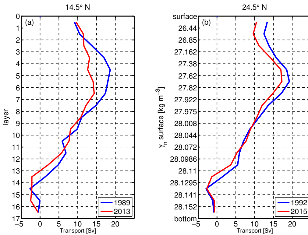
Figure. 3.11 | Meridional overturning stream function from the inverse model at (a) 14.5° N and (b) 24.5° N. It is calculated by cumulatively integrating the layer transport from the surface to the bottom. The vertical coordinate in (a) is the layer number, and in (b) the corresponding neutral density surface. For the 14.5° N section, the blue curve stands for the 1989 realization, the red curve for the 2013 realization. For the 24.5° N section, the blue curve stands for the 1992 realization, and red curve for the 2015 realization.
