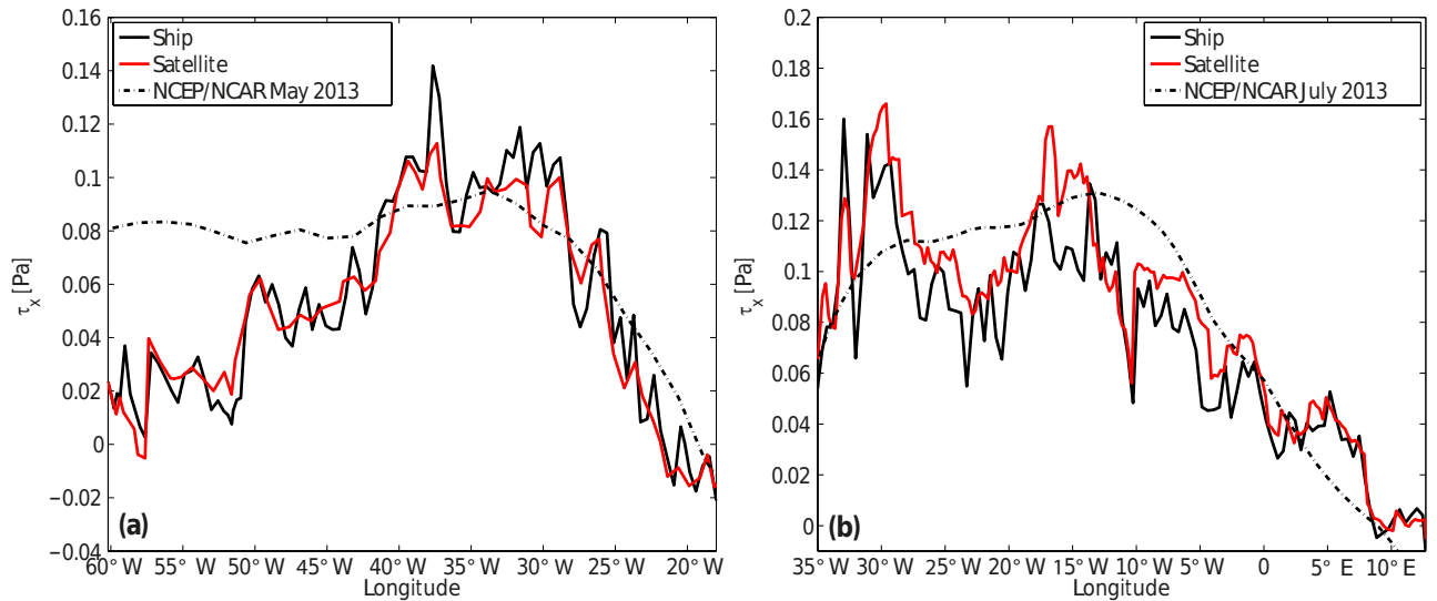
Figure. 2.5 | Zonal wind stress along (a) 14.5° N and (b) 11° S. Ship wind stress (black line) was binned in a 50 km interval. The satellite wind stress data (red) were extracted to the nearest ship time and position. The NCEP reanalysis monthly zonal wind stress (black dashed line) at the same latitude in the cruise month is also plotted.
