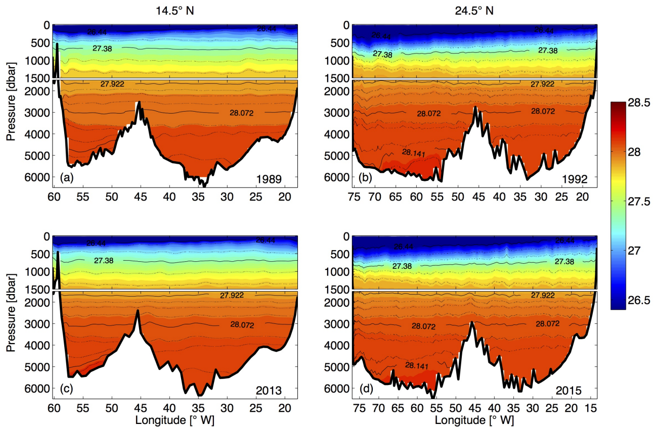
Figure. 3.6 | Vertical sections of neutral density ( \text{kg m}^{-3} ) at 14.5^\circ \text{N} in (a) 1989 and (c) 2013; and at 24.5^\circ \text{N} in (b) 1992 and (d) 2015. The upper 1500 m in each subplot are stretched.
