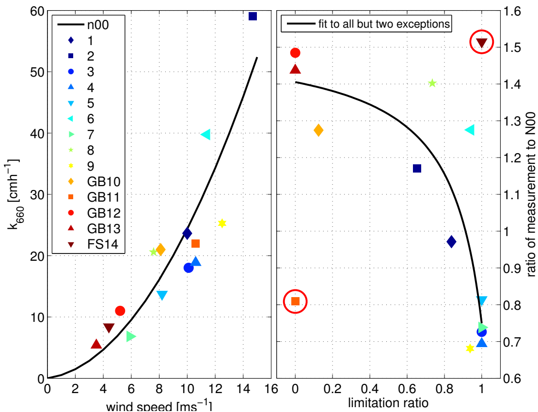
Figure 5.4: Individual dual tracer measurements which contribute to the N00 (solid line) parameterization [left panel]. The relationship of the gas limitation ratio to the measurement/N00 ratio [right panel]. A higher limitation ratio indicates a longer influence of gas transfer limitation on the data point. The solid line in the right panel is a fit to the limitation to measurement/N00 relationship. The two red circles denote the outlier points which are discussed in the text. The black solid line is a fit using the function y(x) = a_1 + a_2 \cdot \frac{1}{x-a_3} . The fit coefficients are: a_1=1.52 , a_2=0.14 and a_3=1.18 .
