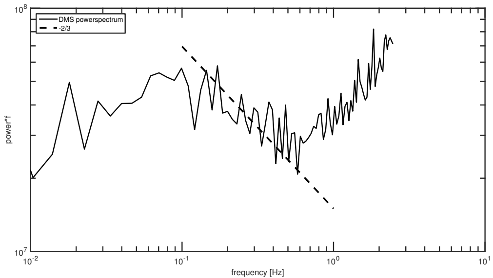
Figure 4.19: A sample power spectrum of the DMS concentration, recorded for 30 minutes. The dashed line is a reference to the -\frac{2}{3} decay in the inertial subrange [Kolmogorov, 1941]. The increase after 1 Hz illustrates noise from the high frequency tubing loss and the instruments measurements.
