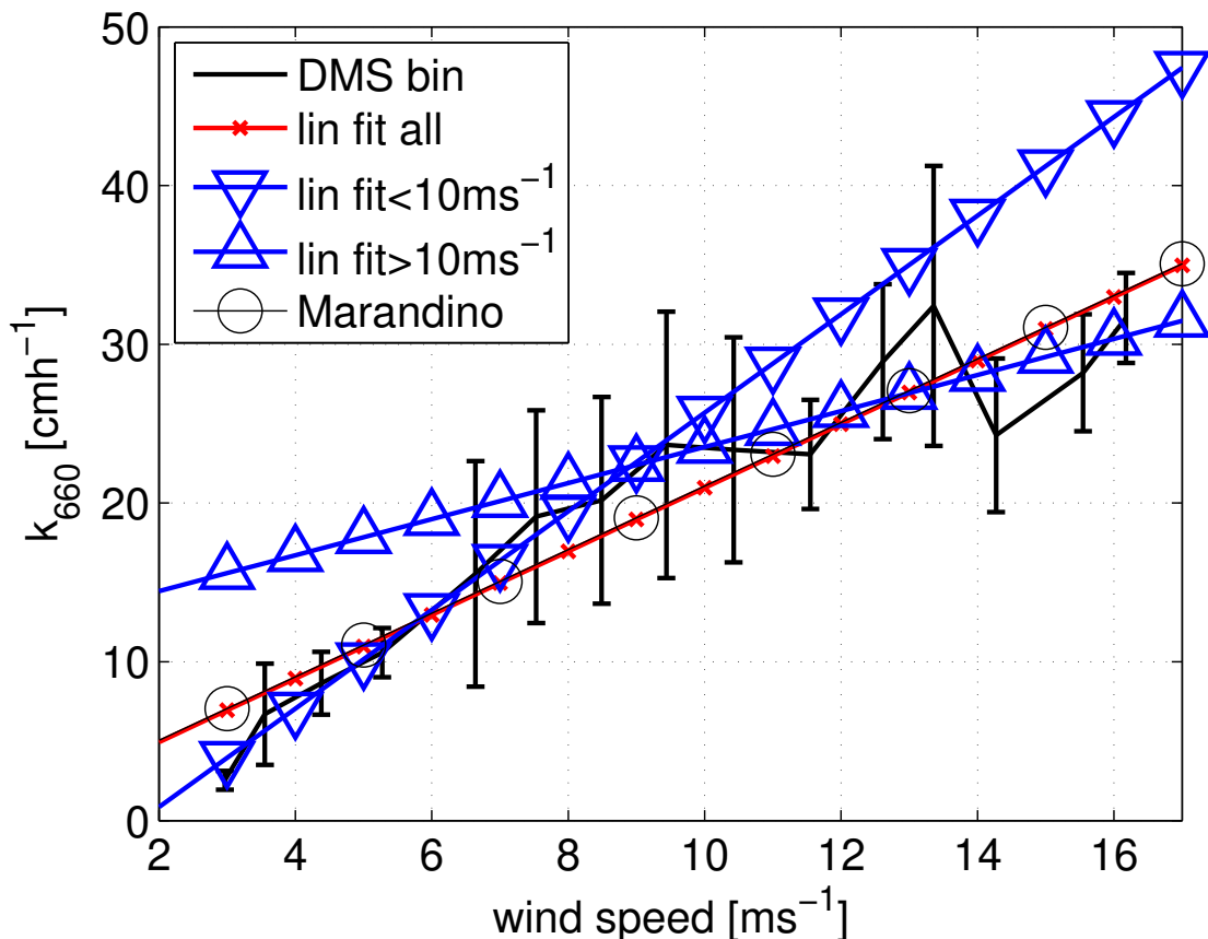
Figure 4.7: Binned (size 1 \text{ ms}^{-1} ) DMS gas transfer velocities and linear fits of the binned data below 10 \text{ m s}^{-1} and above 10 \text{ m s}^{-1} . An overall fit and the linear parameterization, updated from Marandino et al. [2009], is added.
