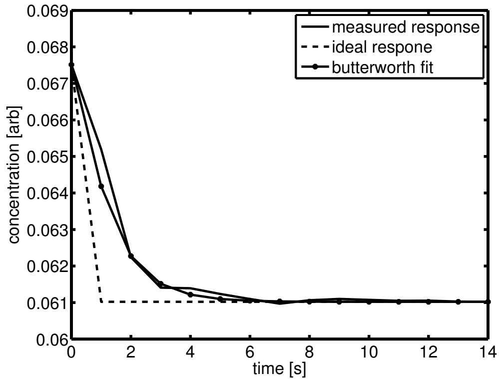
Figure 4.17: The concentration of the isotopically labeled reference gas during a valve switch. We applied and tuned a low-pass filter to an ideal valve switch to match the measured progression. Using the low-pass filter parameters, we accounted for the high frequency loss in the tube.
