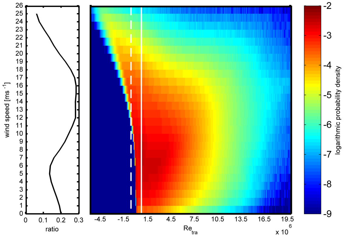
Figure 4.11: We used the global 2014 WWIII data to calculate the transformed Reynolds number. [Right] The global 2014 probability density for the Re_{tra} parameter with respect to wind speed. The limited gas transfer regime is between the dashed and solid white lines. [Left] The ratio of non-limiting (outside the white lines) to limiting (between the white lines) incidents over wind speed.
