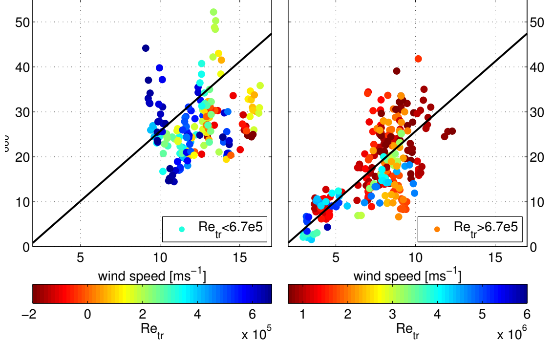
Figure 4.9: Influence of wind-wave interaction on DMS gas transfer. [Left] Limited transfer velocities ( |Re_{tr}| < 6.7 \cdot 10^5 ) measured during SO234-2/235. [Right] Non-limited transfer velocities ( |Re_{tr}| > 6.7 \cdot 10^5 ). For comparison a linear fit through the non-limited transfer velocities is added to both panels. The color shows the transferred Reynolds number Re_{tr} . The colormap is different for the left and the right panel.
