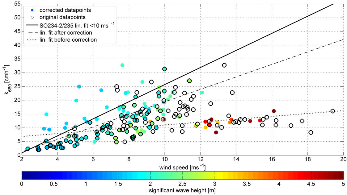
Figure 5.3: Correction of the Knorr11 DMS fluxes. The data points with Re_{tr} < 6.7 \cdot 10^5 were corrected using the gas transfer limitation model. Black circles denote k values at the original wind speed u_{10} . Colored filled circles denote the k value at wind speed =u_{alt} . The color shows the significant wave height. If a data point has a concentric black and filled circle, it was not corrected as it was not subject to gas transfer limitation. The black solid line is the ZAV17 parameterization. The dotted line is the linear fit to the data points before the correction, the dashed line is the linear fit after the correction.
