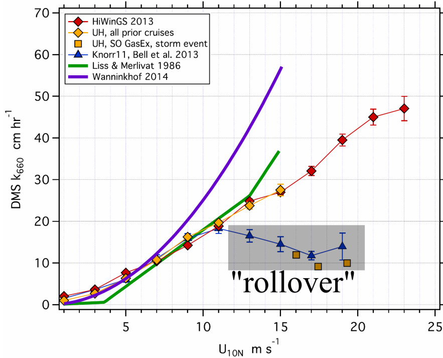
Figure 1.6: Gas transfer velocity measurements with (Knorr11, SO GasEx storm event) and without rolover (all other lines). The data points subject to gas transfer limitation are inside the shaded box. Modified from Blomquist et al. [2017].
