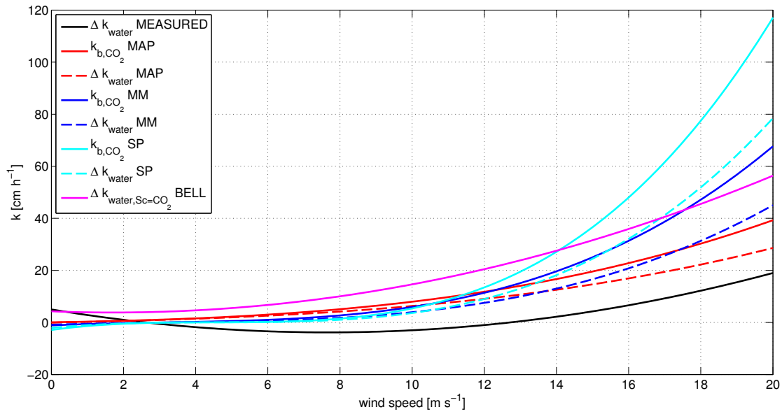
Figure 4.14: Comparison of k_{b,CO_2} and \Delta k_{water} vs wind speed relationships. MAP, MM and SP are calculated by the hybrid model using the three whitecap fraction models. \Delta k_{water, Sc=CO_2} Bell is derived from direct CO 2 and DMS flux measurements by Bell et al. [2017a]. \Delta k_{water} MEASURED is derived from the measurements of this study. The dashed lines represent \Delta k_{water} (Equation 4.18) from the three W models. The difference between the dashed and the equally colored solid line is the modeled k_{b,DMS}
