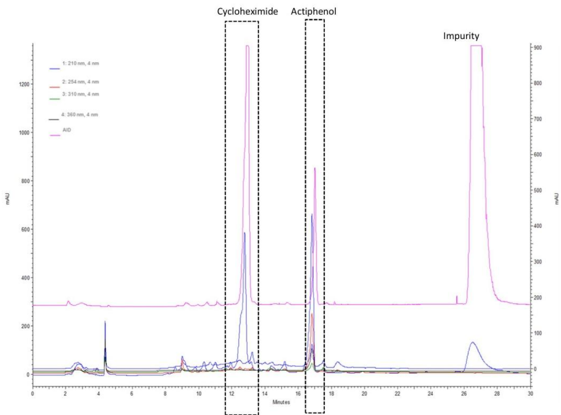
HPLC –ELSD profile of Streptomyces sp. SN25_8.1.
