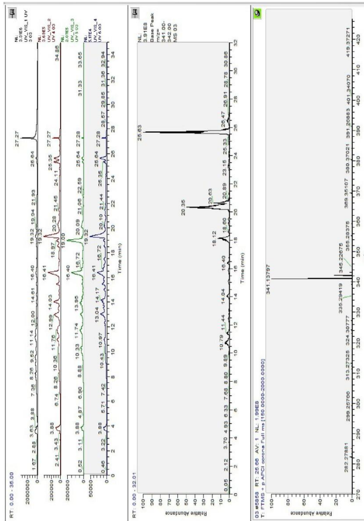
Suppl. Fig. 3. BPC extraction of Lupinacin A (1) (MW: 340) from the crude extract of Verrucosipora sp. SN26_14.1 isolated from the Easter Island sea anemone, Gyactis sesere .
