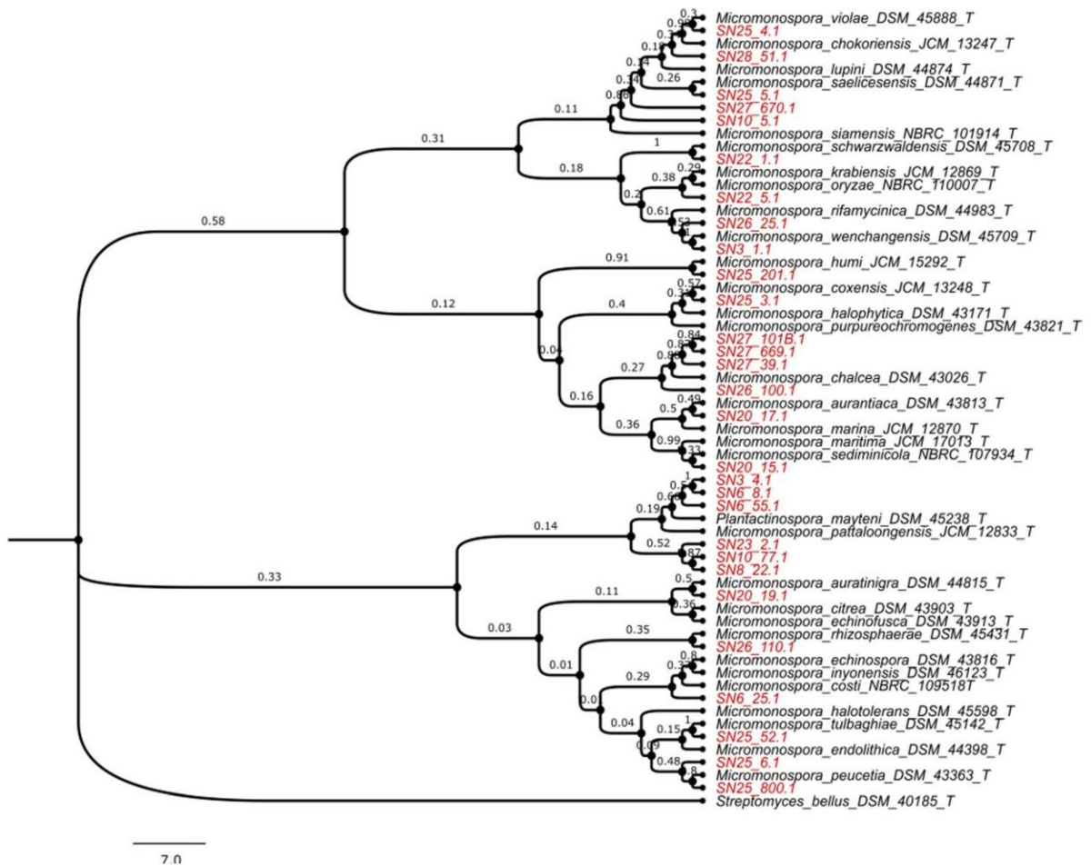
Fig. 3 Phylogenetic analysis of Micromonospora sp. isolates and Micromonospora sp. type strains by maximum likelihood method based on the Kimura 2-parameter model. Bootstrap: 1000 replicates. Red letters:
