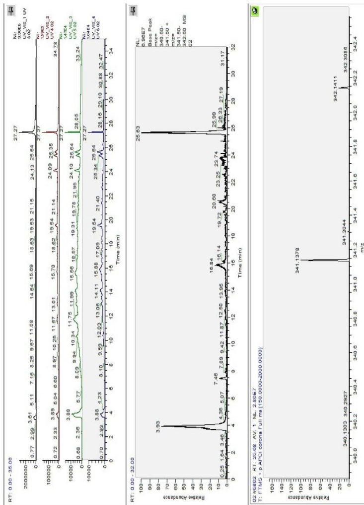
Suppl. Fig. 1. BPC extraction of Sea anemone chloroform extract for Lupinacidin A (1) (MW: 340).
