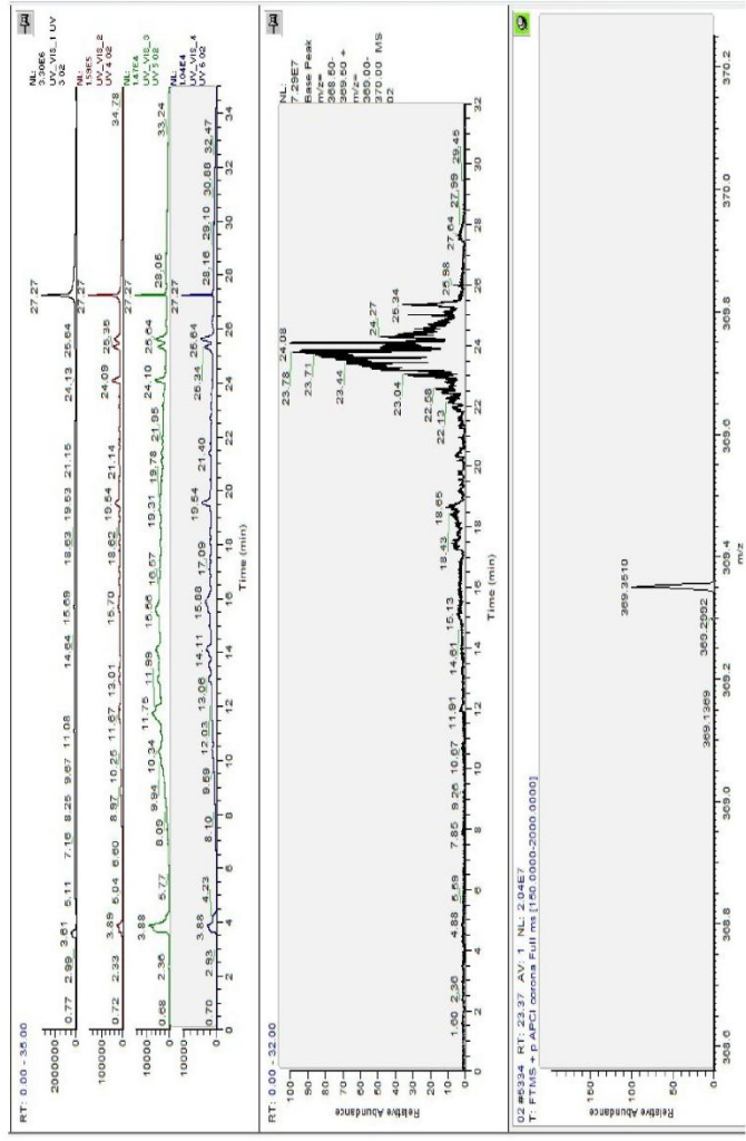
Suppl. Fig. 2. BPC extraction of Sea anemone- Chloroform extract for Galvaquinone B (2) (MW: 368).
