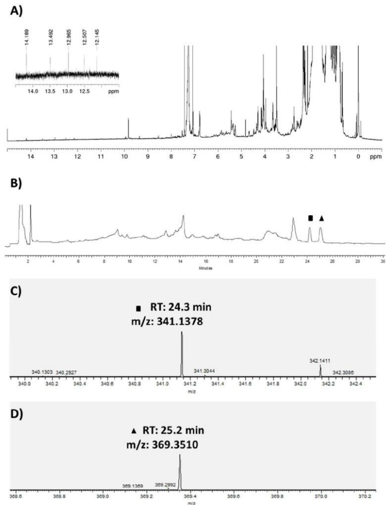
Figure 2. Chemical analysis of the crude extract of the sea anemone Gyraetis sesere . (A) ^1\text{H} NMR spectra of the crude extract of marine anemone Gyraetis sesere acquired in \text{CDCl}_3 , 600 MHz. Highlighted in the zoomed area are the frequencies of characteristic resonances originating from hydroxyl exchangeable protons in vicinity to ketogroups. (B) UV chromatogram (254 nm) of the crude extract of the sea anemone Gyraetis sesere highlighting the specific peaks for ■ RT: 24.3 min, and ▲: RT: 25.2 min. (C) High resolution mass for ■ ( m/z [\text{M} + \text{H}]^+ 341.1378) and (D) high resolution mass for ▲ (2) ( m/z [\text{M} + \text{H}]^+ 369.3510). *RT: Retention Time.
