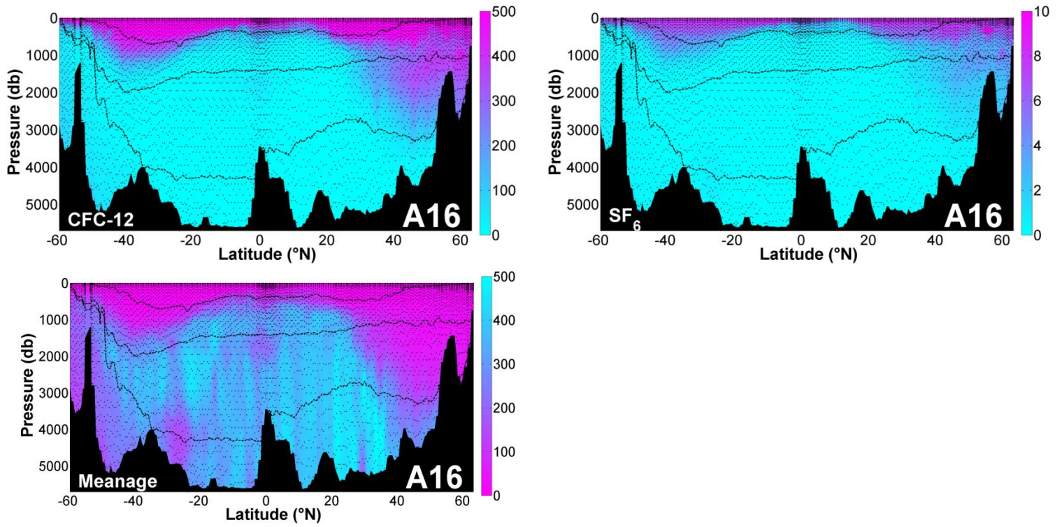
Fig 4.0 Partial pressure of CFC-12 and SF 6 (ppt) and Mean age (year) based on A16 cruise in 2013. Mean age is calculated from CFC-12 in 'old' water samples (partial pressure of CFC-12 < 450 ppt) and from SF 6 in 'young' water samples (partial pressure of CFC-12 > 450 ppt). The dashed lines show four vertical layers of water columns and the black dots show sampling points.
