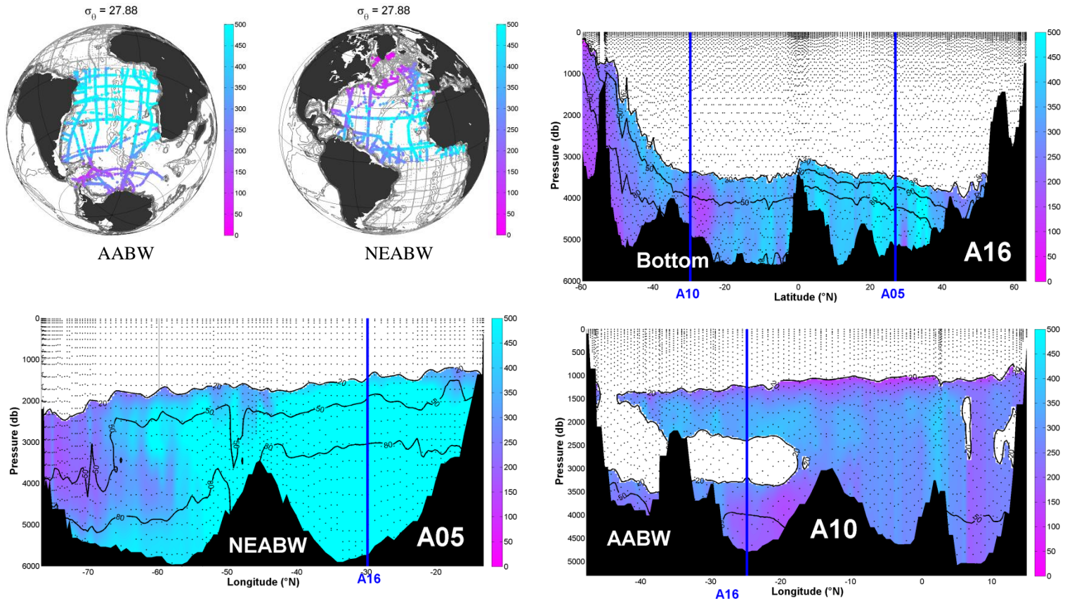
Fig 4.4 Mean ages of Bottom Water (AABW and NEABW)
