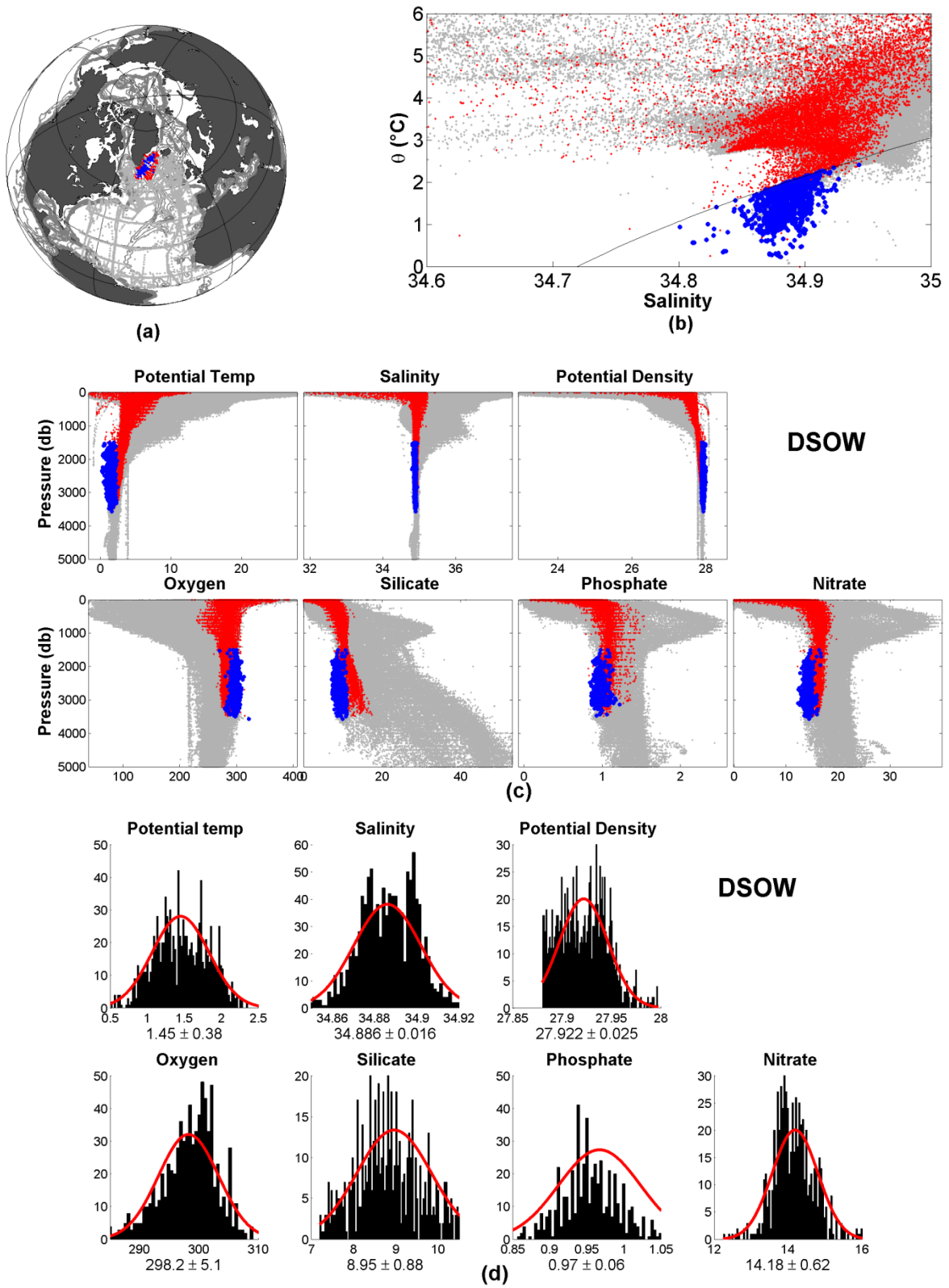
Figure 13: Overview of Denmark Strait Overflow Water (DSOW):
