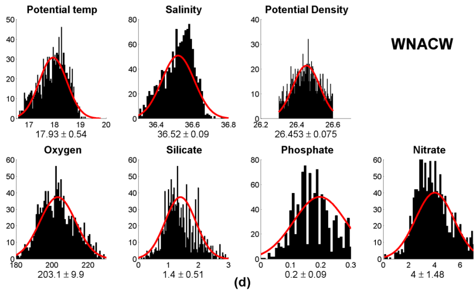
Figure 4: Overview of Western North Atlantic Central Water (WNACW): Panel a) shows the formation area used to define the water mass, panel b) show a T-S diagram and panel c) the distribution of key properties vs. pressure. In panel d) we show bar plots of the data distribution of samples used to define the water mass. Potential Temperature in ( ^{\circ}\text{C} ), Potential Density in \text{kg}/\text{m}^3 , Oxygen and nutrients in \mu\text{mol}/\text{kg}^3 . The red Gaussian fit shows mean and \sigma based on selected data.
