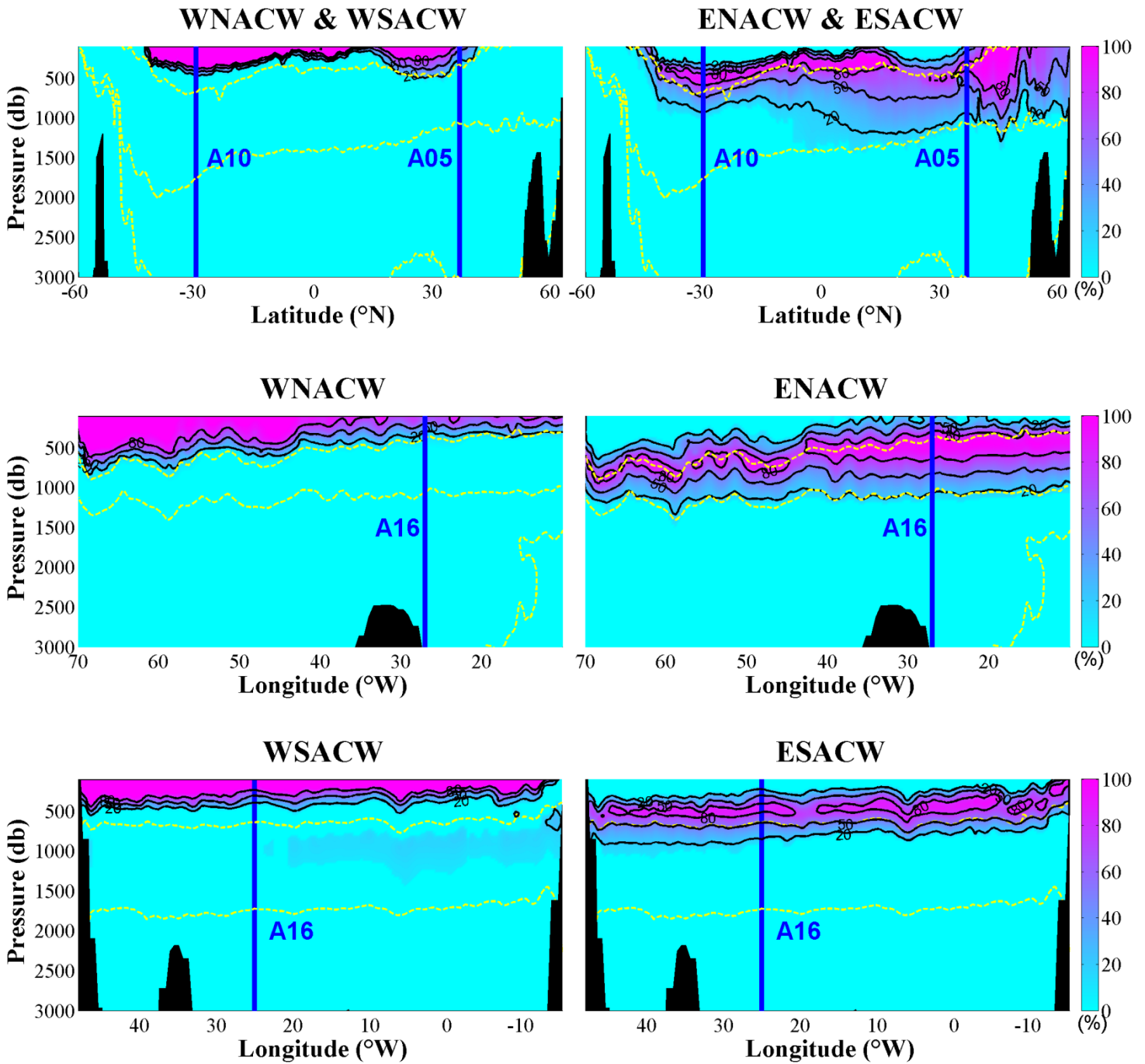
Fig. 4 Distribution of Central Water Masses based on A16 (upper), A05 (middle), A10 (lower) cruises within 3000m. Contour lines show fractions of 20% 50% and 80%, blue lines show cross section of other cruises, yellow dashed lines show the boundaries of vertical water columns layers (potential density at 27, 27.7 and 27.88 kg/m 3 )
