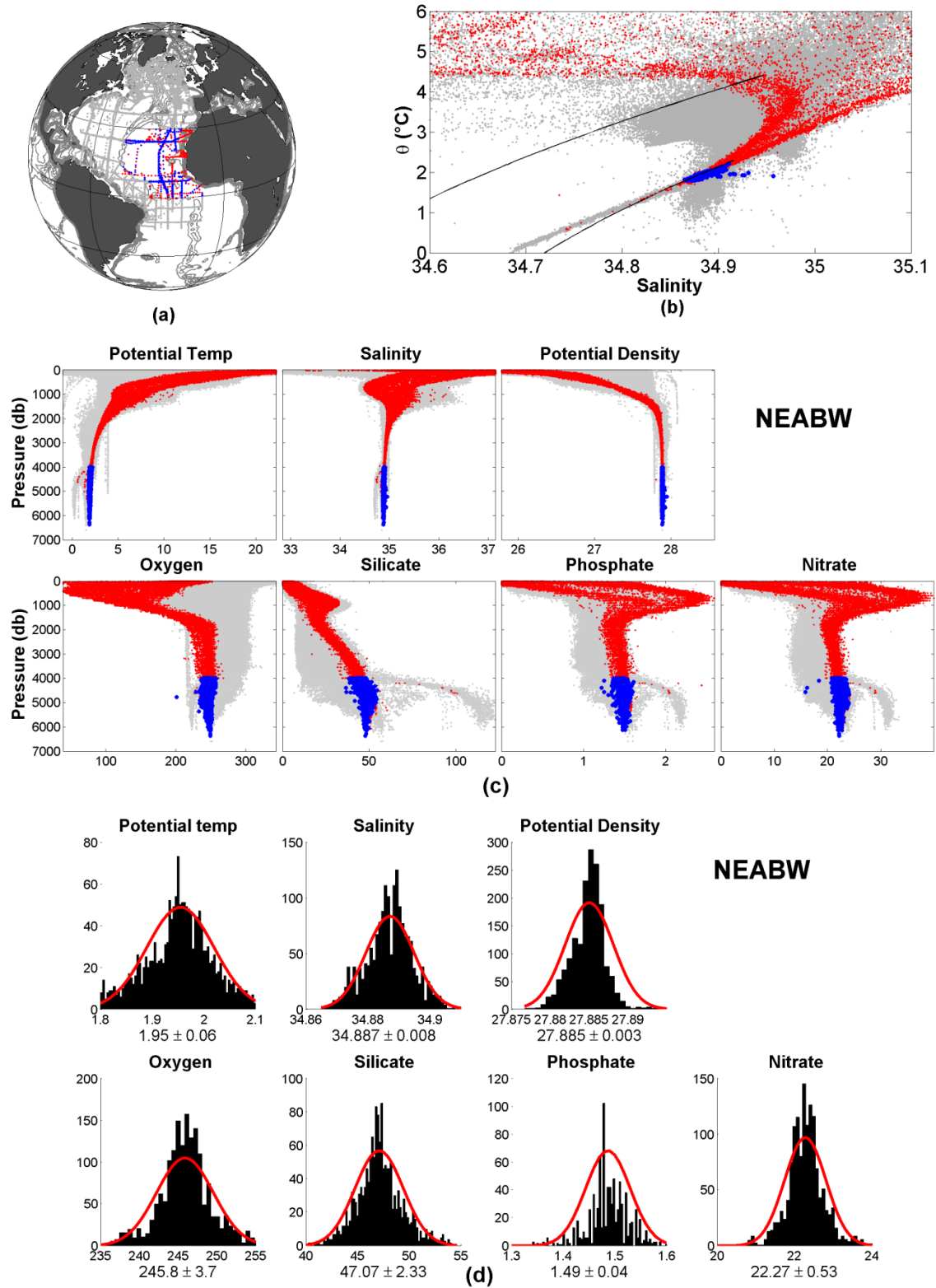
Figure 19: Overview of Northeast Atlantic Bottom Water (NEABW): Panel a) shows the formation area used to define the water mass, panel b) show a T-S diagram and panel c) the distribution of key properties vs. pressure. In panel d) we show bar plots of the data distribution of samples used to define the water mass. Potential Temperature in ( ^{\circ}\text{C} ), Potential Density in \text{kg}/\text{m}^3 , Oxygen and nutrients in \mu\text{mol}/\text{kg}^3 . The red Gaussian fit shows mean and \sigma based on selected data.
