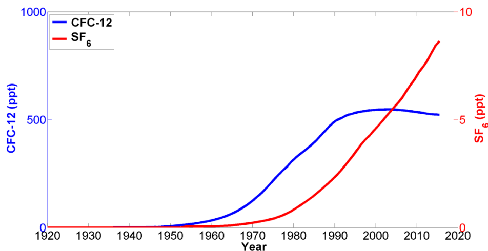
Fig 1.4 Atmospheric history of CFC-12 (blue) and SF 6 (red) in ppt
