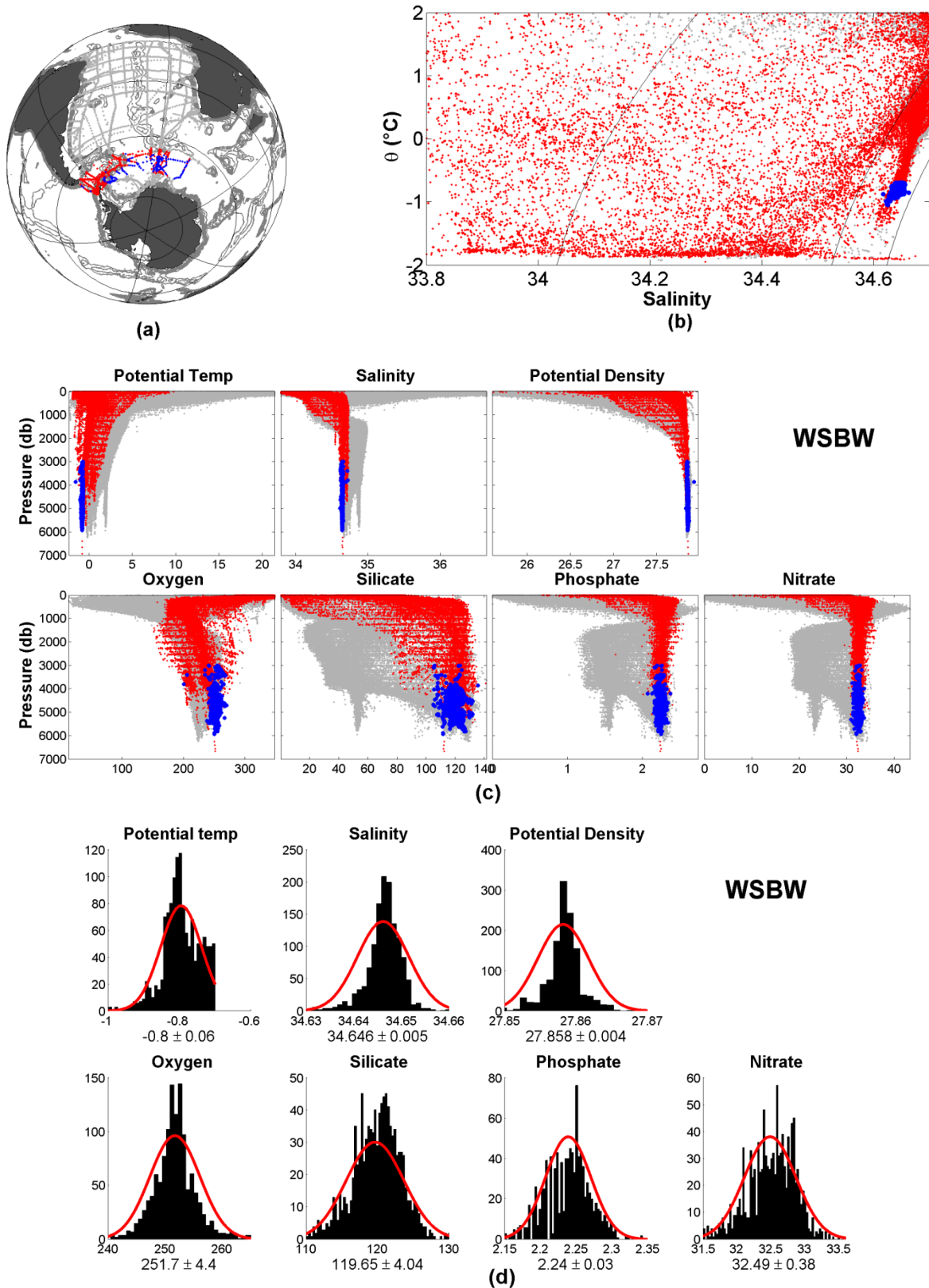
Figure 21: Overview of Weddell Sea Bottom Water (WSBW): Panel a) shows the formation area used to define the water mass, panel b) show a T-S diagram and panel c) the distribution of key properties vs. pressure. In panel d) we show bar plots of the data distribution of samples used to define the water mass. Potential Temperature in ( ^{\circ}\text{C} ), Potential Density in \text{kg}/\text{m}^3 , Oxygen and nutrients in \mu\text{mol}/\text{kg}^3 . The red Gaussian fit shows mean and \sigma based on selected data.
