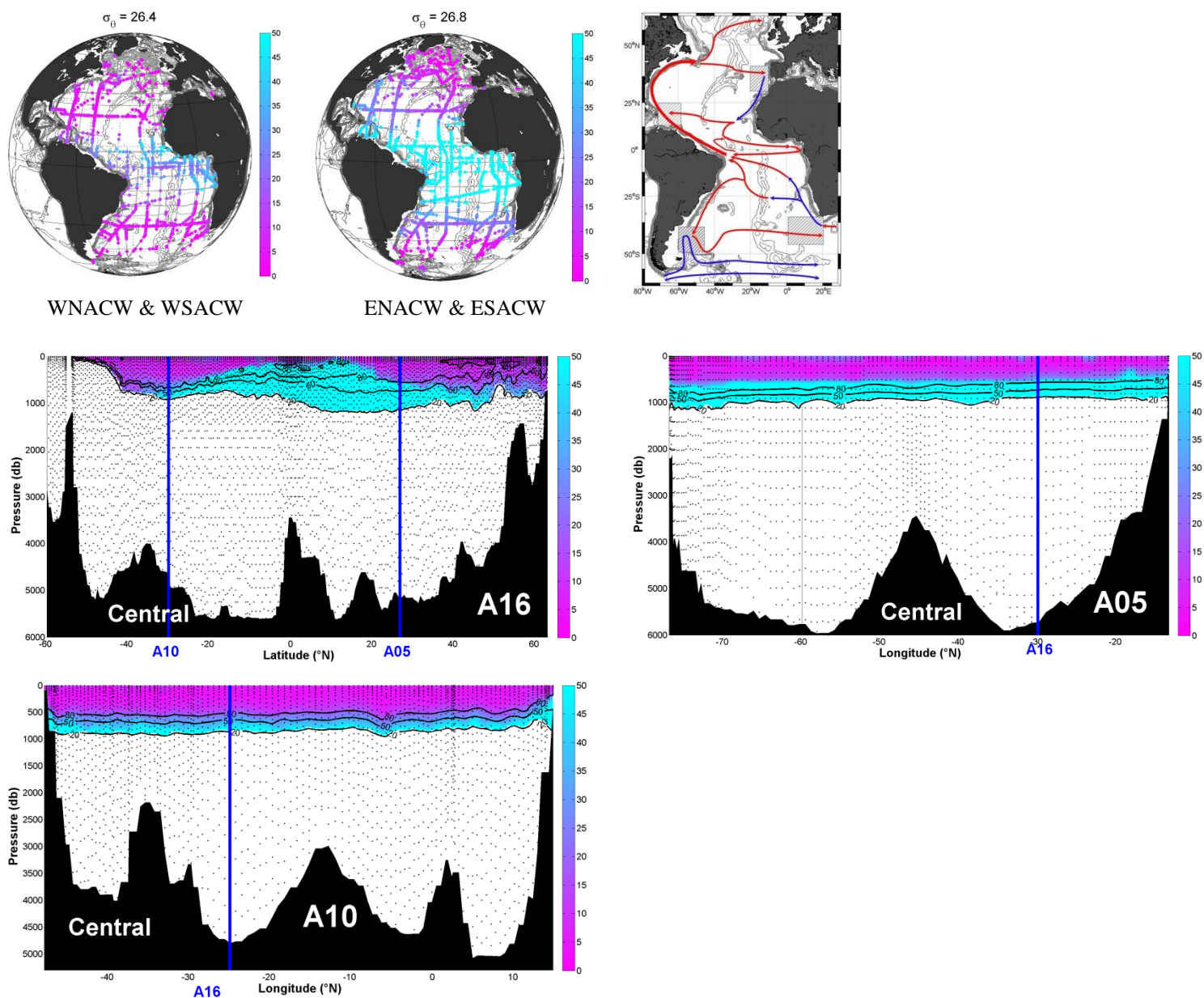
Fig 4.1 Mean ages of Central Water
