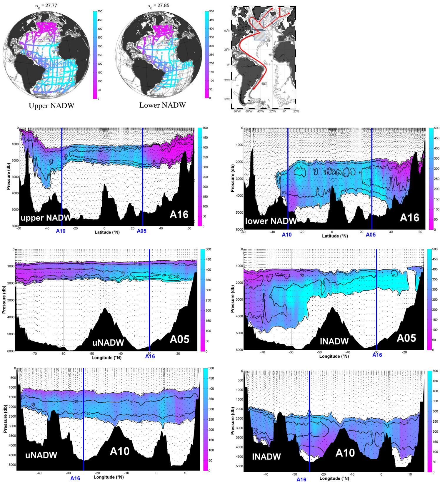
Fig 4.3 Mean ages of water masses in the deep and overflow layer (upper and lower NADW)
