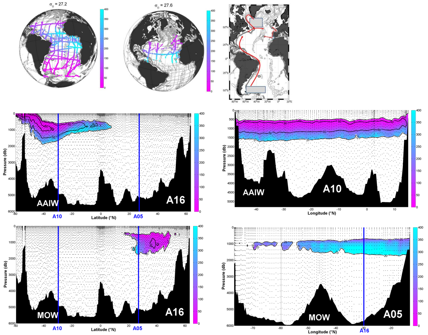
Fig 4.2 Mean ages of Water masses in the intermediate layer (AAIW and MOW)
