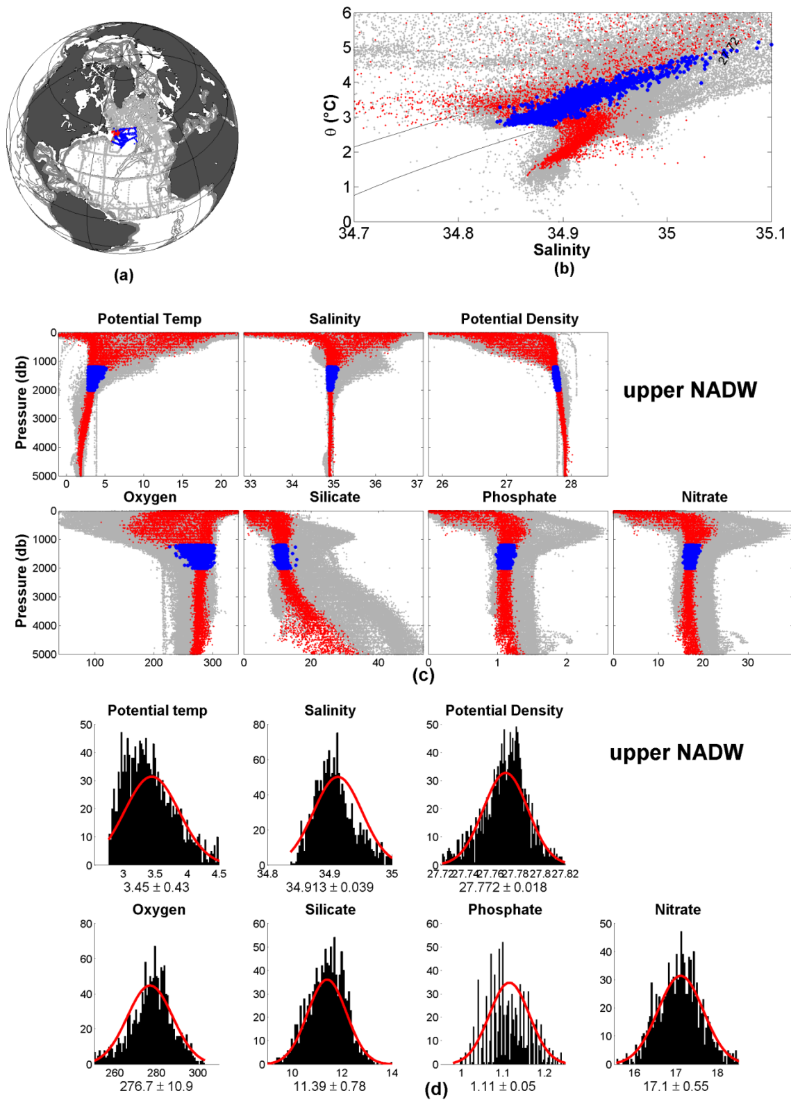
Figure 15: Overview of upper North Atlantic Deep Water (uNADW): Panel a) shows the formation area used to define the water mass, panel b) show a T-S diagram and panel c) the distribution of key properties vs. pressure. In panel d) we show bar plots of the data distribution of samples used to define the water mass. Potential Temperature in ( ^{\circ}\text{C} ), Potential Density in \text{kg}/\text{m}^3 , Oxygen and nutrients in \mu\text{mol}/\text{kg}^3 . The red Gaussian fit shows mean and \sigma based on selected data.
