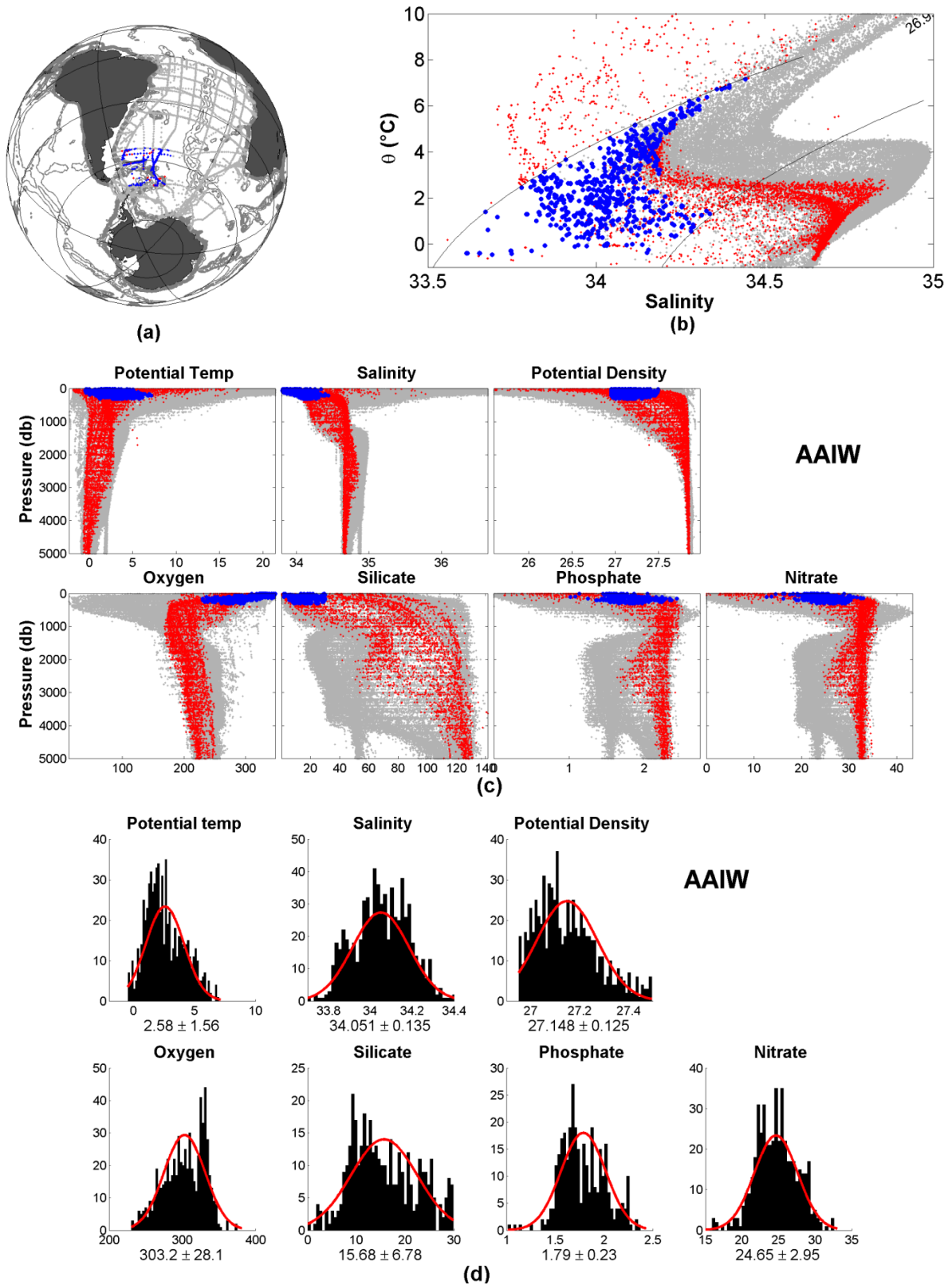
Figure 8: Overview of Antarctic Intermediate Water (AAIW): Panel a) shows the formation area used to define the water mass, panel b) show a T-S diagram and panel c) the distribution of key properties vs. pressure. In panel d) we show bar plots of the data distribution of samples used to define the water mass. Potential Temperature in ( ^{\circ}\text{C} ), Potential Density in \text{kg}/\text{m}^3 , Oxygen and nutrients in \mu\text{mol}/\text{kg}^3 . The red Gaussian fit shows mean and \sigma based on selected data.
