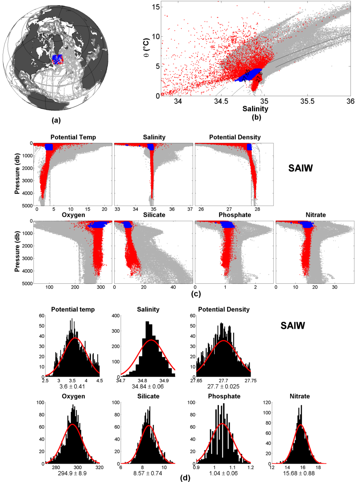
Figure 9: Overview of Subarctic Intermediate Water (SAIW): Panel a) shows the formation area used to define the water mass, panel b) show a T-S diagram and panel c) the distribution of key properties vs. pressure. In panel d) we show bar plots of the data distribution of samples used to define the water mass. Potential Temperature in ( ^{\circ}\text{C} ), Potential Density in \text{kg}/\text{m}^3 , Oxygen and nutrients in \mu\text{mol}/\text{kg}^3 . The red Gaussian fit shows mean and \sigma based on selected data.
