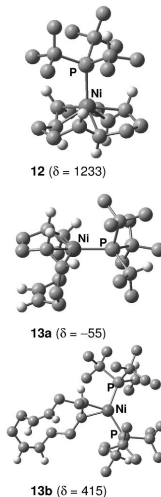
Fig. 2 Optimised \text{Ni}(\text{cdt})\text{-P}(t\text{Bu})_2(i\text{Pr}) adducts (methyl and methylene H atoms omitted for clarity), together with GIAO-B3LYP computed ^{61}\text{Ni} chemical shifts.
