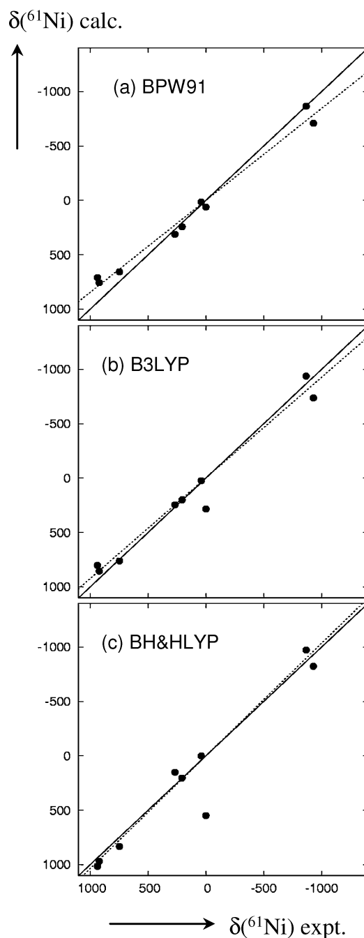
Fig. 1 Plot of GIAO-DFT computed vs. experimental ^{61}\text{Ni} chemical shifts, including linear regression lines (dashed, excluding the data point for 4 at \delta_{\text{expt}} = 0 ) and the ideal line with the slope 1 (solid).
